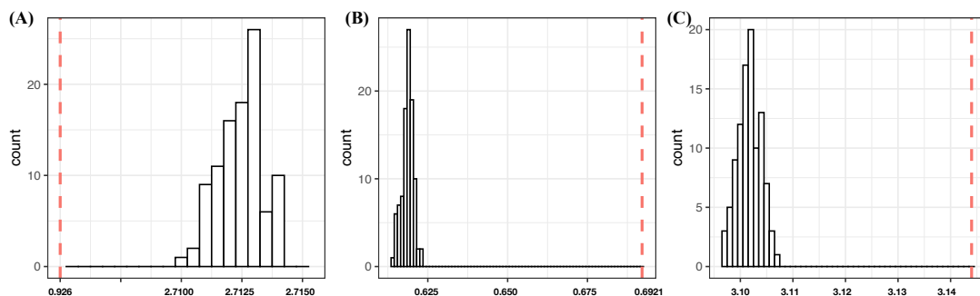
Figure 3. Testing for [C1: confirmable] on \mathcal{Y} = (pfx_X, pfx_Z) : (A) (aX, aZ) (red-marked) against histogram of (aX, \xi) ; (B) (aX, aZ, pitN) and (aX, aZ, vY0) (red-marked) against histogram of (aX, aZ, \xi) ; (C) (vZ0, z0, aY) (red-marked) against histogram of (vZ0, z0, \xi) .
