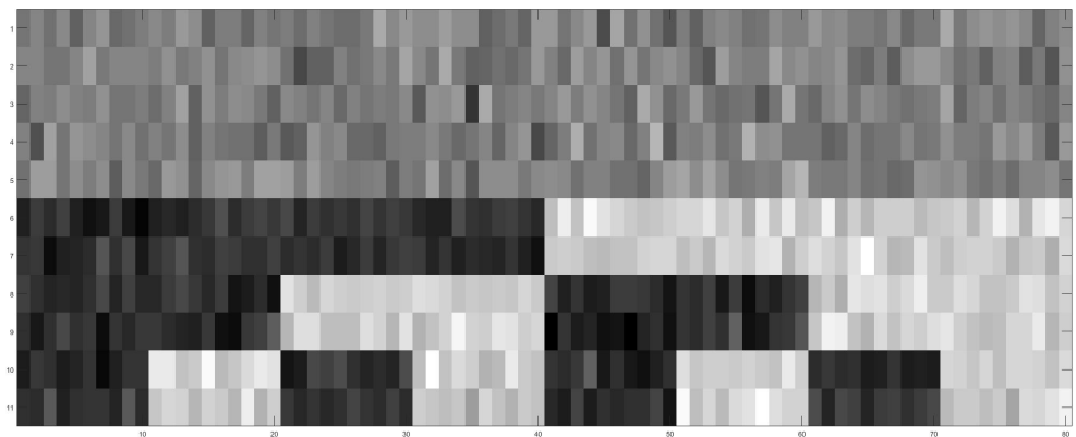
Figure 1. Clustering on 80 IDs’ vectors of means of 11 features.
