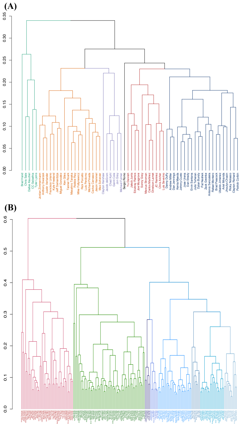
Figure 6. Hierarchical clustering trees marked with pitcher groups: (A) 62 slider pitchers; (B) 199 fastball pitchers with 3 colored major branches A, B, and C (from left to right). The C-branch is further partitioned into six colored sub-branches: C1 to C6 (left to right).
