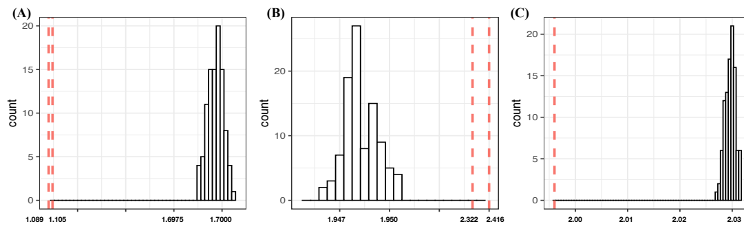
Figure 5. Testing for [C1: confirmable] on \mathcal{Y} = (pfx_X, pfx_Z) : (A) (aX, aZ, vY0) and (aX, aZ, startSp) red-marked against histogram of (aX, aZ, \epsilon) ; (B) (aY, pitN, spinR) and (aY, pitN, startSp) red-marked against histogram of (aY, pitN, \epsilon) ; on \mathcal{Y} = (ax, az) : (C) (spinD, pitN, aY) red-marked against histogram of (spinD, pitN, \epsilon) .
