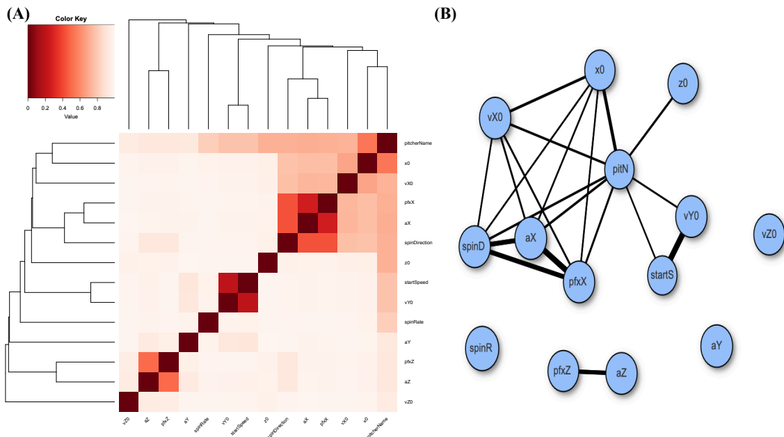
Figure 4. Associative patterns of fastballs among 14 features: (A) heatmap based on MCE-matrix; (B) network built with linkages with thickness proportional to one minus pairwise MCE and subject to a threshold 0.2 (= 1.0 – MCE).
