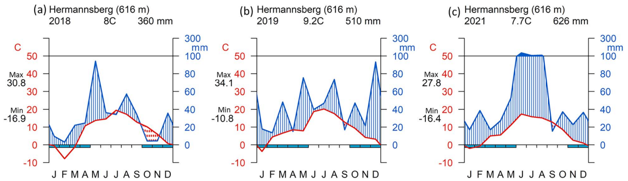
Figure 2. Walter Lieth climate diagram of the study site Hermansberg (Germany) in (a) 2018, (b) 2019 and (c) 2021. Average annual temperature (°C) and annual precipitation (mm) are shown. Max: mean of the maximum temperatures of the warmest month. Min: mean of the minimum temperatures of the coldest month.
