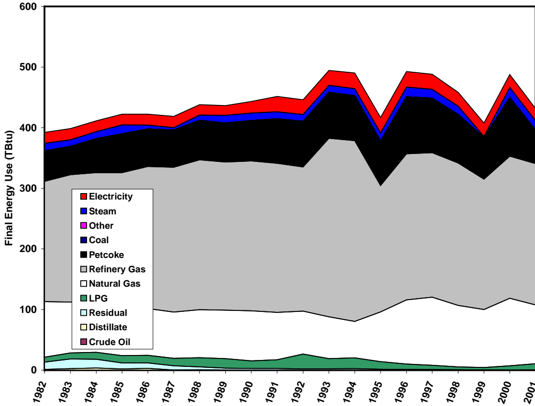
Figure 18. Reported final energy consumption data for petroleum refineries in California. Electricity data is purchased electricity only. Sources: California Energy Commission, utility sales.
