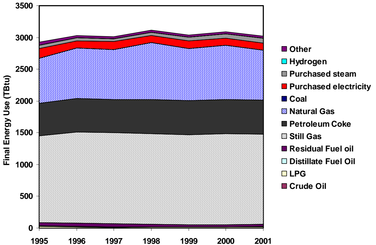
Figure 15. Annual final energy consumption of U.S. petroleum refineries for the period 1995 – 2001. Data for 1995 and 1997 contains estimated values for natural gas, coal, electricity and steam purchases. Source: Petroleum Supply Annual, Energy Information Administration.
