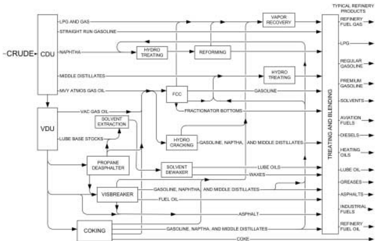
Figure 11. Simplified flowchart of refining processes and product flows. Derived from Gary and Handwerk (1994).
