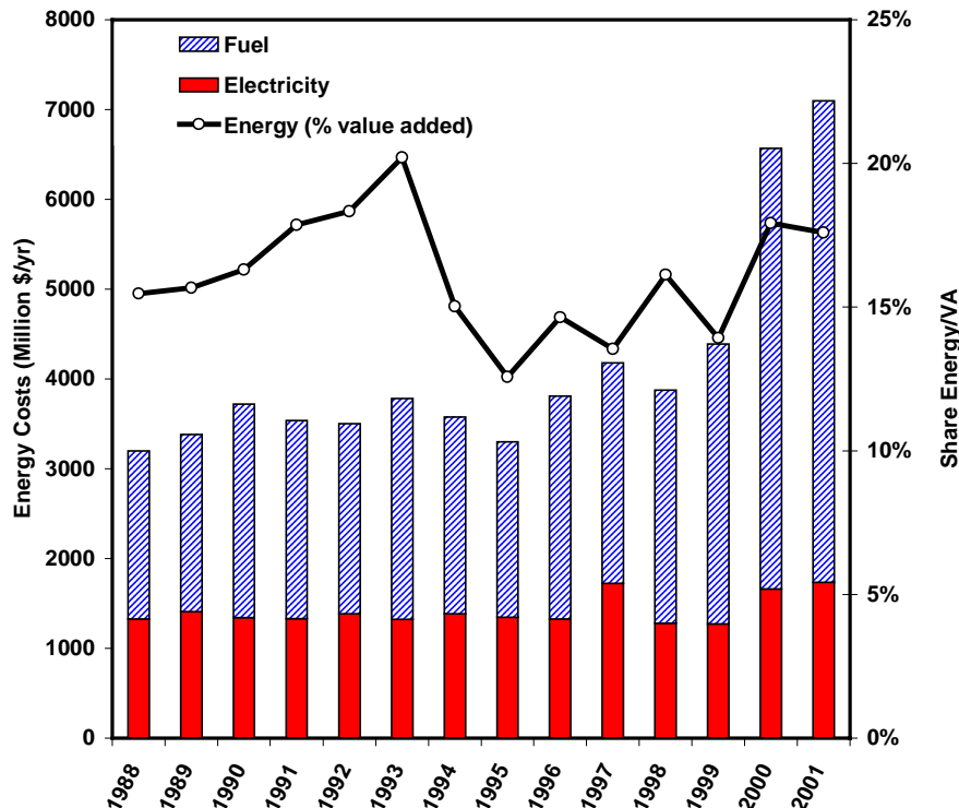
Figure 14. Annual energy costs of petroleum refineries in the United States 1988-2001. Costs are given for purchased fuels and purchased electricity. The total energy costs are given as share of the value added produced by petroleum refineries. Source: U.S. Census, Annual Survey of Manufacturers.
