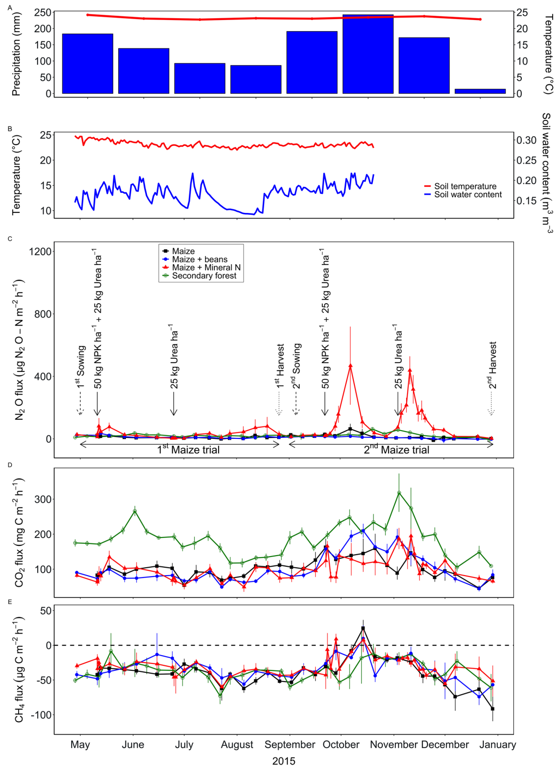
Fig. 3 | Land use effects on soil-atmosphere exchange of greenhouse gases.
