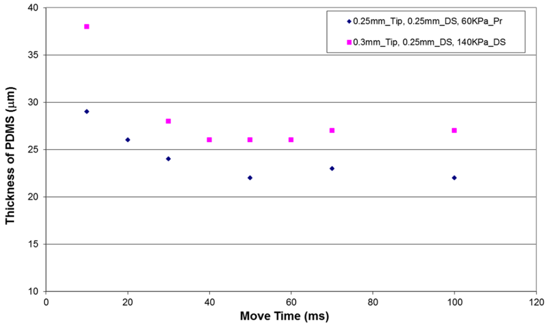
Figure 140. The thickness of PDMS ('D' in Figure 138b) as a function of varying move times in the pneumatic printer.
