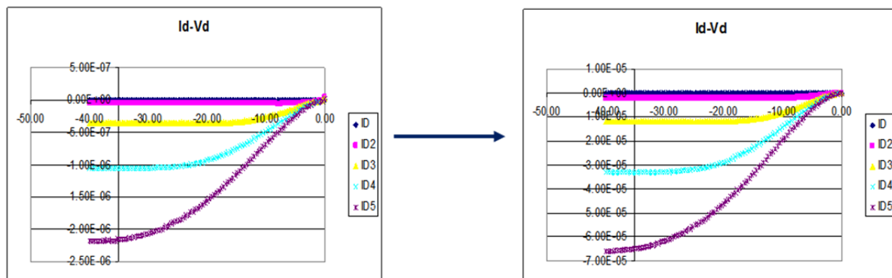
Figure 20. I_{\text{d}} - V_{\text{d}} characteristics from 2 different experiments with the lowest (left) and highest (right) performing samples.
