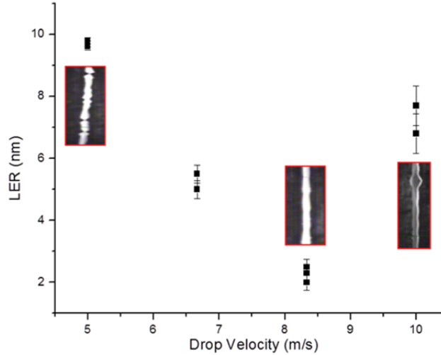
Figure 41. LER Measurements of gold inkjet printed lines performed to obtain optimum drop velocity.
