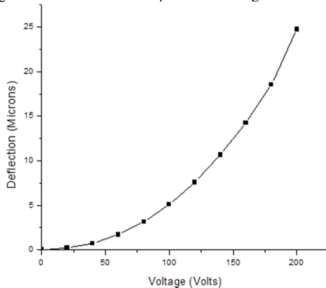
Figure 125. Deflection as a function of voltage for the 2-D simulation in Figure 124.
