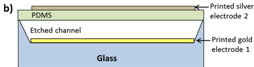
Figure 151. a) Micrograph and b) cross-section of final all-printed PDMS valve structure.
