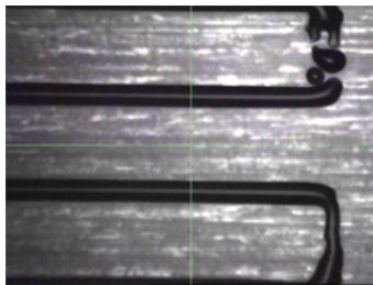
Figure 43. Inaccurate landing of drops in a pattern due to increased print height.
