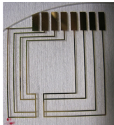
2-RTDs structure
