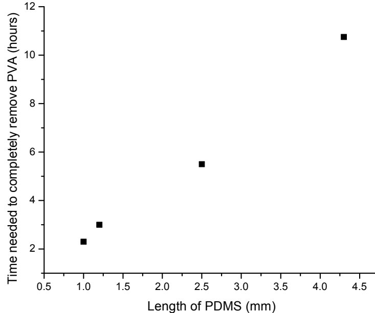
Figure 148. Immersion time required to completely remove PVA as a function of length of PDMS.
