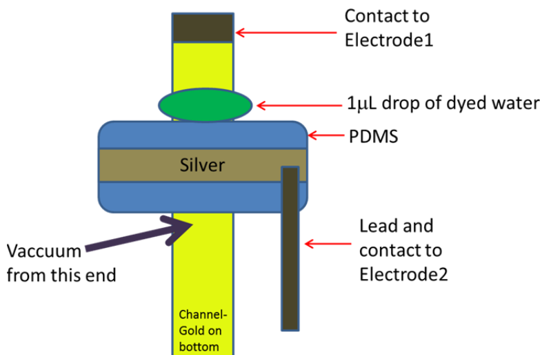
Figure 152. Schematic of setup used to measure flow rate as a function of voltage.
