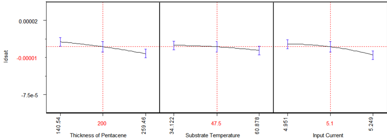
Figure 18. Relationship between the input parameters (substrate temperature ( ^{\circ}\text{C} ), input current (Amps), thickness of pentacene ( \text{\AA} )), and I_{\text{dsatsat}} or saturation current (Amps).
