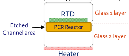
Figure 4. Cross-section of a typical RTD and heater structure used for PCR thermal cycling in LOC devices.
