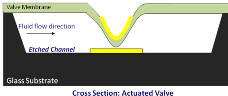
Figure 123. Basic functioning of an electrostatic microvalve; the open valve (top) is when both electrodes are grounded while the actuated valve (bottom) is triggered by a potential difference between the two electrodes.
