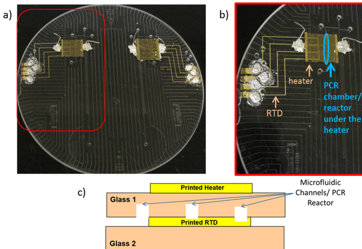
Figure 101. Final thermally bonded chip used to demonstrate PCR: a) An image of the entire chip with two microfluidic channels and reactors (left and right sides of the chip); b) A zoomed-in version of the section of chip (left side) which is used to demonstrate PCR in this project; c) Cross section of the thermally bonded chip.
