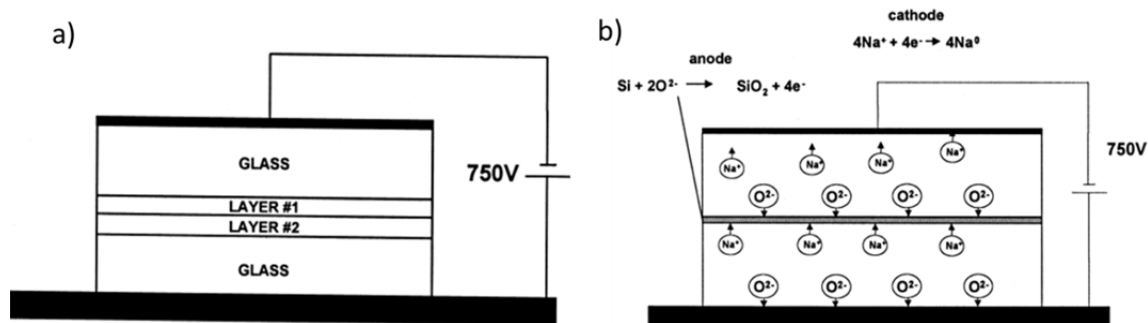
Figure 92. Anodic bonding setup and mechanism: a) schematic of the setup inside the anodic bonder, b) working mechanism of anodic bonding [9] .
