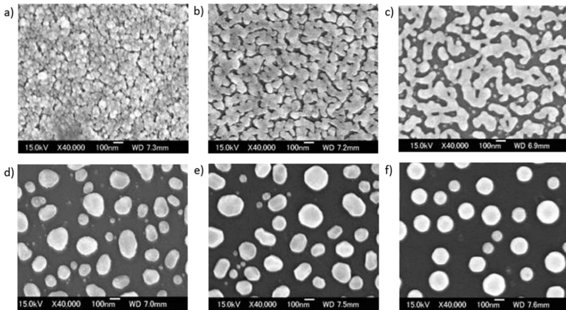
Figure 90. SEM of gold nanoparticle films as a function of increasing temperature: (a) 25 o C, (b) 150 o C, (c) 250 o C, (d) 450 o C, (e) 900 o C and (f) 1100 o C[8].
