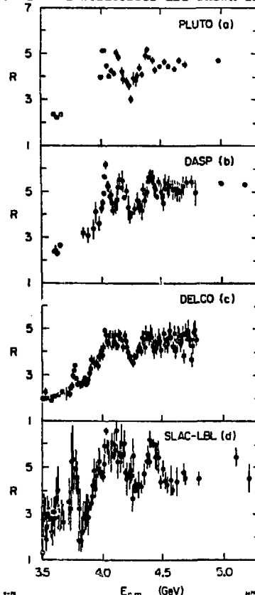
Fig. 9. Ratio R of hadronic annihilation cross section to dimuon cross section.
