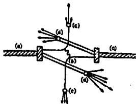
Fig. 4. Possible mechanism for high P_T particle production. (a) Incoming protons. (b) Large angle quark-quark scattering by gluon exchange. (c) Fragmentation of scattered quarks into hadrons. (d) Fragmentation of spectator quarks into hadrons.
