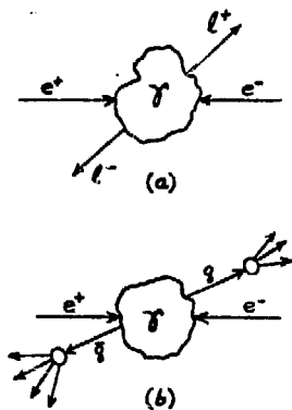
Fig. 8. Mechanism of e^+e^- annihilation to produce (a) lepton pairs, (b) quark pairs which fragment to hadrons.
