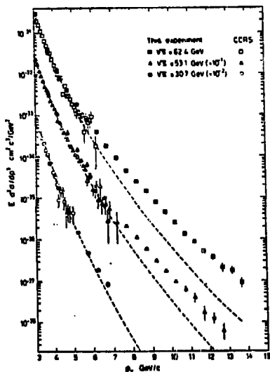
Fig. 5. Cross sections for the reaction p+p \rightarrow \pi^0 + \text{anything} versus P_T . The cross-section scale corresponds to the data at \sqrt{s} = 62 GeV. For \sqrt{s} = 53.1 and 30.6 , the data have been divided by factors of 10 and 100 respectively.
