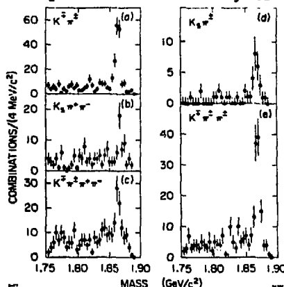
Fig. 12. D^0 and D^+ signals in various effective-mass plots.
