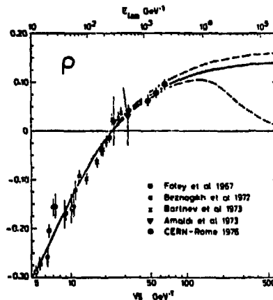
Fig. 1. Ratio of real to imaginary part of forward proton-proton scattering amplitude.
