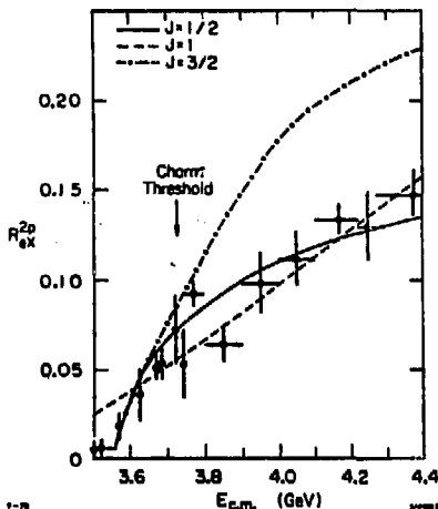
Fig. 13. Cross section for the process e^+e^- \rightarrow e^\pm + \text{anything except } e^\mp .
