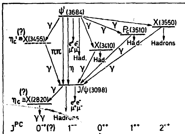
Fig. 11. Charmonium ( c\bar{c} ) level diagram as of October 1977.
