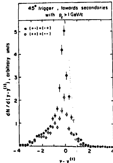
Fig. 6. Rapidity distribution of same-side secondaries ( P_T > 1 GeV/c) relative to the trigger rapidity.
