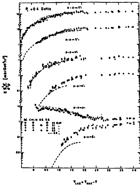
Fig. 2. Cross sections for pion, kaon and proton production versus laboratory rapidity.
