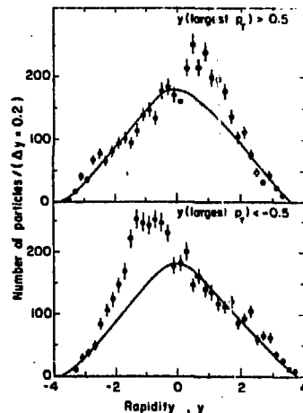
Fig. 7. Rapidity distributions of opposite-side secondaries with P_T > 0.8 GeV/c from events in which the opposite-side particle with highest P_T (the "pseudo trigger" which is not included in the figure) has P_T > 1.0 GeV/c: (a) The pseudo trigger has rapidity y > 0.5 (b) The pseudo trigger has rapidity y < -0.5 .
