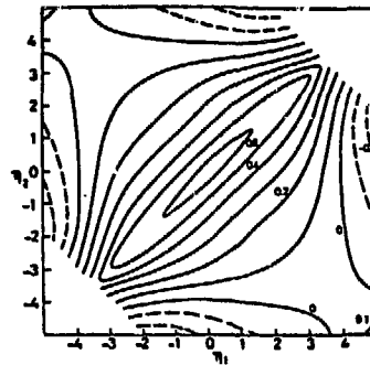
Fig. 3. Contours of constant two-particle correlation in the \eta_1 - \eta_2 plane at a total energy \sqrt{s} = 62 GeV. Here \eta is almost the same quantity as the rapidity y defined in the text.
