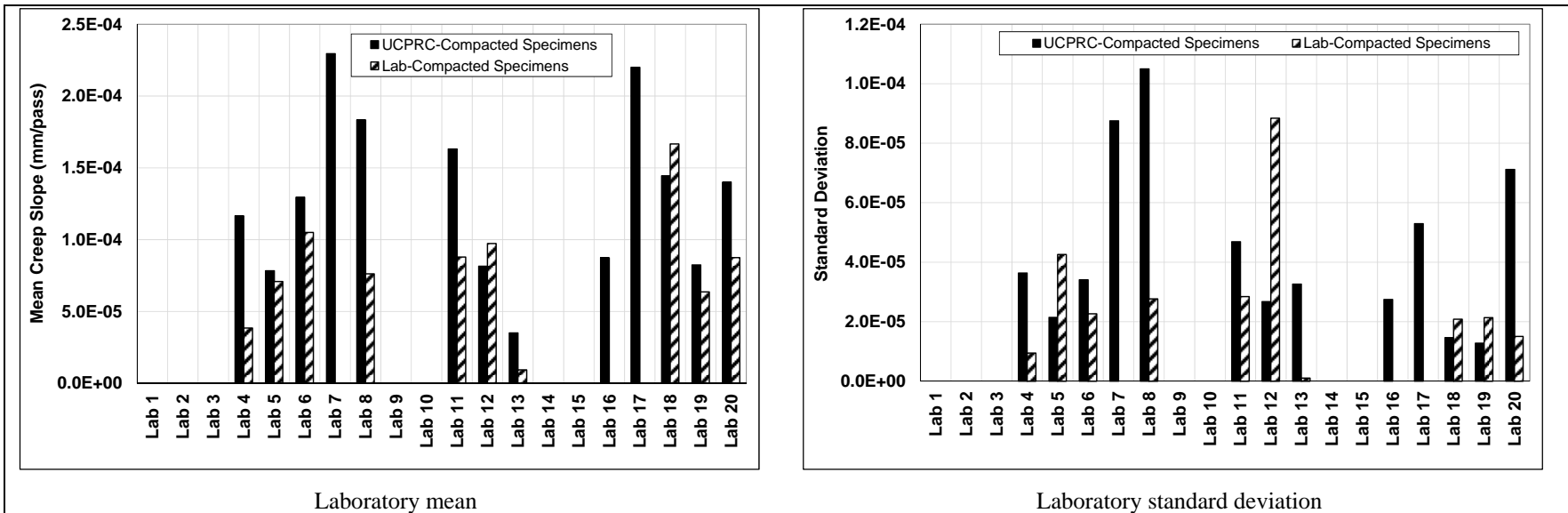
Figure 4.6: Creep slope.
