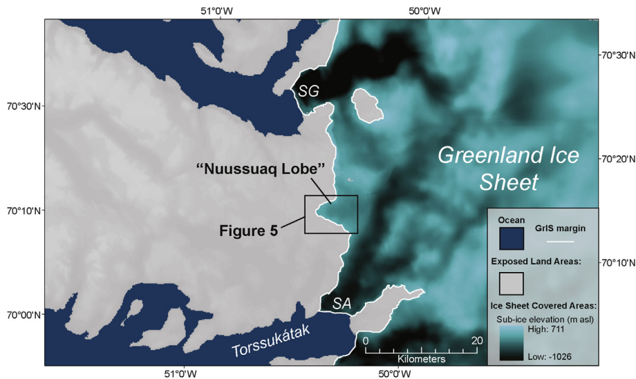
Fig. 8. Sub-ice topography data (Morlighem et al., 2014) showing low-topography areas associated with marine-terminating, high-velocity outlet glaciers (Rignot and Mouginot, 2012) to the north and south of the Nuussuaq Lobe. Sermeq Avannarleq (SA) is the marine-terminating outlet glacier to the south and appears to be more topographically connected to the Nuussuaq Lobe than Store Gletscher (SG) to the north. Radiocarbon constraints from the NPR-4 sediment core constrain minimum ice sheet extent to a period that coincides with local peak oceanic thermal conditions (Perner et al., 2013) suggesting that the Nuussuaq Lobe may be affected by the behavior of the adjacent marine terminating glaciers.
