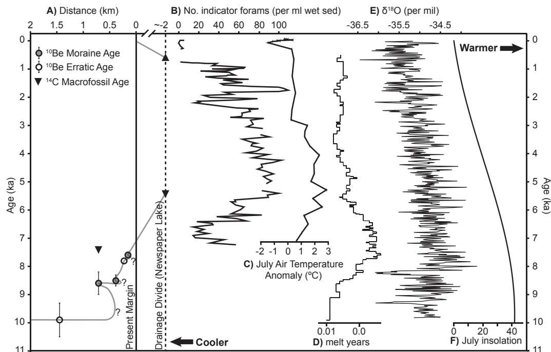
Fig. 7. A) Mean ^{10}\text{Be} \pm 1\sigma and ^{14}\text{C} ages \pm 2\sigma plotted vs. distance from the present ice margin. White circles are erratic ^{10}\text{Be} ages, gray circles are moraine boulder ^{10}\text{Be} ages and black triangles are ^{14}\text{C} ages from macrofossils in lake sediments (some small error bars are captured within symbol). The drainage divide ~2 km inland of the present ice margin (black vertical line) denoted by dotted vertical line. See Supplemental Fig. S1 for broader time-distance history. B) Number of calcareous Atlantic water foraminifera (per ml of wet sediment; Perner et al., 2013). C) Midge-based July air temperature anomaly (Axford et al., 2013). D) Melt years in GISP2 ice core (1000 year running mean, Alley and Anandakrishnan, 1995). E) NGRIP ice core \delta^{18}\text{O} (Vinther et al., 2006). F) Northern hemisphere July insolation values (Berger and Loutre, 1991).
