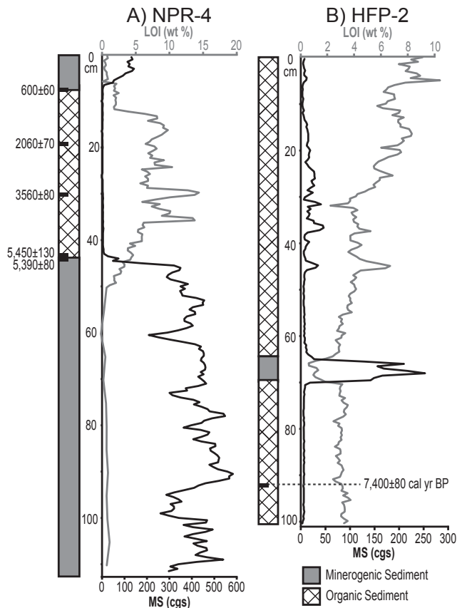
Fig. 6. Sediment core logs from Newspaper Lake and Hvide Falk Lake showing loss-on-ignition (LOI; gray line), magnetic susceptibility (MS; black line) and radiocarbon ages (cal yr BP) reported as the median of the 2\sigma range \pm one half of the 2\sigma range. Ages were calibrated using CALIB v 7.0 (Stuiver et al., 2013) and the IntCal13 calibration curve (Reimer et al., 2013). A) NPR-4 sediment core log. B) HFP-2 sediment core log.
