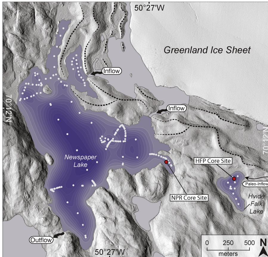
Fig. 4. Bathymetry maps for Newspaper Lake and Hvide Falk Lake superimposed on a hillshade of a digital surface model ( http://www.pgc.umn.edu/elevation/stereo/sets/m ). Bathymetric contours are 5 m each and bathymetry measurement locations are illustrated by white circles. Red circles show coring locations for NPR-4 and HFP-2. Thick black arrows indicate direction of inflows and outflows for Newspaper Lake. The thin black arrow shows a paleo-inflow channel to Hvide Falk Lake that would have been active when the ice margin extent was at the outermost Drygalski Moraine, or perhaps some distance inboard. Drygalski Moraine crests are highlighted with dashed black lines. Grey areas outlined in black are bodies of water where bathymetry data are not available. (For interpretation of the references to colour in this figure legend, the reader is referred to the web version of this article.)
