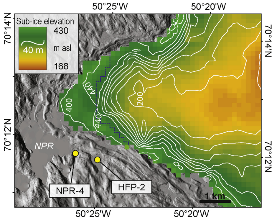
Fig. 5. Map showing sub-ice topography below the Nuussuaq Lobe (Morlighem et al., 2014) and hillshade from digital topographic data of ice-free areas ( http://www.pgc.umn.edu/elevation/stereo ). Sediment core sites denoted by yellow circles. Note Newspaper Lake (NPR) drainage divide ~2 km inboard of the present ice terminus, indicated by the blue dotted line. See text for method used for determining drainage divide location. (For interpretation of the references to colour in this figure legend, the reader is referred to the web version of this article.)
