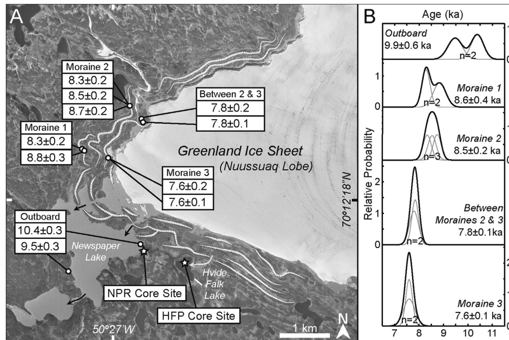
Fig. 2. A) Map with ^{10}\text{Be} ages in ka (1985 aerial photograph base; from National Danish Survey and Cadastre of Denmark). Drygalski Moraine crests delineated by dotted white lines and numbered from one to three from outer to inner. Small black arrows show flow in/out of Newspaper Lake; small white arrow is a paleo-channel into Hvide Falk Lake. Sediment core locations shown by white stars. Note non-glacial Hvide Falk Lake is dark in coloration and proglacial Newspaper Lake is light in color due to high suspended sediment load. B) Camel plots with individual (thin gray lines) and summed (thick black lines) Gaussian age distributions for ^{10}\text{Be} ages ( n = \times denotes number of samples). Mean age \pm 1\sigma is displayed in ka for each sample subset.
