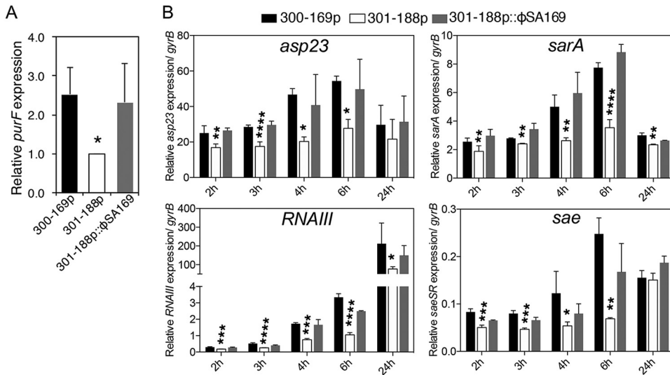
FIG 4 Relative expression levels of purF at the 3-h incubation time point (A) and asp23 (as a surrogate for sigB activation), sarA , RNAlII , and sae at 2-, 3-, 4-, 6-, and 24-h incubation time points (B) in 300-169p, 301-188p, and 301-188p:: \phi SA169 strains. *, P < 0.05 ; **, P < 0.01 ; ***, P < 0.001 ; ****, P < 0.0001 , versus 301-188p strain.
