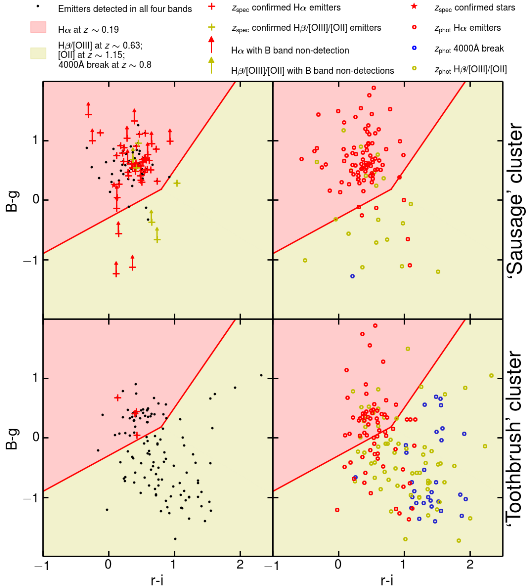
Figure 4. Colour-colour plot of ‘Sausage’ (top) plot and ‘Toothbrush’ (bottom) emitters, selected according to the criteria described in Fig. 3. B - g versus r - i colours are plotted. H \alpha emitters are expected to lie above and to the left of the thick red lines, in the red shaded areas. H \beta , [OIII], [OII] emitters and 4000Å break galaxies lie in the yellow shaded area. Left panels: Sources with clear detections are plotted with black dots. Spectroscopically confirmed H \alpha emitters are plotted in red crosses. Right panel: Sources with photometric redshifts consistent with being H \alpha emitters at z \sim 0.2 are plotted with red circles. Possible 4000Å break galaxies are plotted in blue. Sources with photo- z 's around 0.63 (between 0.5 and 0.7) and 1.15 (between 1.0 and 1.2) are selected as H \beta , [OIII] and [OII] emitters (plotted in yellow).
