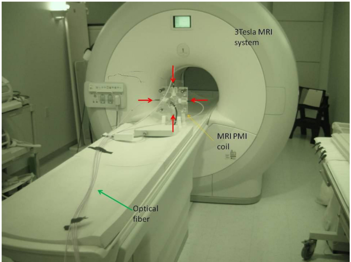
Figure 2. shows the Photo-magnetic experiment set-up. The green arrow shows the 20 meters long, 1mm diameter optical fibers which transfer the light from MRI control room into MRI scanner room. The fibers are coupled to a specially designed MRI coil, which can illuminate the laser to the medium from four sides. (red arrows) The yellow arrow is the custom designed MRI animal coil for the PMI system.
