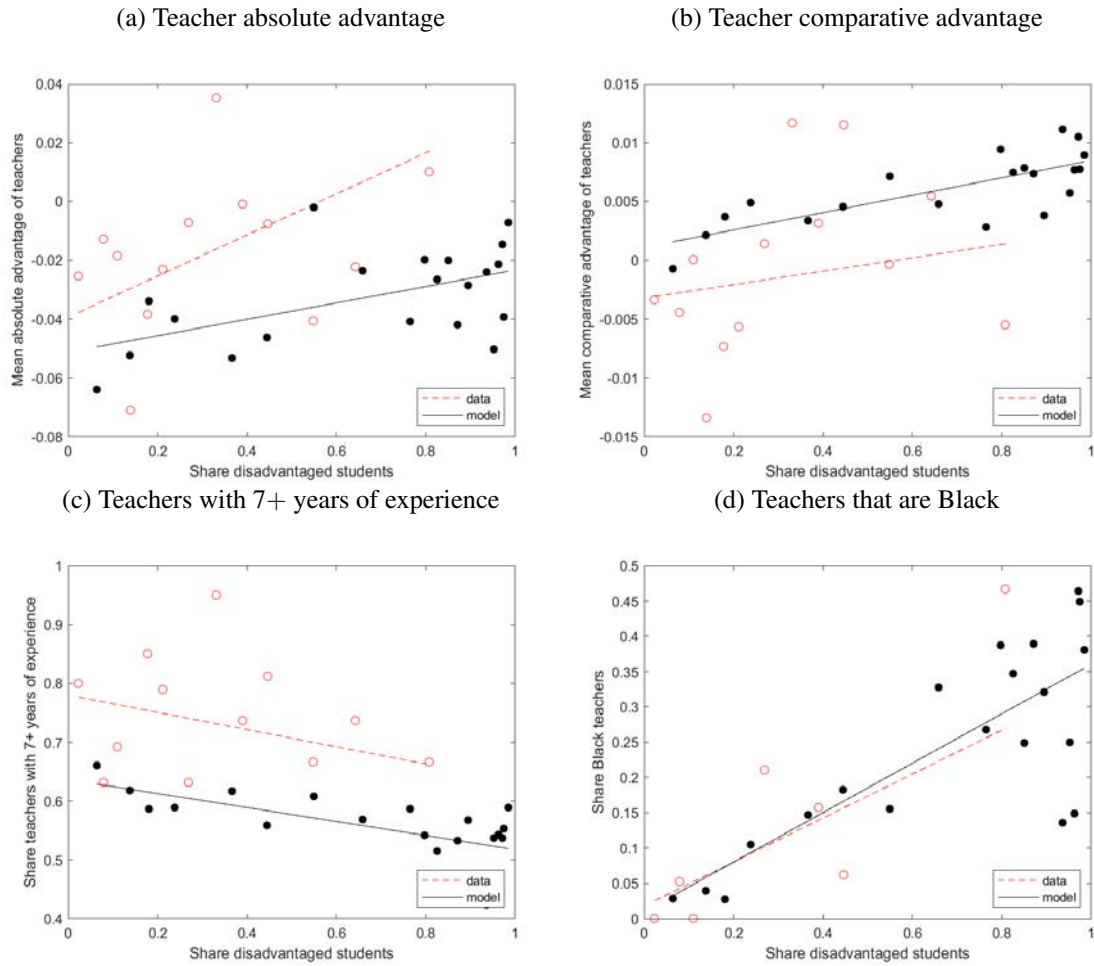
Figure 7: Model fit
