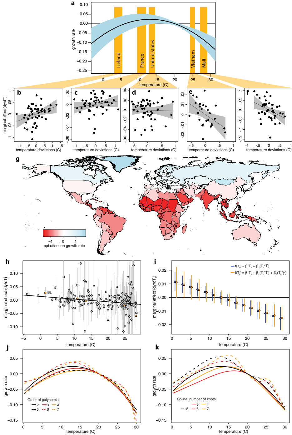
Extended Data Figure ED1: Understanding the non-linear response function. a . Response function from Figure 2a. b-f . The global non-linear response reflects changing marginal effects of temperature at different mean temperatures. Plots represent selected country-specific relationships between temperature and growth over the sample period, after accounting for the controls in Equation 15; dark line is the estimated linear relationship for each specific country, grey area the 95% CI. g . Percentage point effect of uniform 1°C warming on country-level growth rates, as estimated using the global relationship shown in a . A value of -1 indicates that a country growing at 3% yr -1 during the baseline period is projected to grow at 2% yr -1 with +1°C warming. h . Dots represent estimated marginal effects for each country from separate time series regressions (analogous to slopes of lines in Panels b-f), and grey lines the 95% CI on each. The dark black line plots the derivative \frac{\partial Y}{\partial T} of the estimated global response function in Figure 2a. i . Global nonlinearity is driven by differences in average temperature, not income. Blue dots (point estimates) and lines (95% CI) show marginal effects on growth evaluated at different average temperatures, as estimated from a model that interacts country annual temperature with country average temperature (see SI Equation 17; \frac{\partial Y}{\partial T_{it}} = \beta_1 + \beta_2 * \bar{T}_i ). Orange dots and lines show equivalent estimates from a model that also interacts annual temperature with average GDP. Point estimates are similar across the two models, indicating that the non-linear response is not simply due to hot countries being poorer on average. j-k . More flexible functional forms yield similar non-linear global response functions. j . Higher order polynomials in temperature, up to order 7. k . Restricted cubic splines with up to 7 knots. Solid black line in both plots is quadratic polynomial shown in a .
