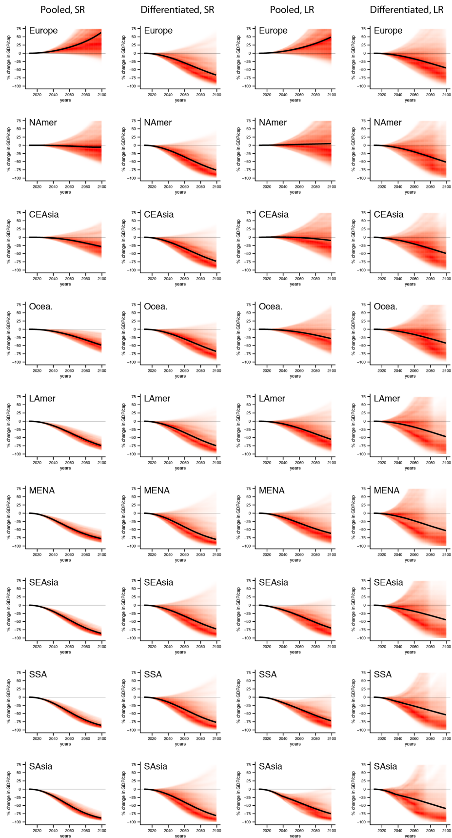
Extended Data Figure ED5: Projected impact of climate change (RCP 8.5, SSP5) on regional per capita GDP by 2100, relative to a world without climate change, under the four alternate historical response functions: pooled SR (column 1), differentiated SR (column 2), pooled LR (column 3), differentiated LR (column 4). Shading is as in Fig. 5a.
