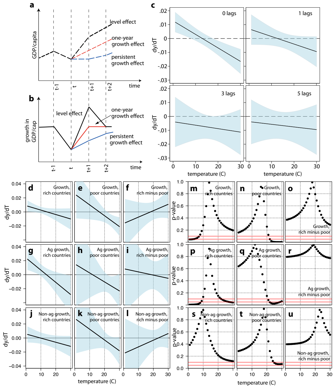
Extended Data Figure ED2: Growth versus level effects, and comparison of rich and poor responses.
