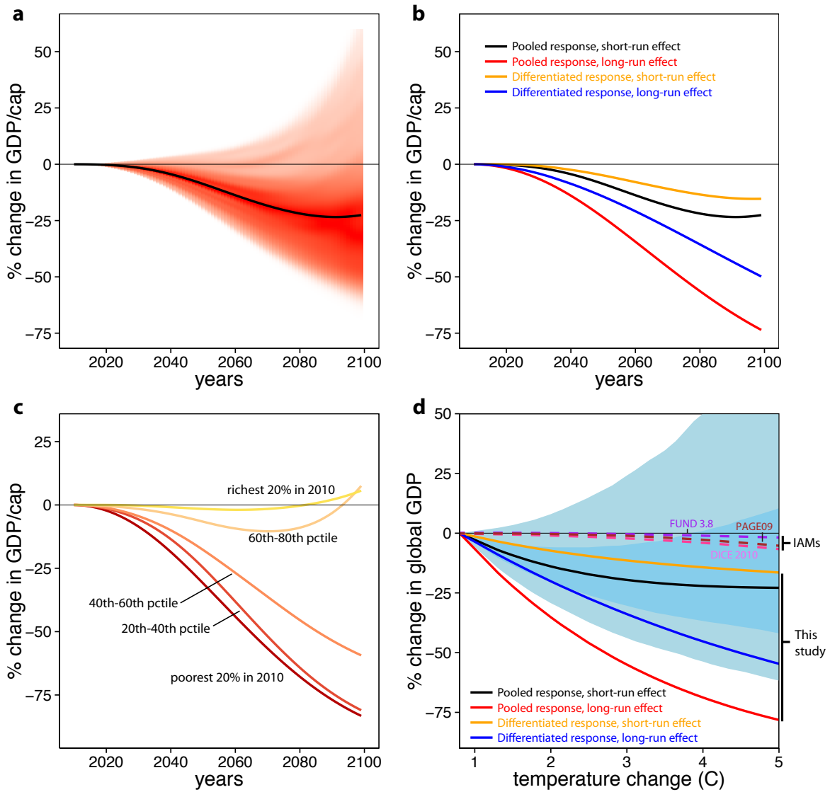
Figure 5: Global damage estimates arising from nonlinear effects of temperature. (A) Change in global GDP by 2100 using benchmark model (Figure 2a). Calculation and display same as Figure 4. (B) Same as (A) (median estimate only) comparing approaches to estimating temperature effects (pooled/differentiated: rich and poor countries assumed to respond identically/differently; Short Run/Long Run: effects account for one/five years of temperature; see SI). (C) Mean impacts by 2010 income quintile (benchmark model). (D) Projected income loss in 2100 (SSP5) for different levels of global mean temperature increase, relative to pre-industrial temperatures. Solid lines marked as in (B). Blue shaded areas are interquartile range and 5th-95th percentile estimates. Dashed lines show corresponding damages from major Integrated Assessment Models (IAMs) 12 .
