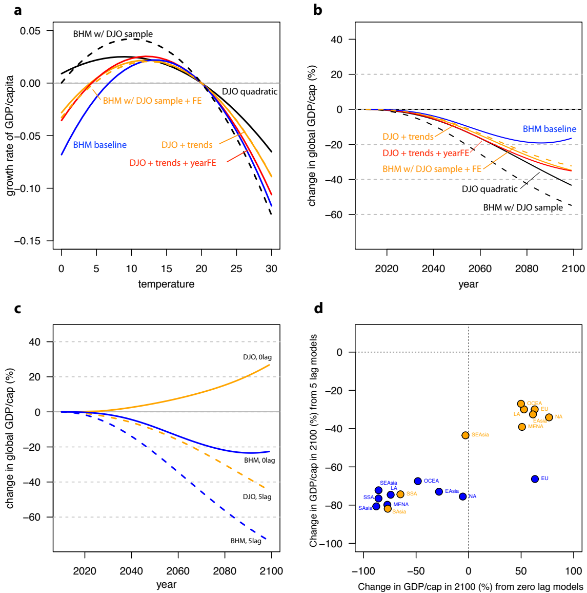
Extended Data Figure ED3: Comparison of our results (BHM) and those of Dell, Jones, and Olken (DJO). a. Allowing for non-linearity in the original DJO data/analysis indicates a similar temperature-growth relationship as obtained here under various choices about data sample and model specification (coefficients in SI Table S3). b. Projections of future global impacts on per capita GDP (RCP 8.5, SSP5) using the re-estimated non-linear DJO response functions in a. again provide similar estimates to our baseline BHM projection (shown in blue, and here using the sample of countries with >20yrs of data to match the DJO preferred sample). c. Projected global impacts differ substantially between DJO and BHM if DJO's original linear results are used to project impacts. Lines show projected change in global GDP per capita by zero- and 5-lag pooled nonlinear models in this study (blue), and zero- and 5-lag linear models in DJO (orange). d. Projected regional impacts also differ strongly between BHM's nonlinear and DJO's linear approach. Plot shows projected impacts on GDP per capita in 2100 by region, for the zero-lag model (x-axis) and 5-lag model (y-axis), with BHM estimates in blue and DJO estimates in orange. See SI for additional detail.
