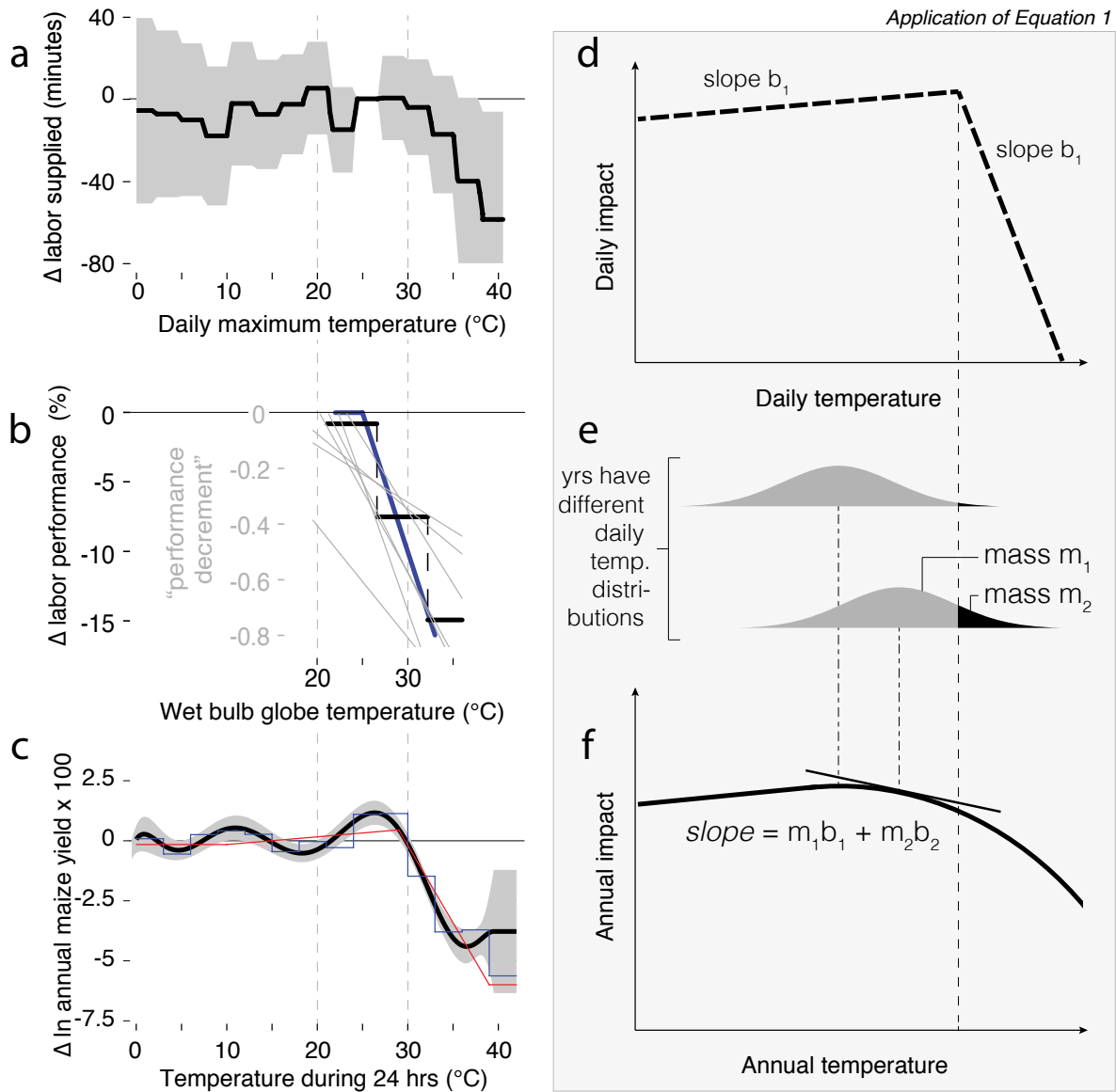
Figure 1: Highly non-linear micro responses generate smooth and shifted macro response. Highly non-linear micro-level responses of (A) labor supply 4 , (B) labor performance 6 and (C) crop yield 3 to daily temperature exposure exhibit similar “kinked” structure between 20-30°C. (D) These micro-level responses ( f_i(t) in Equation 1) map onto (E) country-level distributions of temperatures across different locations and times within that country ( g_i(T - \bar{T}) in Equation 1). Shifts in country-level distributions correspond to changes in average annual temperature, altering the fraction of location-times ( m_1 and m_2 ) exposed to different regions of the micro response in (D). (F) Aggregating daily impacts according to Equation 1 maps annual average temperature to annual output as a nonlinear and concave function that is smoother than the micro-response with a lower optimum ( Y(\bar{T}) in Equation 1).
