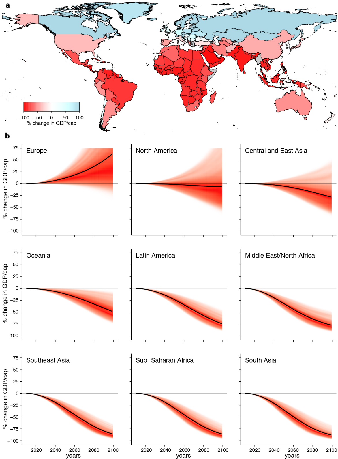
Figure 4: Projected effect of temperature changes on regional economies. Change in GDP per capita (RCP8.5, SSP5) relative to projection using constant 1980-2010 average temperatures. (A) country-level estimates in 2100. (B). Effects over time for nine regions. Black lines are projections using median estimates. Red shaded area is 95% C.I., color saturation indicates estimated likelihood an income trajectory passes through a value. 27
