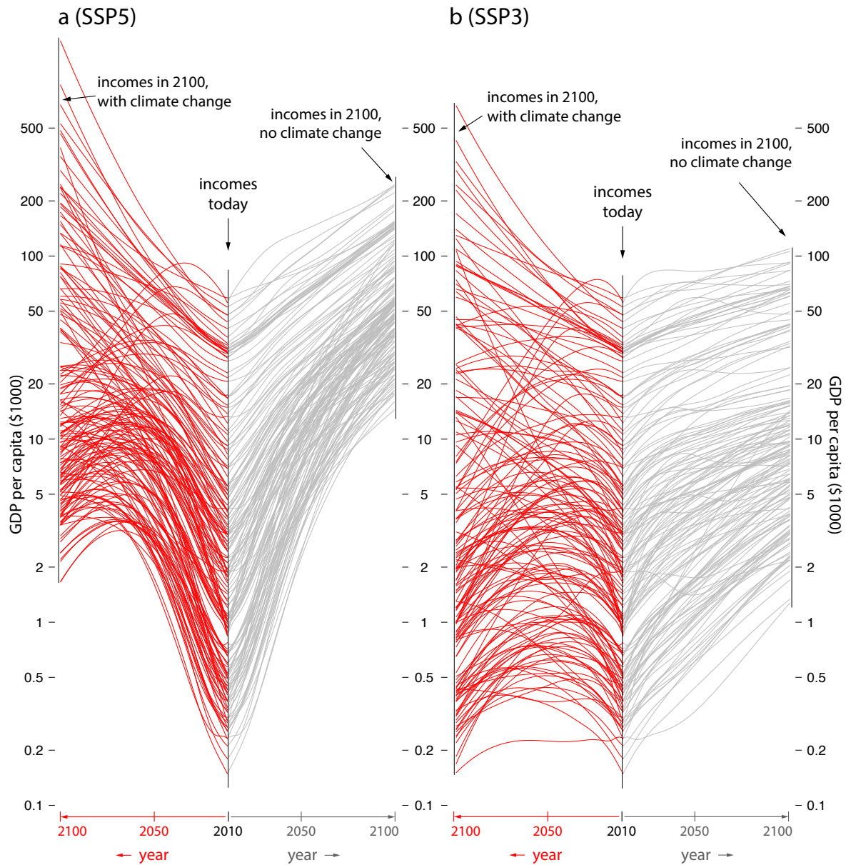
Figure 3: National income projections with and without temperature effects of climate change. Projections to 2100 for two socioeconomic scenarios consistent with RCP8.5 “business as usual” climate change: (A) SSP5 assumes high baseline growth and fast income convergence; (B) SSP3 assumes low baseline growth and slow convergence. Center in each panel is 2010, each line is a projection of national income. Right (grey) are incomes under baseline SSP assumptions, left (red) are incomes accounting for nonlinear effects of projected warming.
