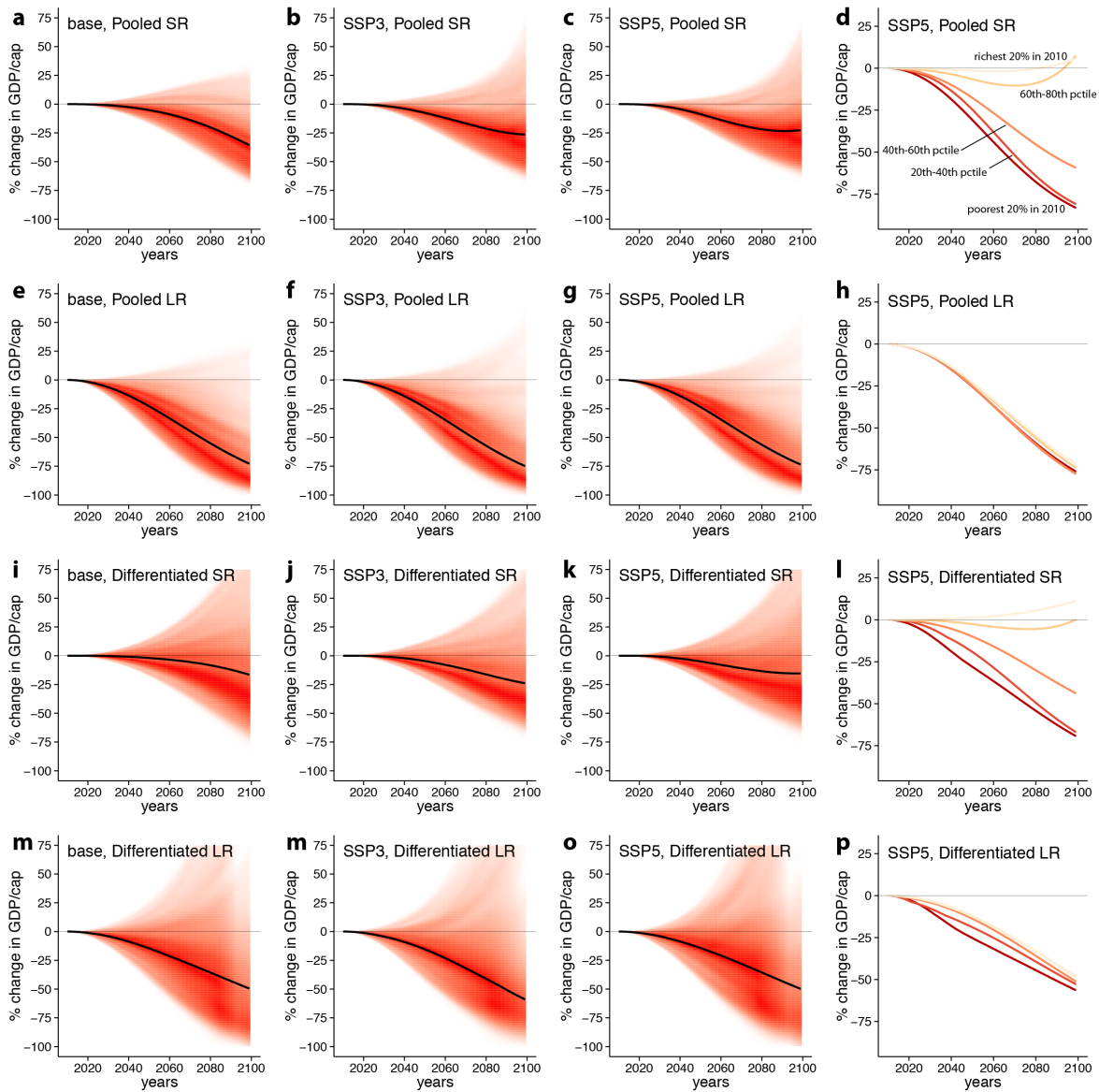
Extended Data Figure ED4: Projected impact of climate change (RCP 8.5) by 2100 relative to a world without climate change, for different historical response functions and different future socioeconomic scenarios. The first three columns show impacts on global per capita GDP (analogous to Fig. 5a), for the three different underlying socioeconomic scenarios and four different response functions shown in Figure 5b. Last column (d, h, l, p) shows impact on per capita GDP by baseline income quintile (as in Fig. 5c), for SSP5 and the different response functions. Colors correspond to the income quintiles as labeled in d. Globally aggregated impact projections are more sensitive to choice of response function than projected socioeconomic scenario, with response functions that allow for accumulating effects of temperature (LR) showing more negative global impacts but less inequality in these impacts.
