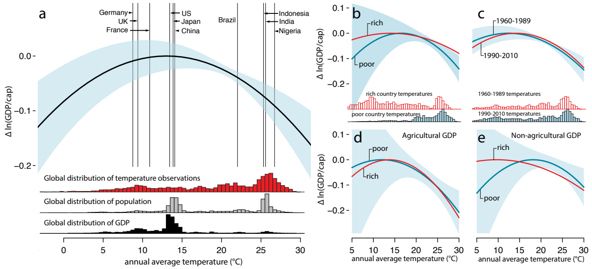
Figure 2: Effect of annual average temperature on economic production. (A) Global nonlinear relationship between annual average temperature and change in log GDP per capita (thick black line, relative to optimum) during 1960-2010 with 90% C.I. (blue, clustered by country). Model includes country fixed effects, flexible trends, and precipitation controls (see SI). Vertical lines indicate average temperature for selected countries, although averages are not used in estimation. Histograms show global distribution of temperature exposure (red), population (grey), and income (black). (B) Comparing rich (above median, red) and poor (below median, blue) countries. Blue shaded region is 90% C.I. for poor countries. Histograms show distribution of country-year obs. (C) Same as (B) but for early (1960-89) and late (1990-2010) subsamples (all countries). (D) Same as (B) but for agricultural income. (E) Same as (B) but for non-agricultural income.
