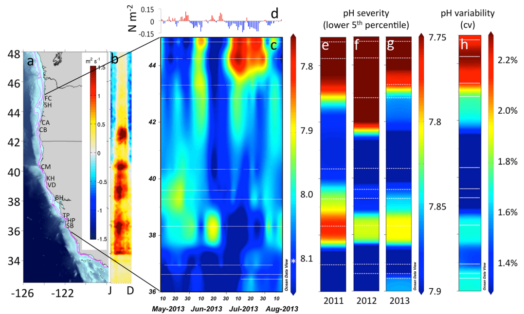
Figure 1. (a) Intertidal \text{pH}_{\text{total}} variation across the CCLME study domain of contrasting shelf topography as delineated by the 75 m, 100 m, 200 m isobaths (magenta), and (b) wind-driven cross-shelf surface transport ( \text{m}^2 \text{s}^{-1} ) (see scale inset in a). Map was generated from the ETOPO1 dataset 42 in Matlab v8.2 ( http://www.mathworks.com/products/matlab ). (c) Variation in pH at the event-scale during part of the 2013 upwelling season with asterisk denoting global mean surface \text{pH}^{12} and (d) accompanying daily wind stress ( \text{N m}^{-2} ) at 44.65^\circ\text{N} , (e–g) severity of low pH exposure (lower 5 th percentile) across three years of deployment and (h) pH variability. White dotted lines in pH panels denote station locations.
