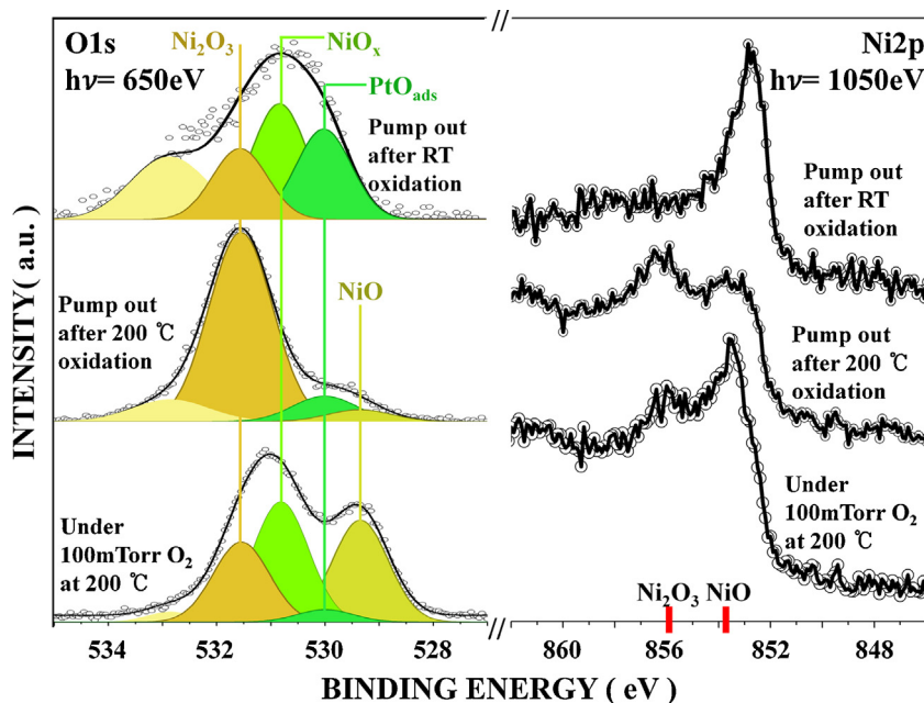
Fig. 4. O 1s and Ni 2p core-level spectra measured after oxidation processes. During the evacuation of oxygen gas, the temperature of sample is maintained at T=200\text{ }^{\circ}\text{C} and RT separately.
