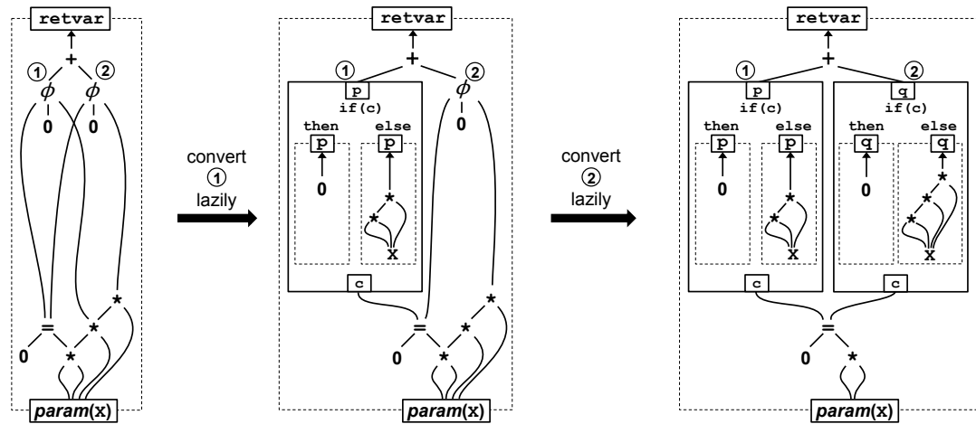
Figure 8.11. Conversion of \phi nodes to revised branch nodes
