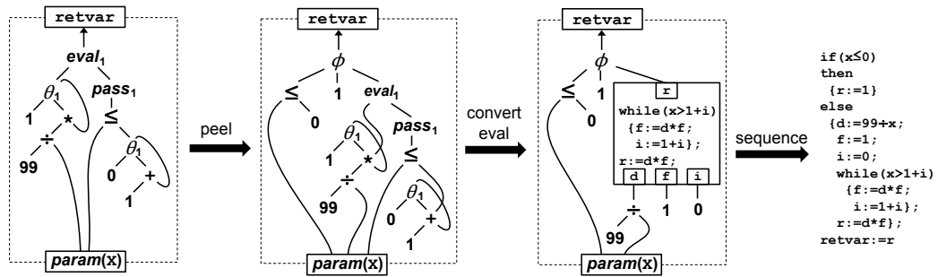
Figure 8.17. Reversion of a PEG after peeling the loop once
