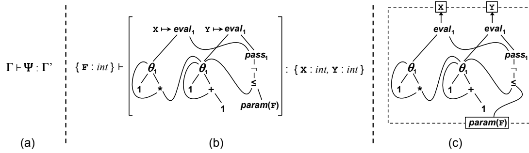
Figure 8.2. Visual representation of the judgement for CFG-like PEG contexts: (a) shows the syntactic form of the judgement; (b) shows an example of the syntactic form; and (c) shows the same example in visual form
