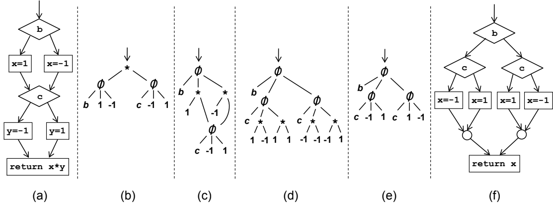
Figure 4.2. An example of how local changes in the PEG can cause large changes in the CFG: (a) the original CFG, (b) the original PEG, (c) the PEG after distributing * through the left-hand \phi , (d) the PEG after distributing * through the bottom \phi , (e) the PEG after constant folding, (f) the resulting CFG
