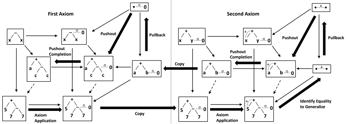
Figure 15.1. Example of generalization using E-PEGs
