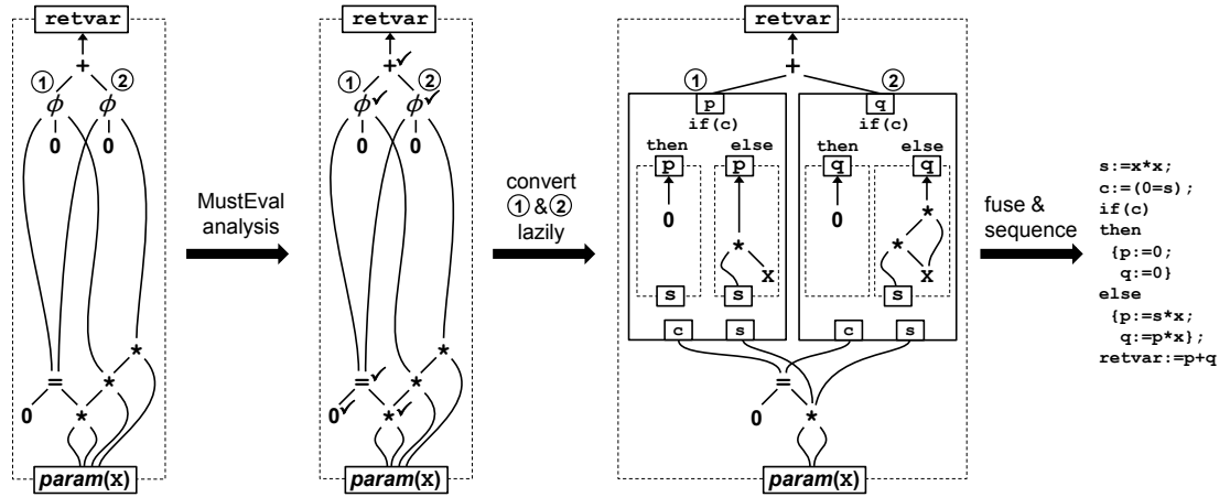
Figure 8.14. Same example as in Figure 8.11, but this time hoisting redundancies from branches
