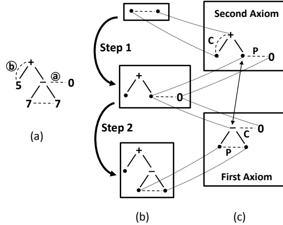
Figure 13.3. Example showing how generalization works
