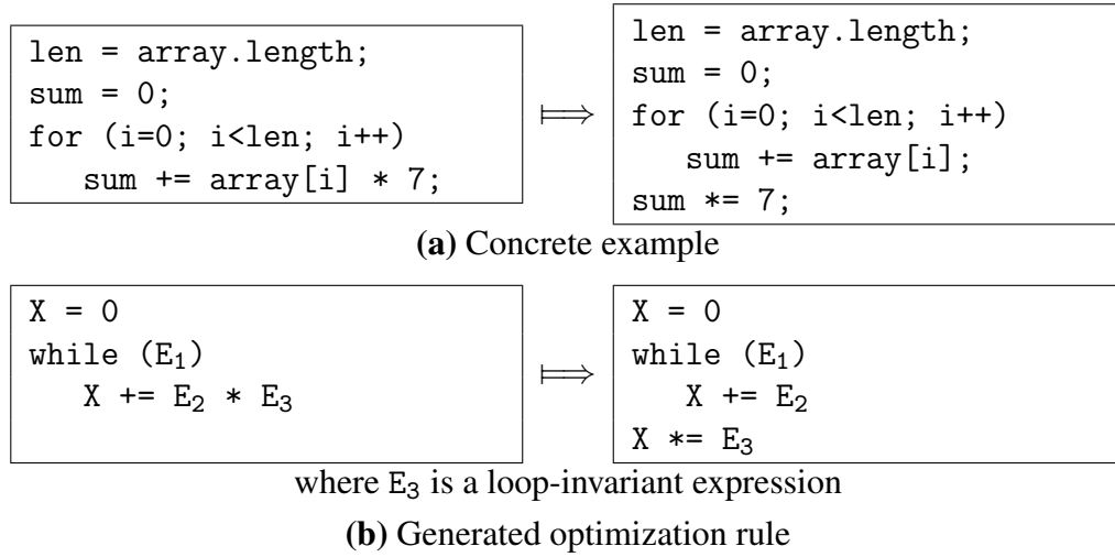
Figure 18.3. Loop-operation factoring
