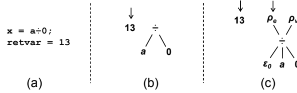
Figure 7.6. Representation of a division by zero: (a) the original source code, (b) the PEG produced without effect witness, and (c) the PEG produced with effect witnesses. The arrows indicate the return values.
