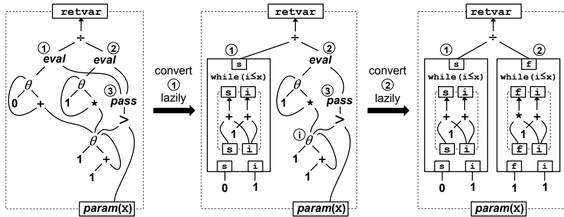
Figure 8.8. Conversion of eval nodes to revised loop nodes
