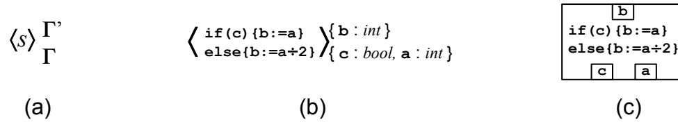
Figure 8.3. Diagrammatic representation of a statement node
