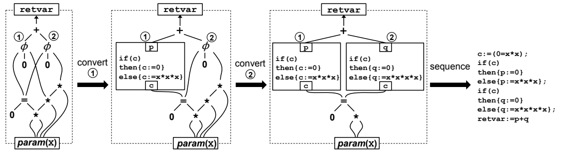
Figure 8.10. Reversion of a PEG without applying branch fusion
