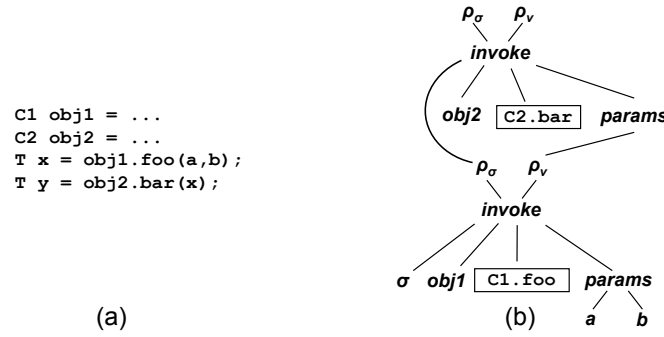
Figure 10.1. Representation of Java method calls in a PEG: (a) the original Java source code and (b) the corresponding PEG
