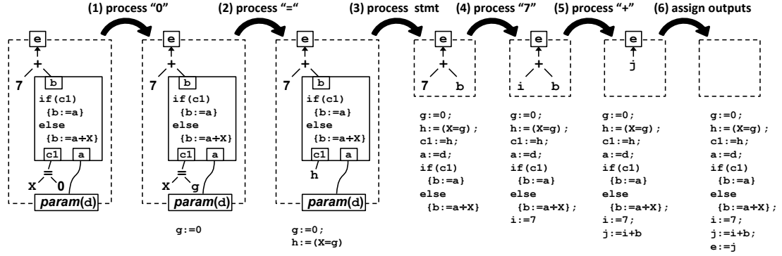
Figure 8.6. Example of sequencing a PEG context (with statement nodes) into a statement
