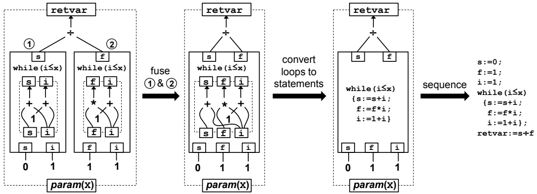
Figure 8.9. Fusion of loop nodes
