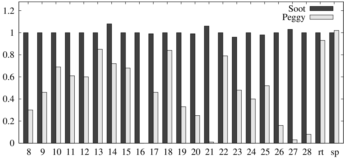
Figure 11.2. Run times of generated code from Soot and Peggy, normalized to the runtime of the unoptimized code. The x-axis denotes the optimization number from Figure 11.1, where “rt” is our raytracer benchmark and “sp” is the average over the SpecJVM benchmarks.
