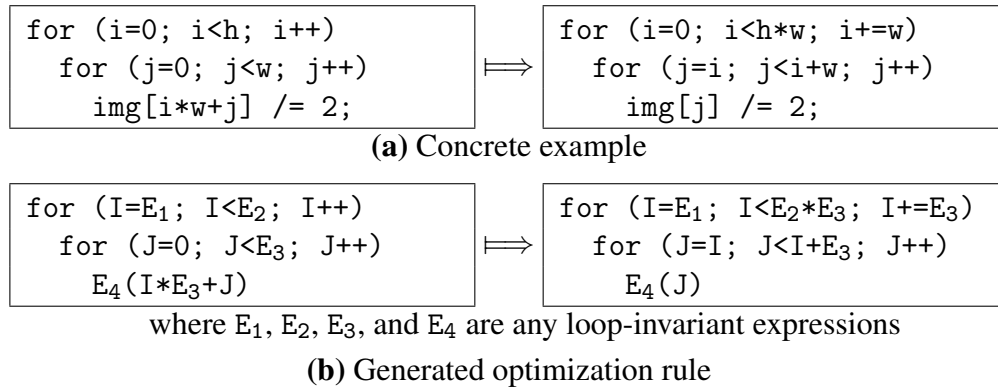
Figure 18.2. Generalized inter-loop strength reduction
