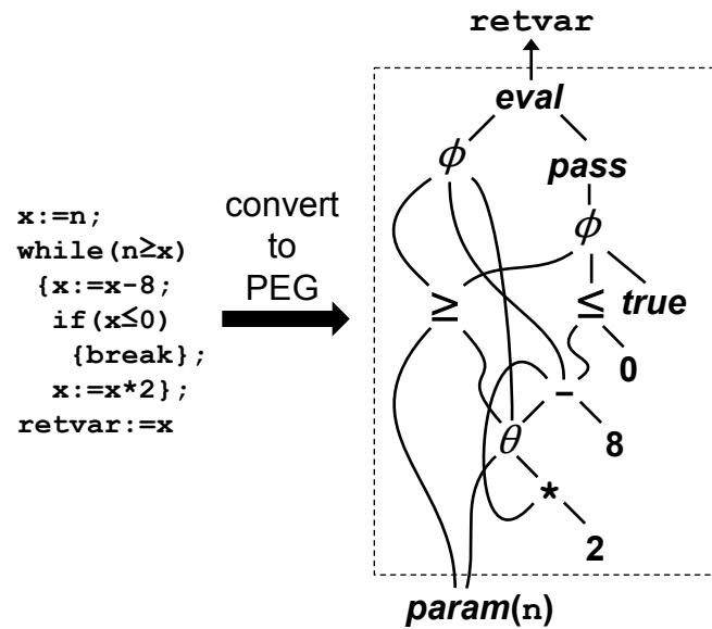
Figure 8.18. Conversion of a SIMPLE program with a break to a PEG
