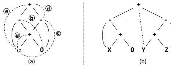
Figure 13.2. Example showing the need for splitting
