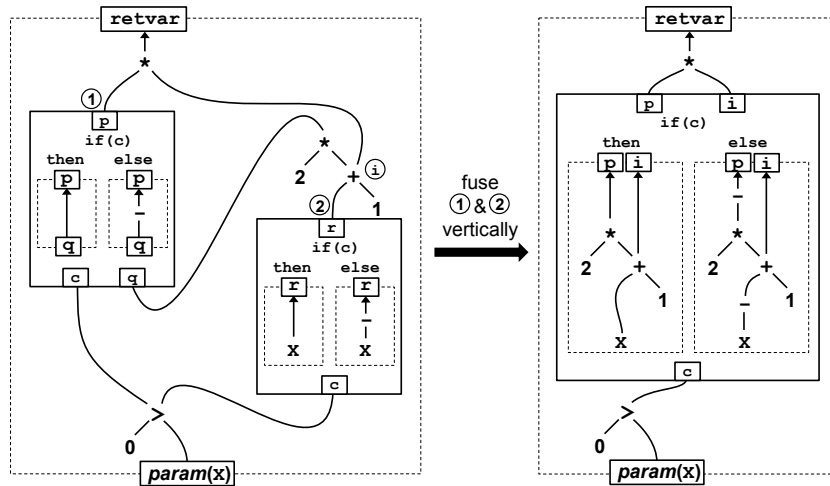
Figure 8.13. Vertical fusion of branch nodes
