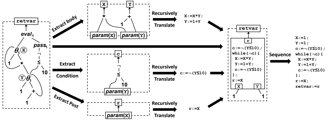
Figure 8.4. Example of converting eval nodes to while-loop statement nodes
