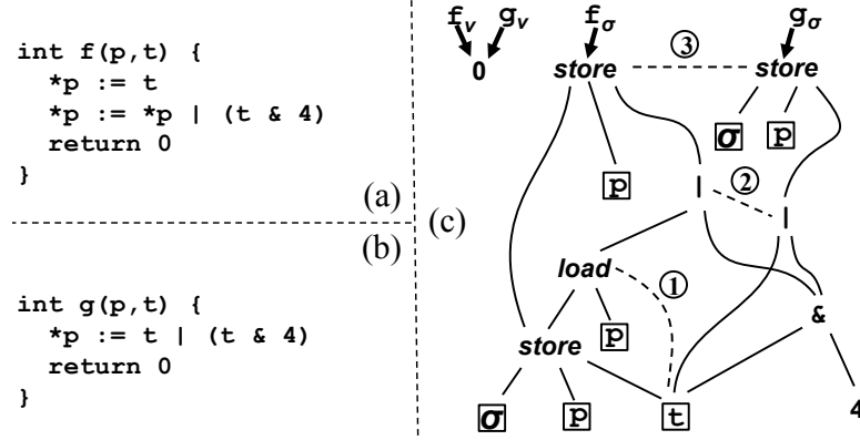
Figure 12.1. (a) Original code (b) Optimized code (c) Combined E-PEG
