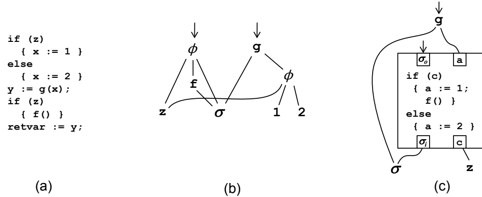
Figure 10.2. Example demonstrating challenges of linearizing heap values.
