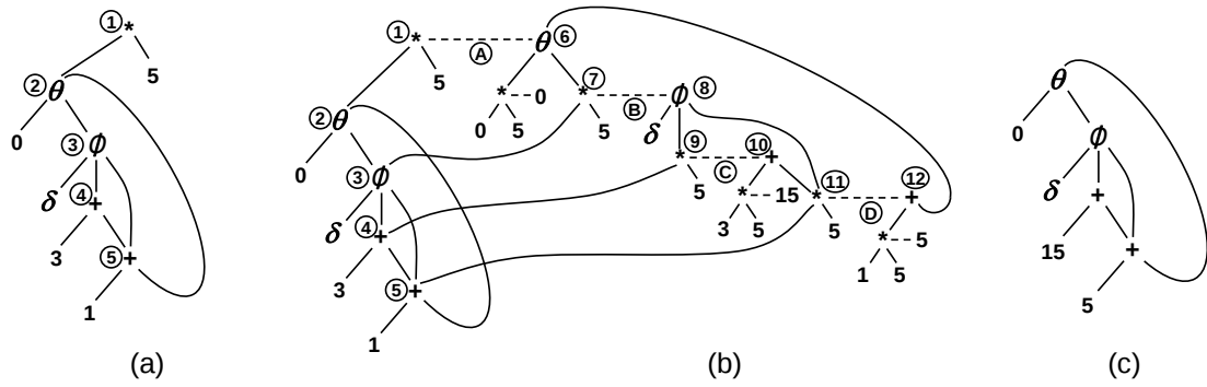
Figure 2.2. Loop-induction-variable Strength Reduction using PEGs: (a) shows the original PEG, (b) shows the E-PEG that our engine produces from the original PEG, and (c) shows the optimized PEG, which results by choosing nodes 6, 8, 10, and 12 from (b)
