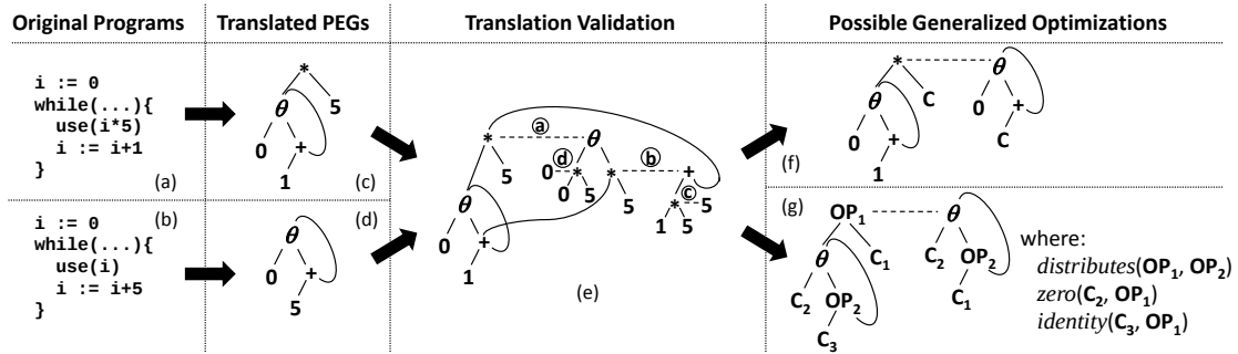
Figure 13.1. Learning loop-induction-variable strength reduction from an example
