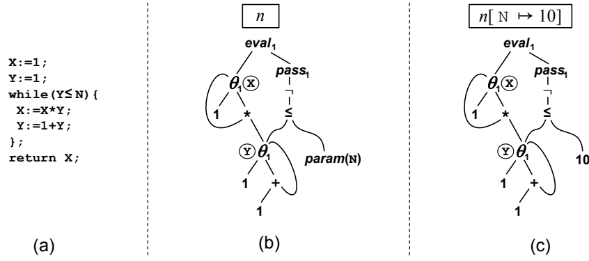
Figure 6.2. Example showing a PEG with parameter nodes: (a) shows code for computing the factorial of N , where N is a parameter; (b) shows the PEG with n being the value returned; and (c) shows n[N \mapsto 10] , which is now a PEG whose semantics is well defined in our formalism
