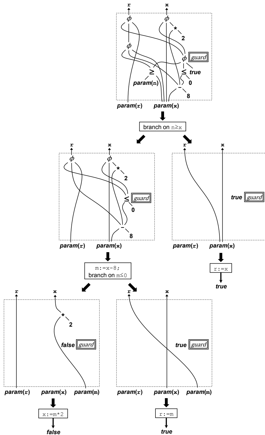
Figure 8.20. Reversion of a guarded PEG context to a CFG with exits marked true/false
