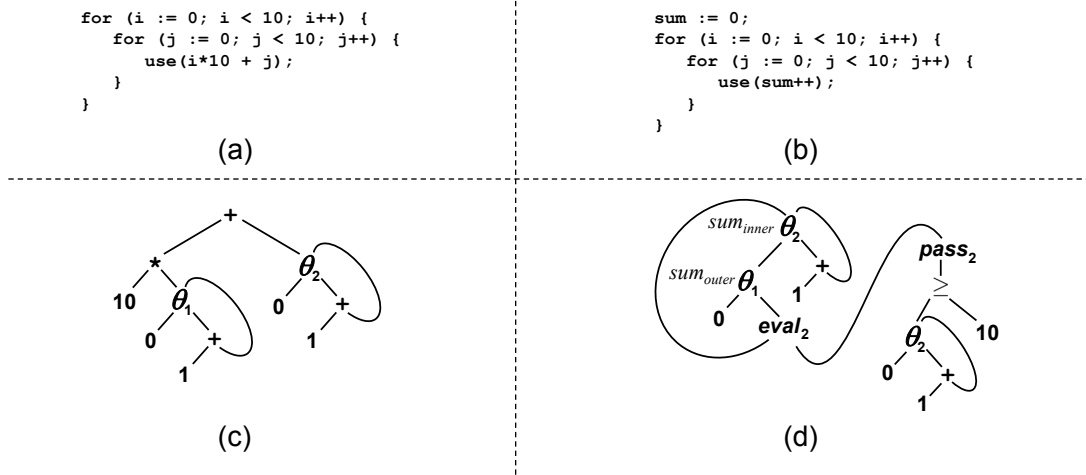
Figure 3.2. Two equivalent loops and their PEG representations. The PEGs for the expressions inside the use statements in (a) and (b) are shown in (c) and (d), respectively.
