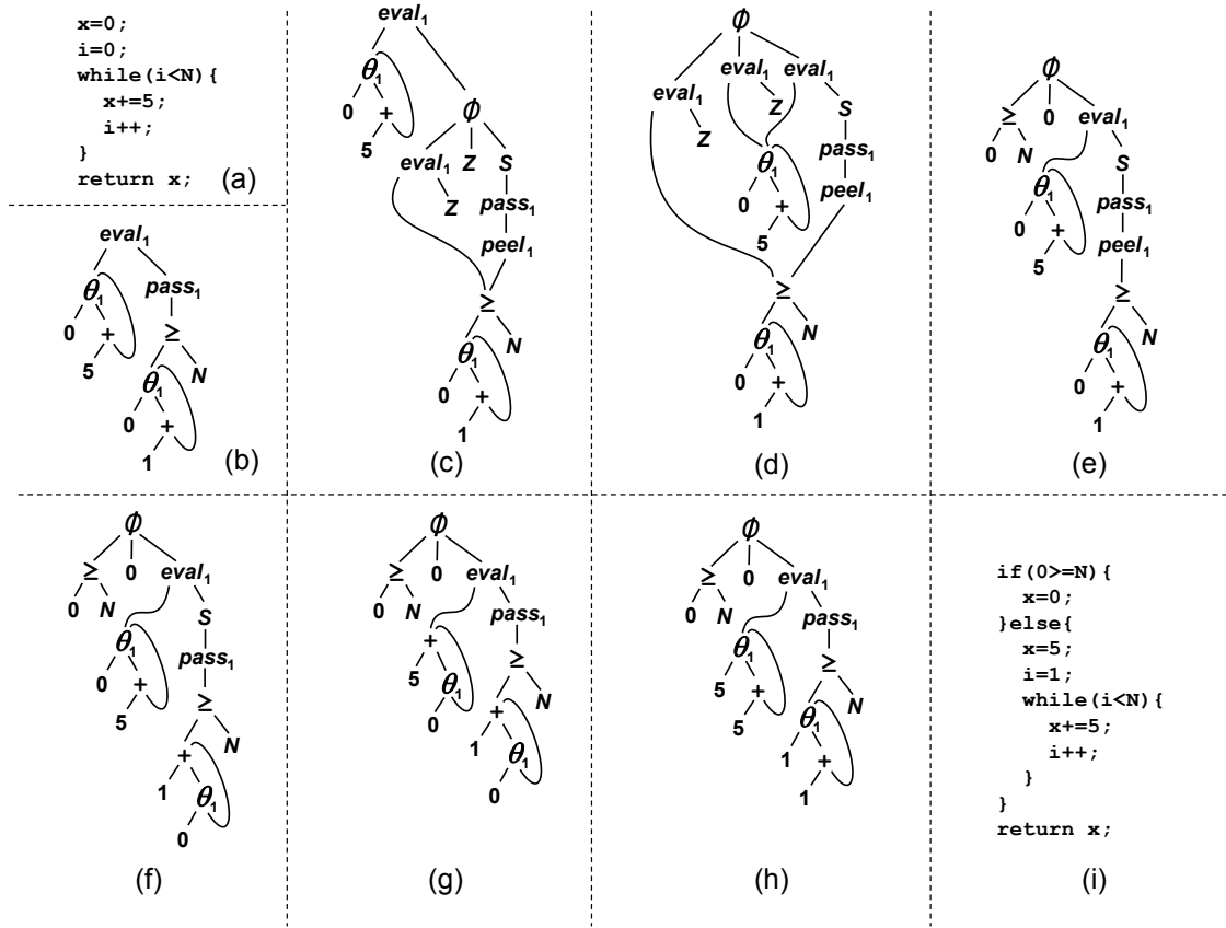
Figure 4.3. An example of axiom-based loop peeling: (a) the original loop, (b) the PEG for part (a), (c)-(h) intermediate steps of the optimization, (i) the final peeled loop, which is equivalent to (h)
