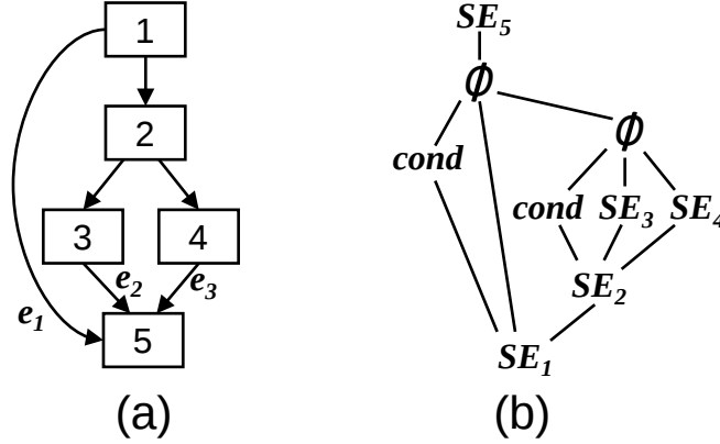
Figure 7.7. Sample CFG and corresponding A-PEG
