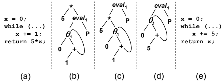
Figure 4.1. An example of loop-based code motion from simple axiom applications; (a) the original source code, (b) the original PEG, (c) the PEG after distributing * through eval_1 , (d) the PEG after performing loop-induction-variable strength reduction, (e) the resulting source code
