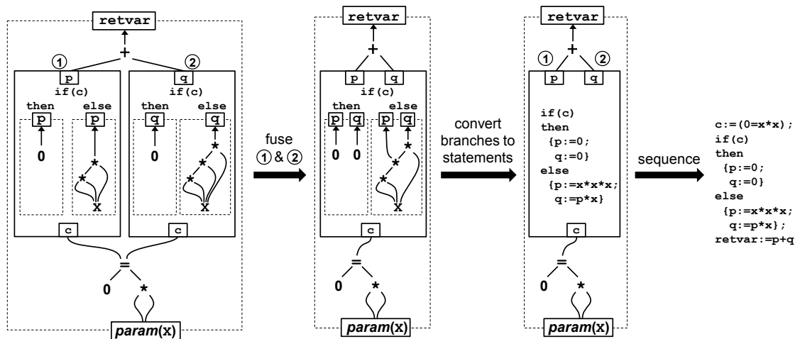
Figure 8.12. Fusion of branch nodes
