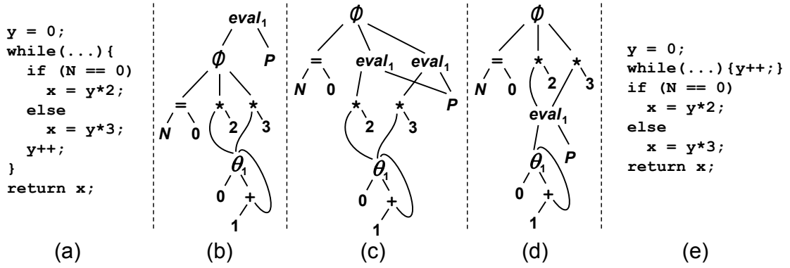
Figure 4.4. An example of branch hoisting: (a) the original program, (b) the PEG for part (a), (c) the PEG after distributing eval through \phi , (d) the PEG after distributing eval through * , (e) the code resulting from (d)
