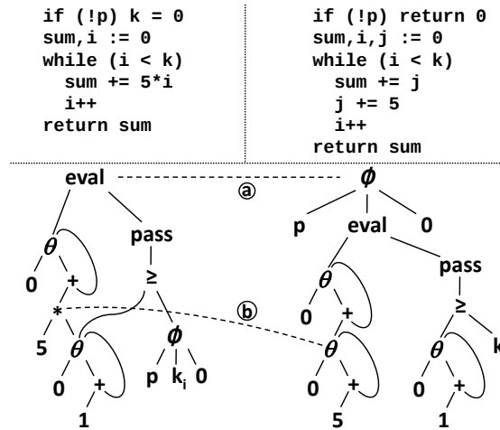
Figure 13.4. One E-PEG with conceptually two optimizations
