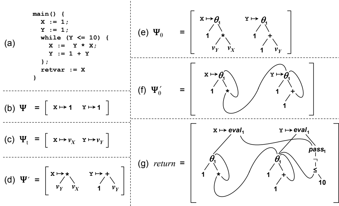
Figure 7.4. Steps of the translation process: (a) shows a SIMPLE program computing the factorial of 10; (b) through (f) show the contents of the variables in TS when processing the while loop; and (g) shows the return value of TS when processing the while loop
