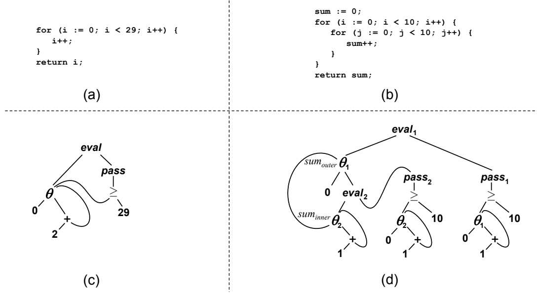
Figure 3.1. Two loops and their PEG representations
