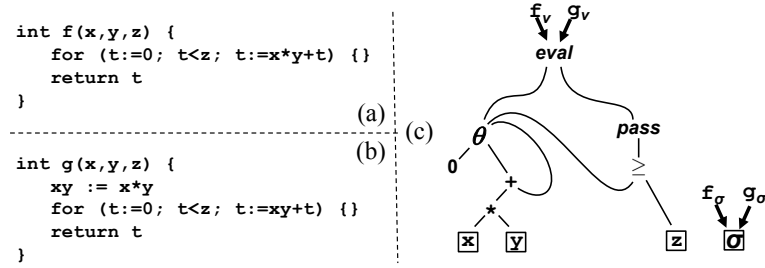
Figure 12.3. (a) Original code (b) Optimized code (c) Combined E-PEG
