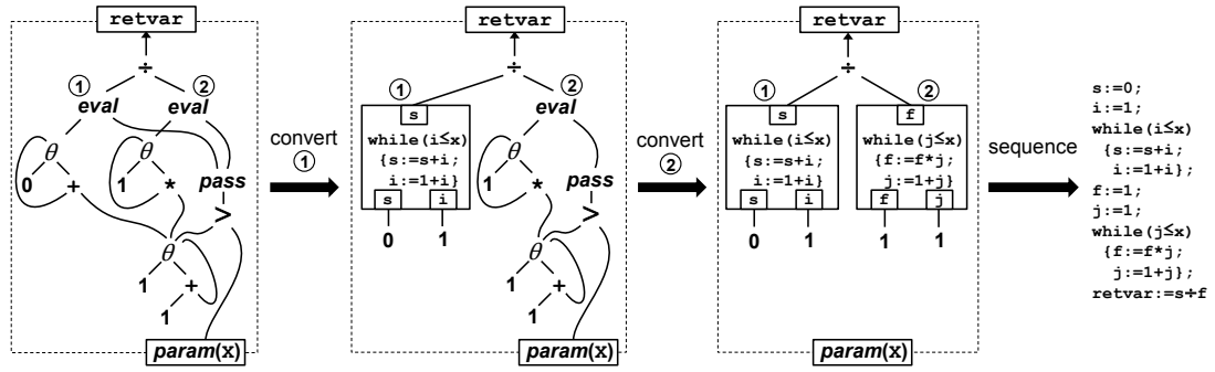
Figure 8.7. Reversion of a PEG without applying loop fusion
