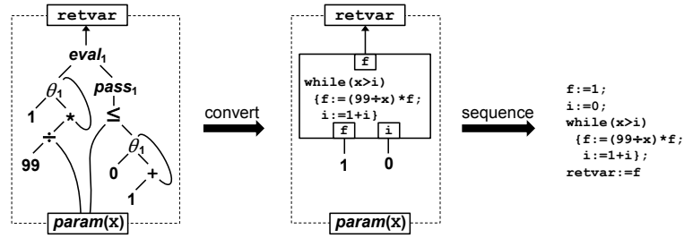
Figure 8.15. Reversion of a PEG without applying loop-invariant code motion
