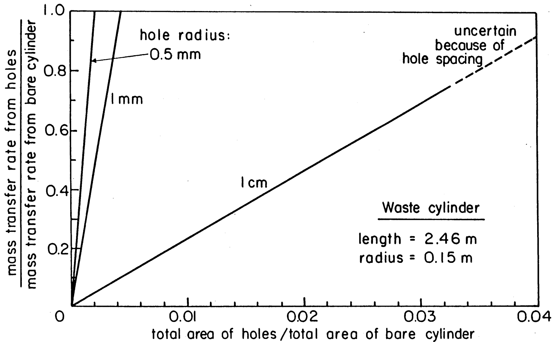
Figure 2. Radionuclide Fluxes from Multiple Holes and a Bare Waste Cylinder
