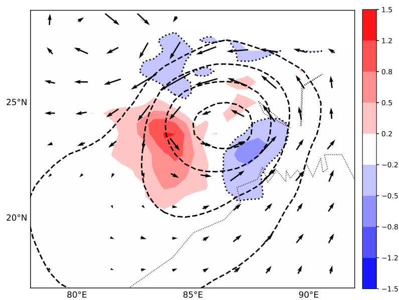
Figure 15. Perturbation vertical velocity ( w' , shading, \text{cm s}^{-1} , averaged from 1.2 to 5.3 km) and perturbation winds ( v' , vectors, 3.1 km) for Exp. C at 72 hours into the simulation. Negative values of w' are enclosed with a dotted line.
