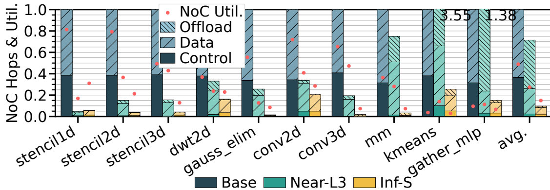
Figure 7.12: NoC Traffic Breakdown (Bar) and Util. (Dot)
