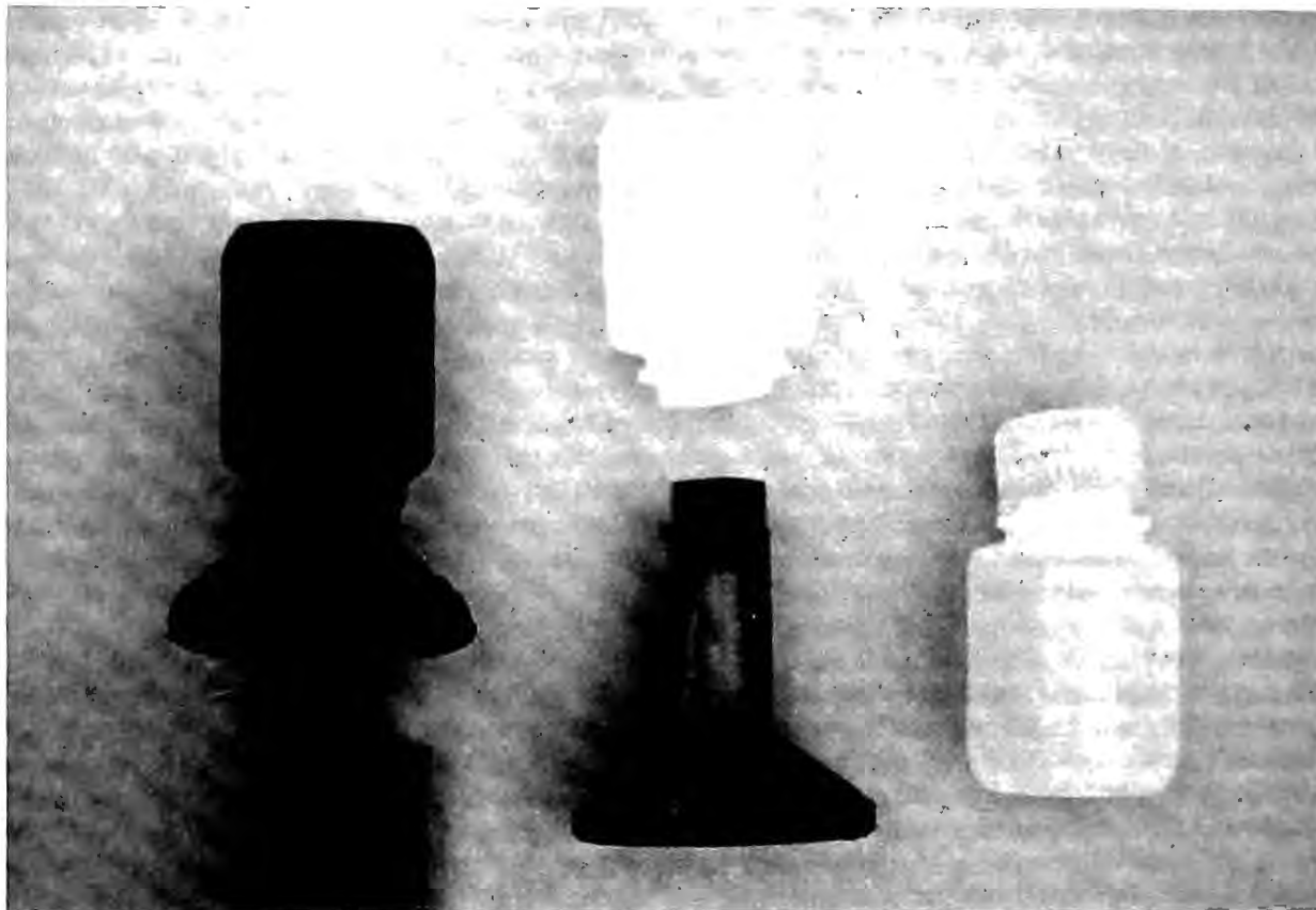
Fig. 1. Components of a Coyote Lure Operative Device (CLOD). From L to R, an assembled CLOD, covered with a layer of black plastic, screwed onto an angle-iron stake (driven into the ground), the commercial labware vial modified to slip over the stem of the acrylic CLOD core, and the labware vial as received from the manufacturer.
