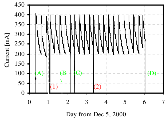
Figure 1: Beam current over time in the selected typical week, December 5-11.
