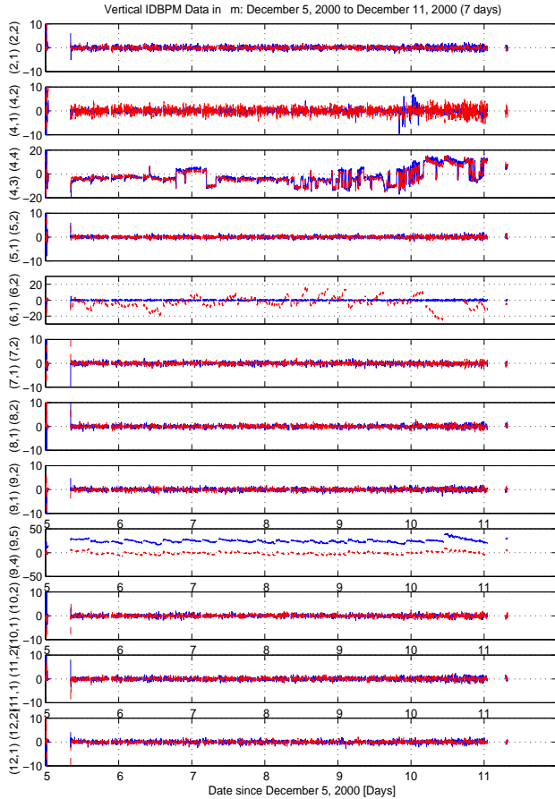
Figure 4: Vertical beam motion (December 5-11) at upstream and downstream ends of straight sections, in the center of sector 4 straight (4,3 & 4,4) and in the center of sector 9 arc (9,4 & 9,5).
