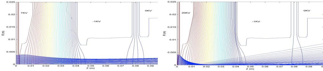
Figure 3. IMPACT-T simulation of the beam emerging from the RIA ECR ion source showing the effect of electrode voltage on the beam quality emerging from the source. Left: correct voltage. Right: incorrect voltage (J. Qiang, LBNL).
