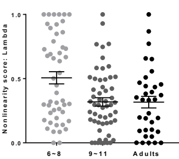
Figure 3. Distribution of nonlinearity score across age groups
