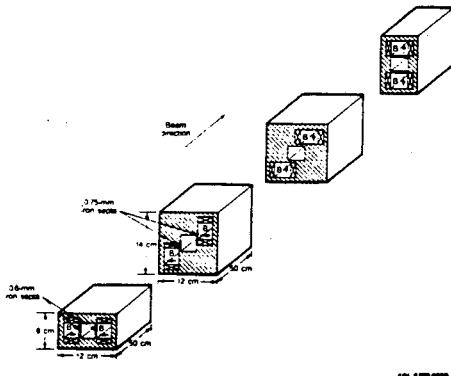
Figure 3. Emittance Exchanger
