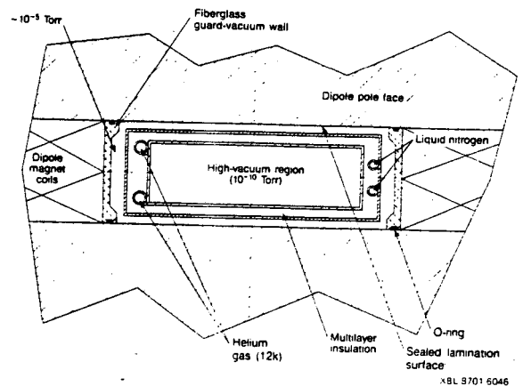
Figure 4. Vacuum Chamber Cross Section
