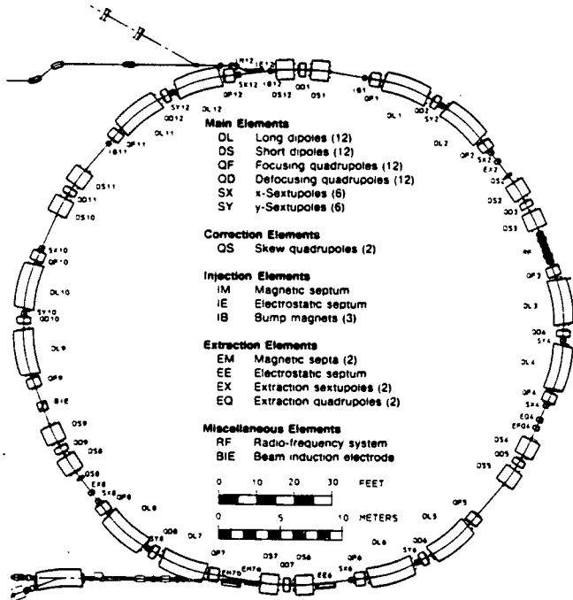
Figure 2. Accelerator Lattice
