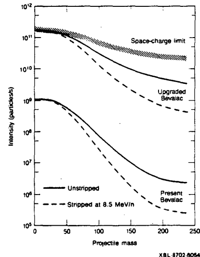
Figure 1. Intensity per Pulse vs Projectile Mass
