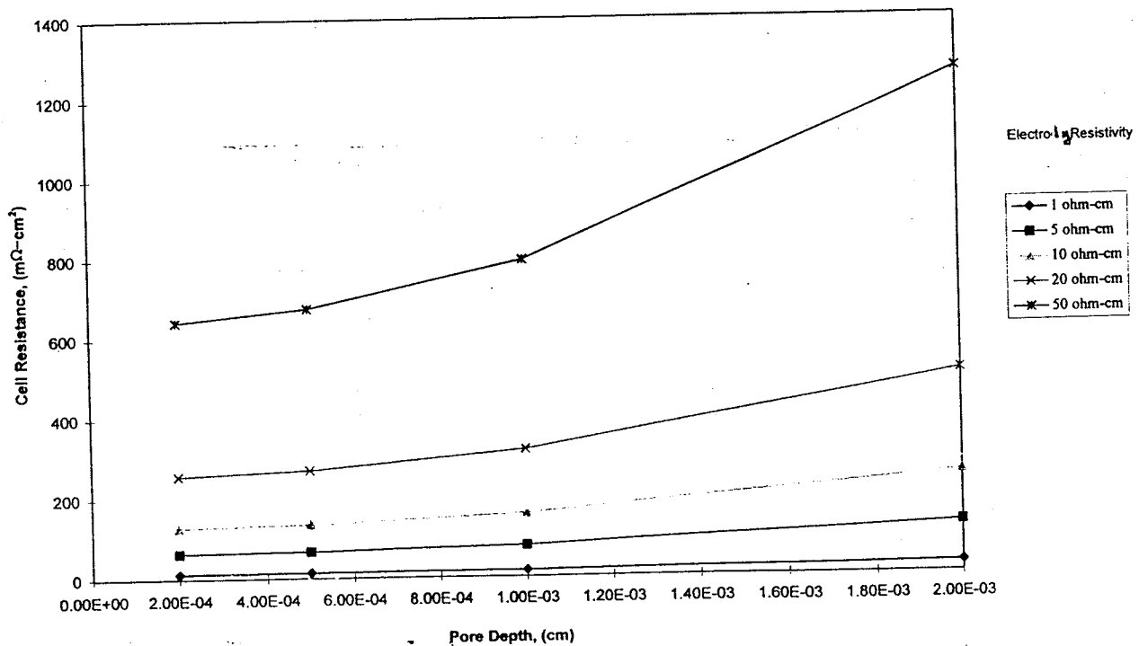
Figure 23: Projections of cell resistance ( \text{ohm-cm}^2 ) for various designs as a function of electrode material pore depth
