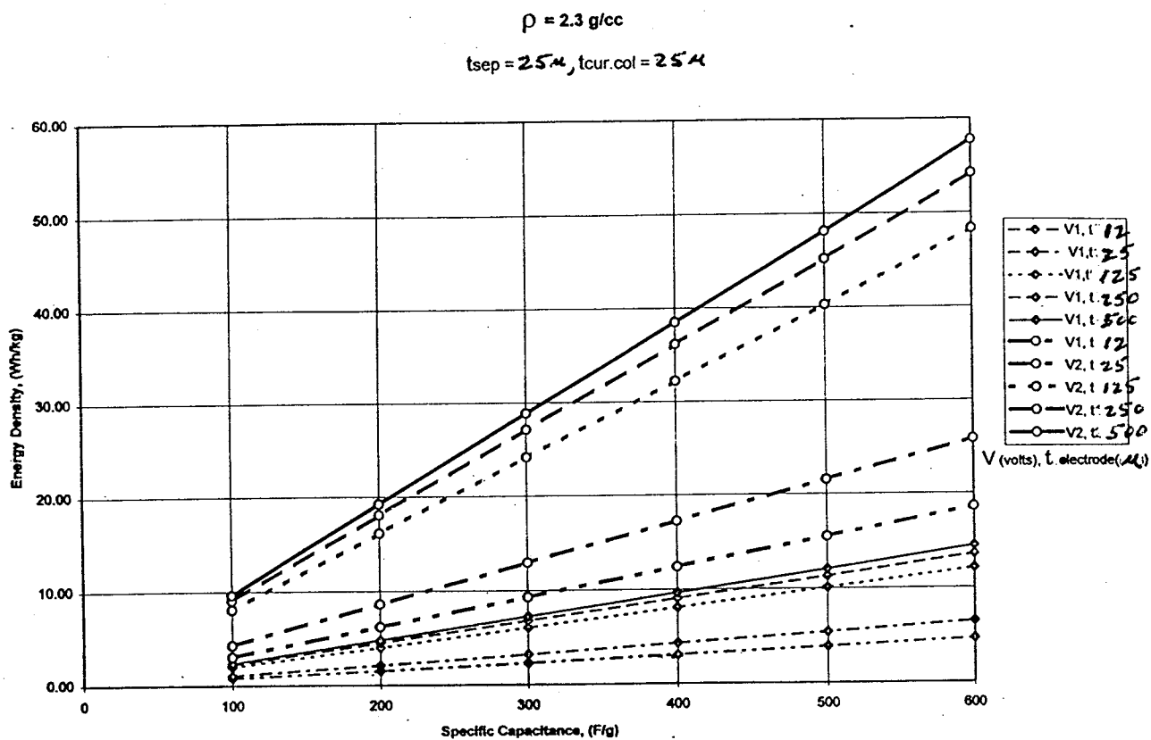
Figure 24: Projections of the energy density of ultracapacitors using mixed metal oxide electrodes for various cell designs
