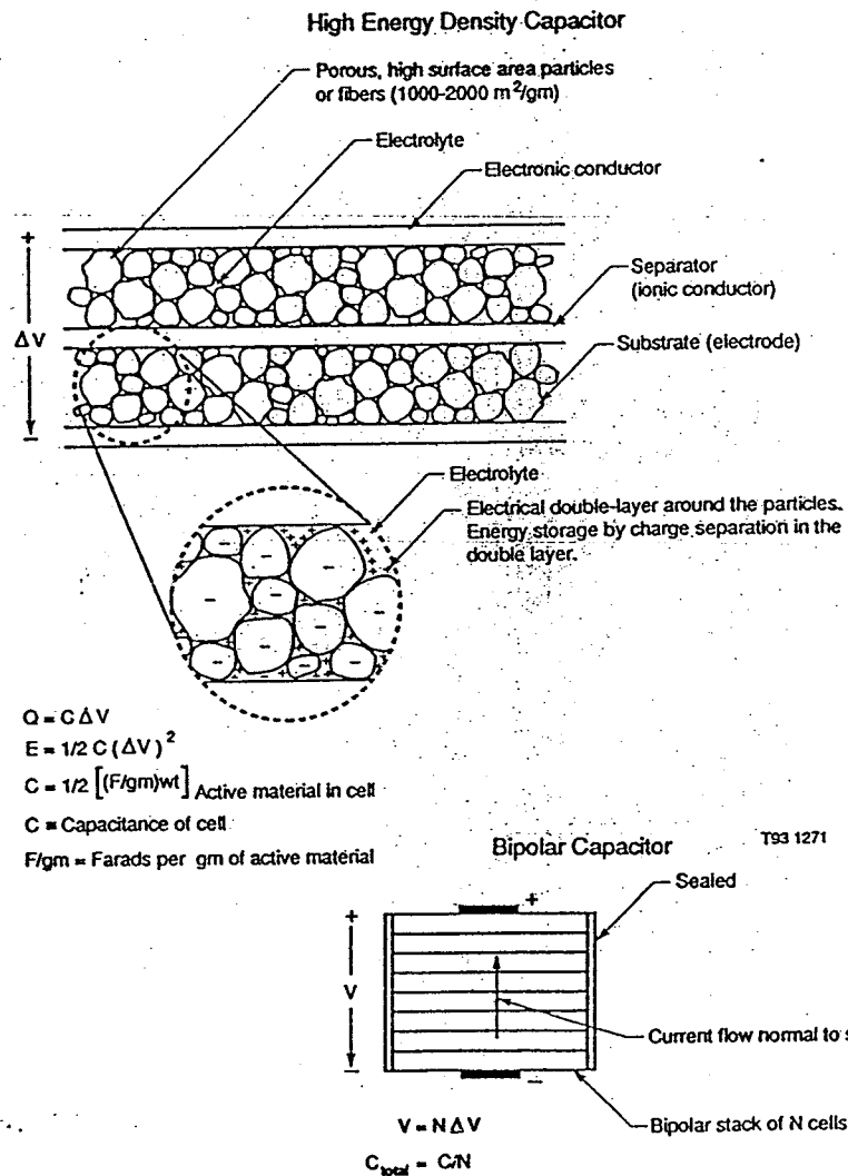
Figure 17: Schematic of an ultracapacitor cell using porous electrodes and a bipolar stack
