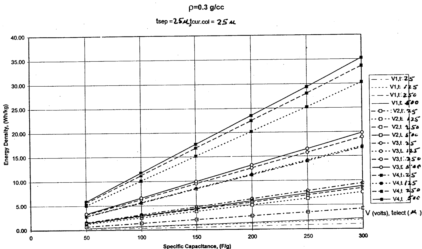
Figure 18: Projections of the energy density of carbon-based ultracapacitors of various design (carbon loading = .3 \text{ gm/cm}^3 )
