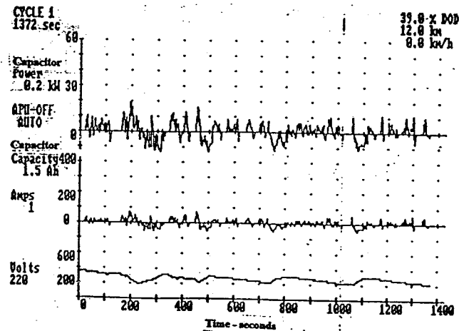
Figure 2: Discharge/charge (simulation) of a 400Wh Ultracapacitor in a Series Hybrid Passenger Car on the Federal (USA) Urban Driving Cycle
