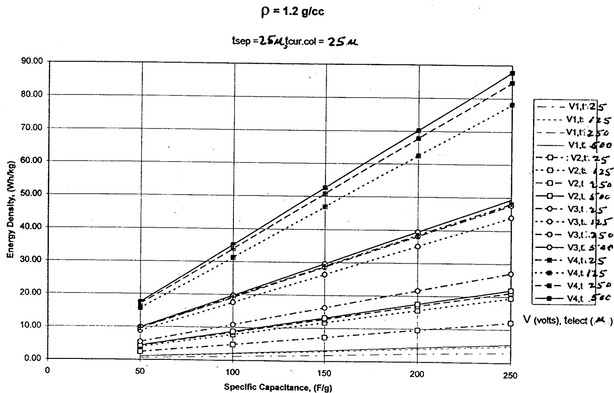
Figure 21: Projections of the energy density of carbon-based ultracapacitors of various design (carbon loading = 1.2 \text{ gm/cm}^3 )
