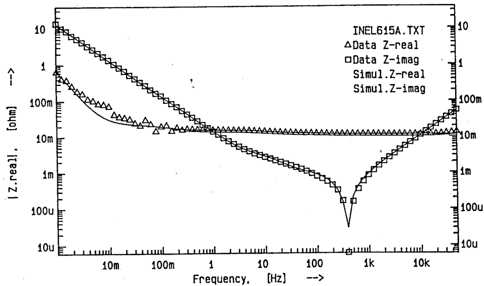
Figure III-9: AC Impedance data for the 1V Maxwell Capacitor
