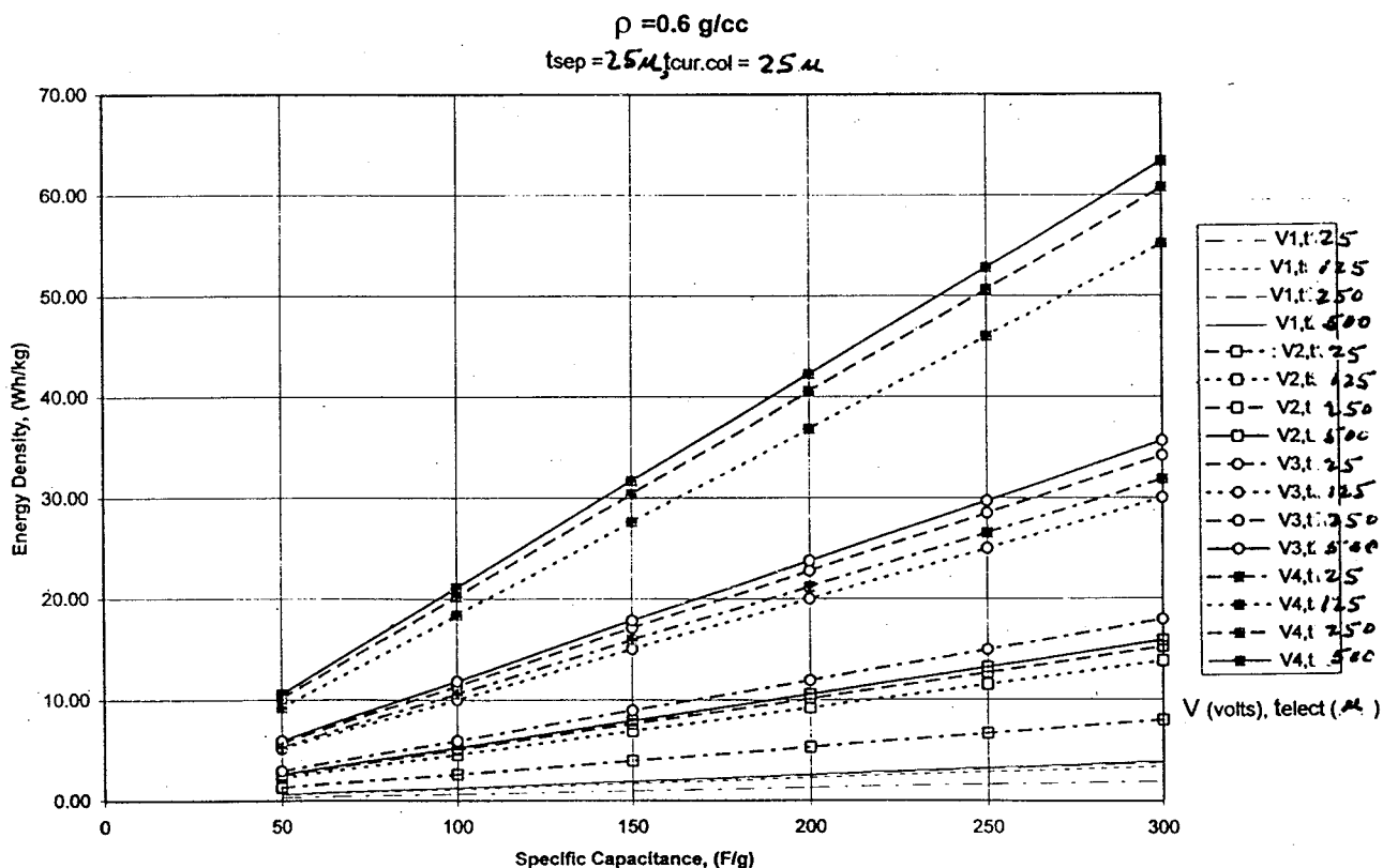
Figure 19: Projections of the energy density of carbon-based ultracapacitors of various design (carbon loading = .6 \text{ gm/cm}^3 )
