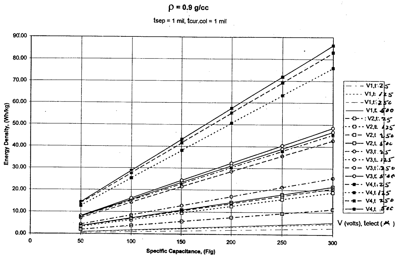
Figure 20: Projections of the energy density of carbon-based ultracapacitors of various design (carbon loading = 0.9 \text{ gm/cm}^3 )
