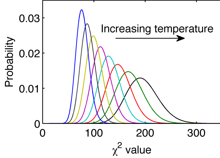
Figure 3.1: Annealed or tempered likelihood functions as a function of their \chi^2 misfit. Note how the leftmost likelihood function at T = 1 is narrow and peaked, which can manifest as a model space which is harder to sample.
