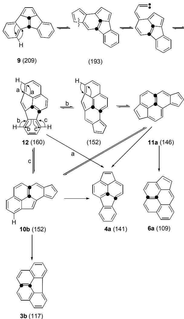
Figure 1. The major isotopomers isolated from the FVP of 2a and their relative abundances, based on normalized ^{13}\text{C} NMR signal intensities.
