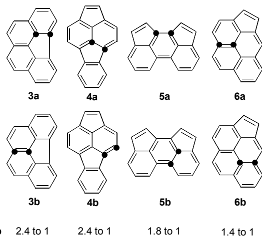
Figure 1. The major isotopomers isolated from the FVP of 2a and their relative abundances, based on normalized ^{13}\text{C} NMR signal intensities.
