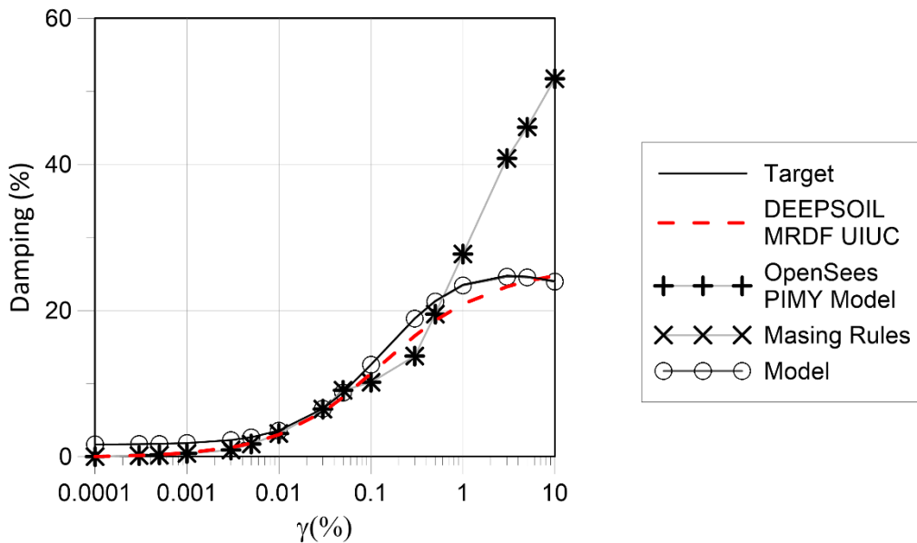
Figure 5. Hysteretic damping curves predictions of different models for a clay PI=40 \sigma'_v=47.5 kPa, \gamma=15 kN, V_s=80 m/s, OCR=1.15 K_0=0.5 .
