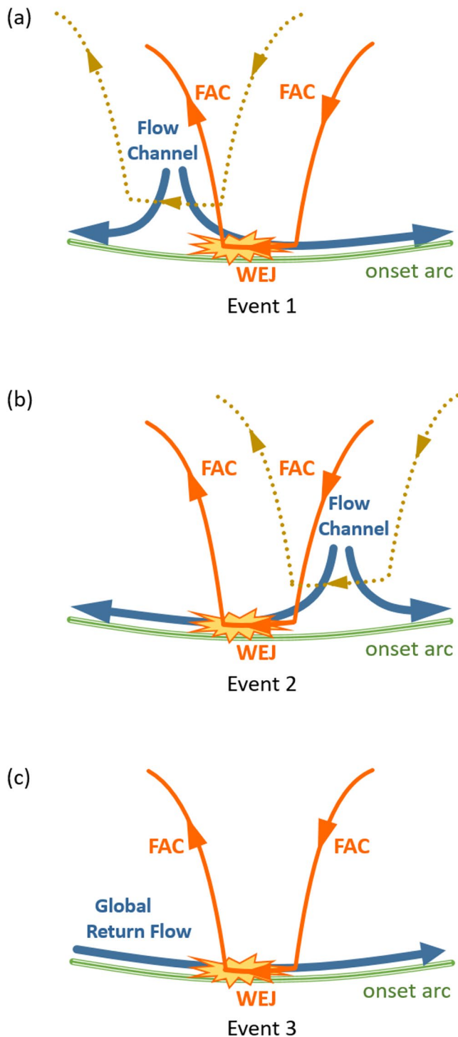
Figure 8. Schematic illustration of the location of auroral breakup relative to the pre-onset equatorward flow channel and wedge current systems expected for the flow braking (dotted yellowish brown) and auroral breakup (orange) for (a) Event 1, (b) Event 2, and (c) Event 3.
