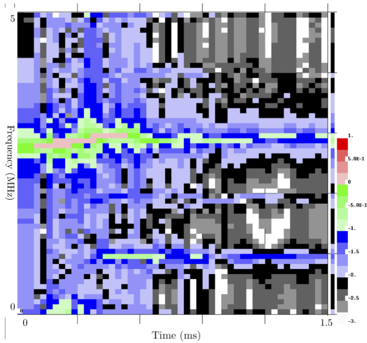
Figure 3.6: Direct excitement of pump wave and subsequent growth of daughter wave. Frequency is on the vertical axis at left, time is on the horizontal axis, and amplitude is represented in a logarithmic scale by the colors on the scale at right.
