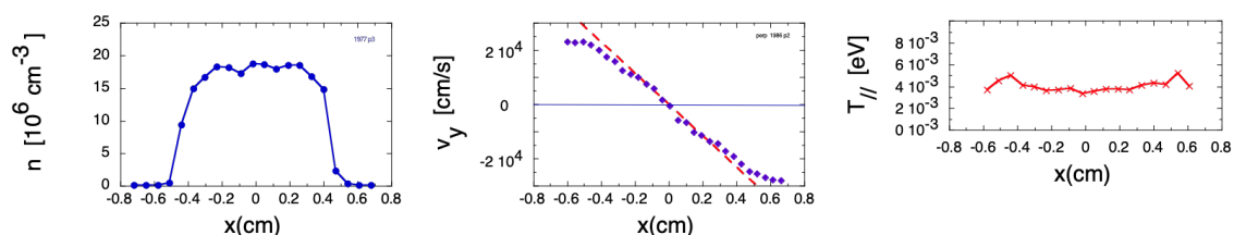
Figure 2.1: Plasma profiles for (a) density, (b) rotation, and (c) temperature. The linear fit shown on plot (b) in red shows that the rotational velocity is constant, with f_{E \times B} = 9 \text{ kHz} and radial dimension x .
