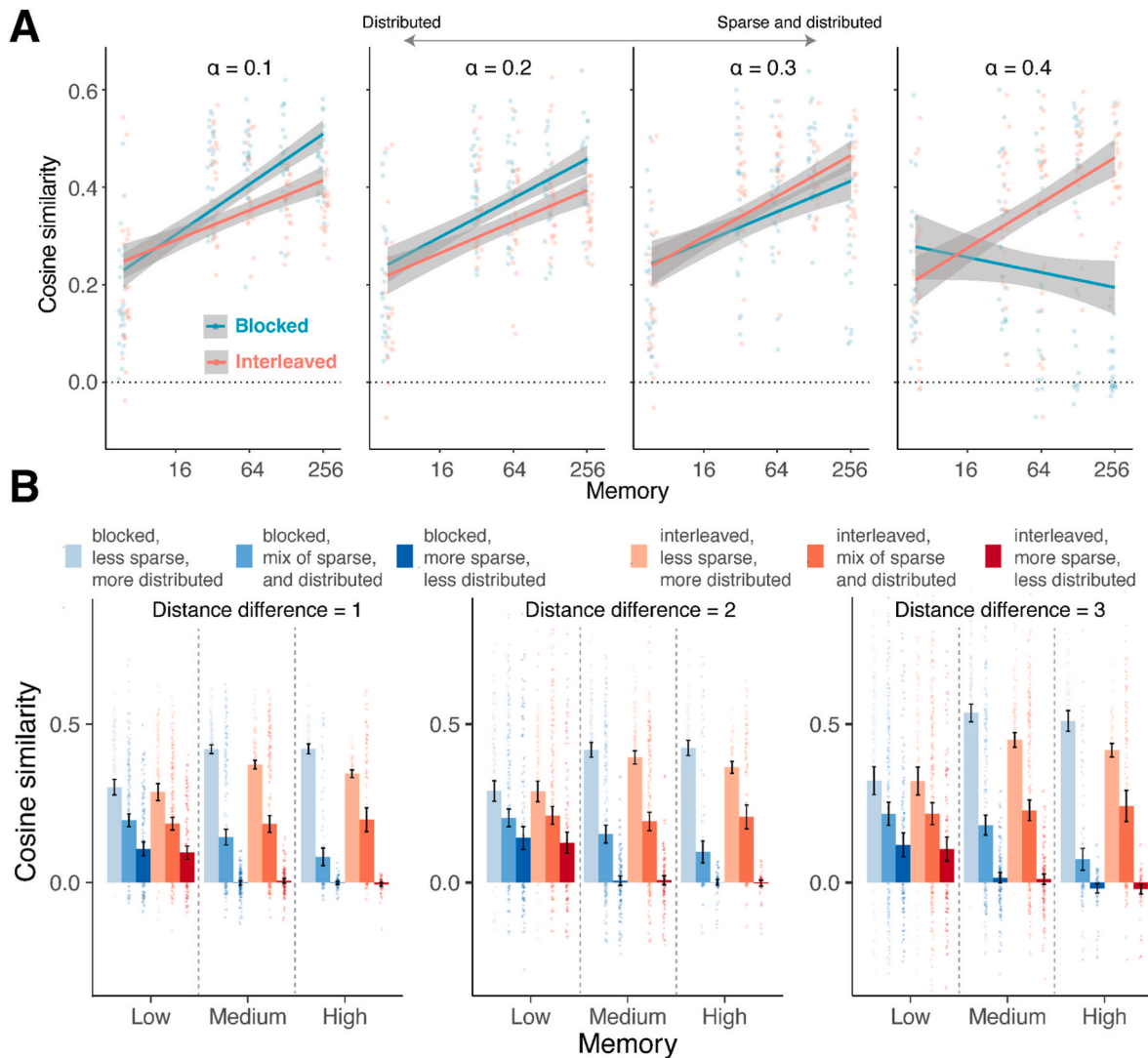
Fig. 6. Effect of sparse and distributed codes on integration of task representations. (A) For correct trials, the integration value is calculated as how much more similar the correct pair became after training compared to the incorrect pair. The relationship between integration and memory differs across different levels of \alpha . As sparsity ( \alpha ) increases towards a mixture of sparse and distributed representations, integration is more likely to occur in high memory capacity conditions after interleaved training. (B) An analysis of the full range of sparsity and entropy levels. When coding strategies have mixed sparsity and distributedness (mixed local and distributed coding), high memory capacity conditions support integration when trained via an interleaved schedule versus a blocked schedule. In contrast, when coding strategies are less sparse and more distributed, higher memory capacity conditions support integration when trained via a blocked schedule versus an interleaved schedule. These effects are consistent across levels of task difficulty (distance differences).
