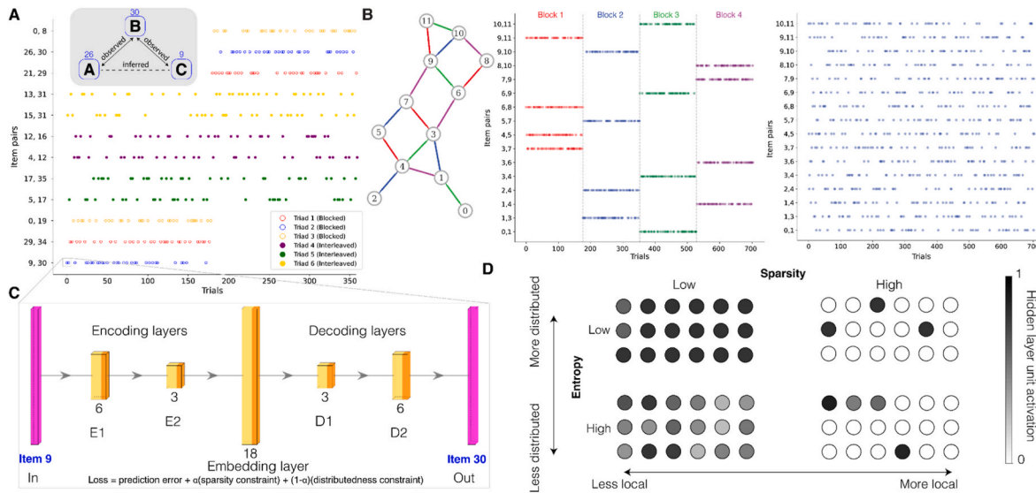
Fig. 1. Tasks and models. (A) Structural inference in simple triad graphs. Models are trained to predict paired sequences then tested on an inference task. Inset: Triad with solid arrows showing observed associations and dashed line showing the unobserved association that must be inferred. Items were organized into 6 triads (colors) in a blocked (open circles) and interleaved schedule (filled circles). (B) Neural networks were also trained to perform structural inference across an entire graph. A different set of models were trained to learn a sequence of edges drawn from a latent graph structure. Edges are colored according to the blocked schedule, where half the models were trained with a blocked schedule. In this schedule, 4 mini-blocks were created where each block contained 4 edges that did not share any nodes with each other. (C) The neural network was trained using a loss function that penalized for errors in predicting the next item, given the current item (Chandak et al., 2024). The loss function also contained a term that encourages sparse representations with low activation strengths, inspired by energy constraints in biology. A scaling parameter, \alpha , controls the degree of sparsity. Different memory capacities were simulated by varying the size of the encoding (E1, E2) and decoding (D1, D2) layers. (D) The loss function encourages localist versus distributed codes in the 18 embedding layer units (circles). Sparser activation (lighter colors) characterize more localist versus distributed codes by encouraging fewer units to activate (see Supplementary Materials, section on Defining sparsity ). We can also quantify the information content by calculating the code's entropy, where higher entropy indicates a more diverse and distributed pattern of activation to encode the same stimulus. (For interpretation of the references to color in this figure legend, the reader is referred to the Web version of this article.)
