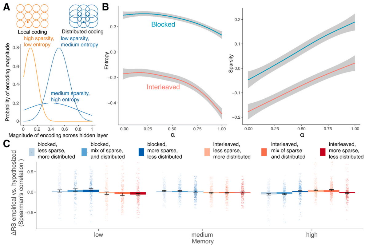
Fig. 4. Effects of sparse and distributed codes on the integration of AC representations. (A) A schematic demonstrating how local and distributed coding can be understood by the receptive field of each unit (circle) that responds to a stimulus (point). We quantify these concepts by measuring how distributedness differs according to the information content (entropy) and magnitude (sparsity) of activation in embedding layer units. The orange distribution is localist because it substantially overlaps with 0, indicating that many units are inactive. The blue curves are more distributed codes because most units are involved in coding for stimuli. The sharper blue curve (low entropy) is less distributed but has lower information content relative to the flatter blue curve (high entropy) that has a higher probability of inactive units and higher information content. (B) Different models trained with more constraints on localist memory encoding produced embedding representations with more sparsity (Pearson's r(39,036) = 0.07 , p < 0.001 ) and less entropy ( r(39,598) = -0.07 , p < 0.001 ). Models with different sparsity and distributedness constraints mimic mixed representations in hypothesized information processing pathways that use representations with both low and high sparsity or distributedness. (C) When representations are more sparse and less distributed, AC inference seems to benefit from the blocked schedule encouraging integrated representations. In contrast, when representations are less sparse and more distributed, successful AC inference tends to benefit from the interleaved schedule encouraging more integrated AC representations. (For interpretation of the references to color in this figure legend, the reader is referred to the Web version of this article.)
