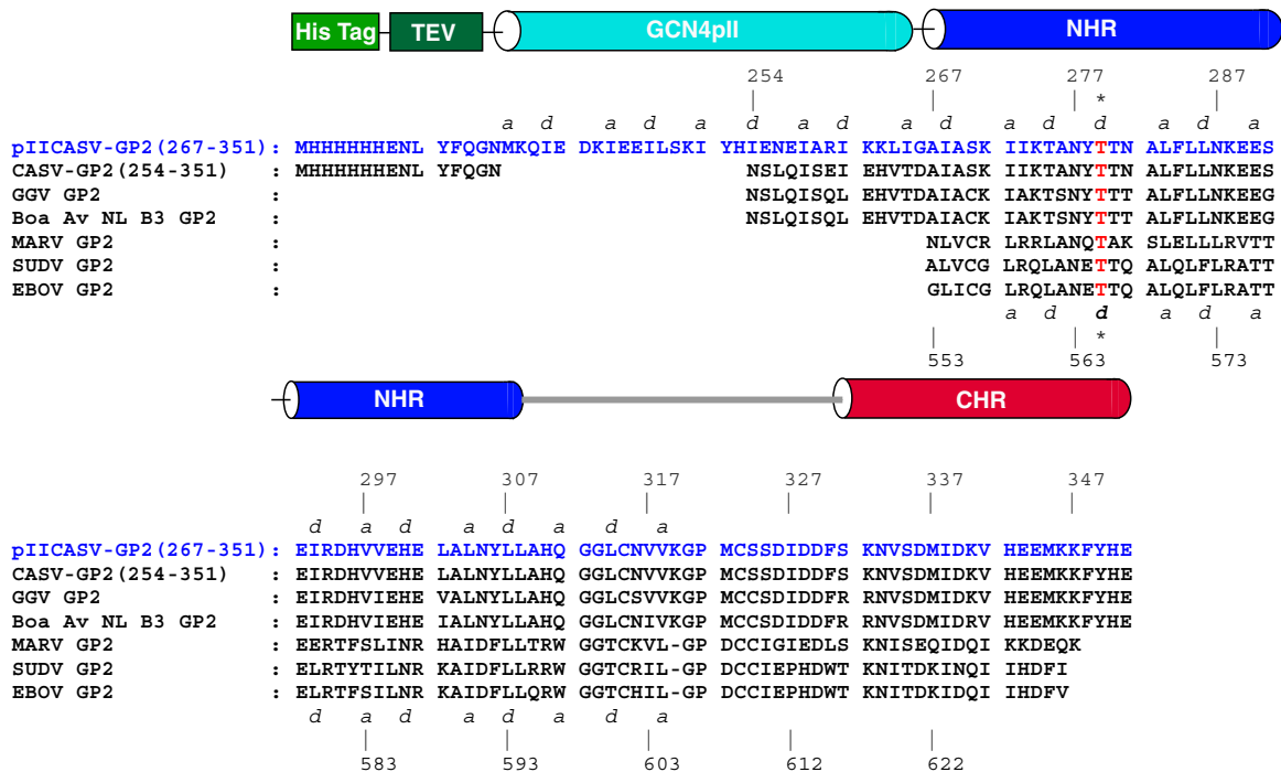
Fig. 1. CASV GP2 protein design. The sequences of the CASV GP2 constructs [pIIICASV-GP2(267–351) and CASV-GP2(254–351)] are shown in alignment to the sequences of EBOV, SUDV, MARV, GGV and BoA Av NL B3 GP2. Segments corresponding to \alpha -helical segments for the previously reported EBOV GP2 and MARV GP2 structures, as well as for the pIIICASV-GP2(267–351) structure, are represented as colored cylinders, with the colors of the cylinders matching the structural elements depicted in Fig. 5a for the pIIICASV-GP2(267–351) structure. The numbering for the EBOV GP2 residues is shown below the sequences; the numbering for the CASV GP2 residues is shown above the sequences. The a and d positions for the heptad repeat are indicated for the NHR region, with the heptad repeat stutter residue (T565 in EBOV; T279 in CASV) indicated with asterisks. The GCN4 pII segment is shown for pIIICASV-GP2(267–351) (cyan-colored cylinder).
