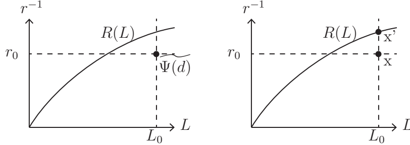
Figure 3.3: Schematic illustration of the proof involving direct limits in Theorem 1. In the region above R(L) , i.e. when r \leq R(L) , we have isomorphisms of ECH_*^L(Y_1 \#_r Y_2, \alpha_r) given a fixed value of L by Proposition 61.
