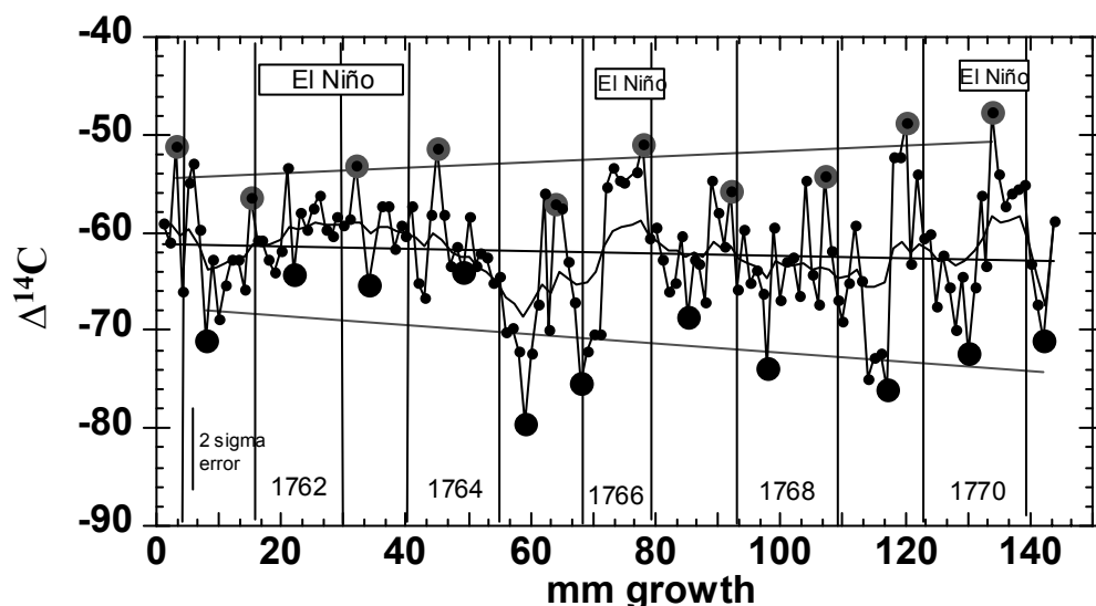
Figure 1 \Delta^{14}\text{C} measurements of monthly coral bands from Urville Bay, Galapagos, during the period 1760 to 1771. The uncertainty of the age assignments in this age range is \pm 6 yr. Duplicate analyses of separate aliquots from the same coral sample and splits of the same \text{CO}_2 were averaged to a single point. Large grey points represent the highest \Delta^{14}\text{C} values for each year (lowest upwelling) and large black points represent the lowest \Delta^{14}\text{C} values for each year (most intense upwelling). Vertical lines mark the base of the high-density bands, which are generally formed when upwelling is low. Horizontal lines (grey) are the least-squares fits of the high and low ^{14}\text{C} values, and that (black) for all of the monthly results. The smoothed line of the monthly data is obtained using a Stineman function, which suggests that El Niño events occurred during 1762–63 and possibly 1766.
