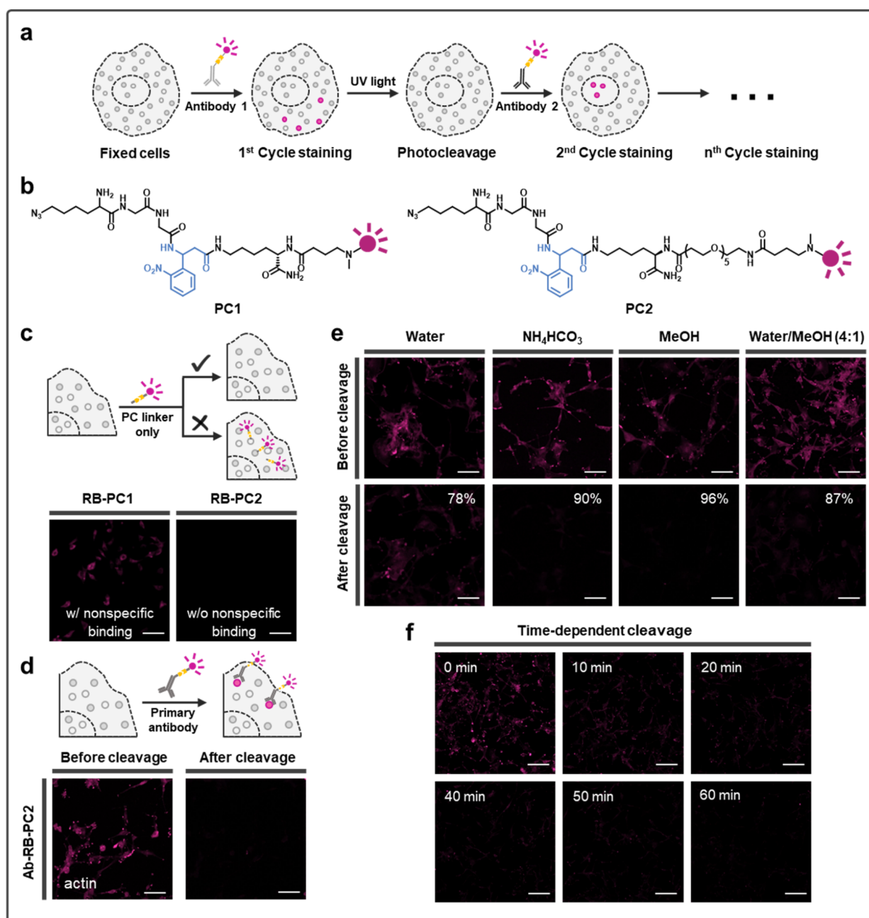
Figure 1. Design and optimization of PACIFIC. (a) Proteins in the cells can be quantified through fluorescent antibodies labeled with photocleavable (PC) linkers. After imaging, the PC linker and the fluorophore can be cleaved with UV light. This process allows iterative label-erase-label cycles of immunofluorescence. (b) Two PC linkers are designed. The azide tag allows antibody conjugation via a strain-promoted azide–alkyne cycloaddition (SPAAC) reaction, the ANP module works as the photoactive moiety, and a PEG5 segment is used in PC2 to increase the hydrophilicity. (c) Confocal images showing that RB-PC1 had a nonspecific binding with fixed cells and RB-PC2 could be easily removed. (d) Confocal images showing that the Ab-RB-PC2 was able to label the actin from U87 cells, and the signal can be erased by UV irradiation. (e) Cleavage tests of Ab-RB-PC2 in different media. (f) Time-dependent cleavage of Ab-RB-PC2 in argon-purged methanol. Scale bar, 50 \mu\text{m} .
