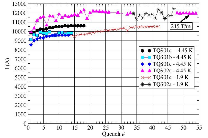
Fig.3. Training curves of the 4 test TQS magnets.
