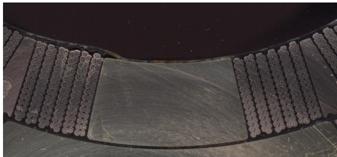
Fig.10. Visible damage to coil 15 after MITTs heater study.
