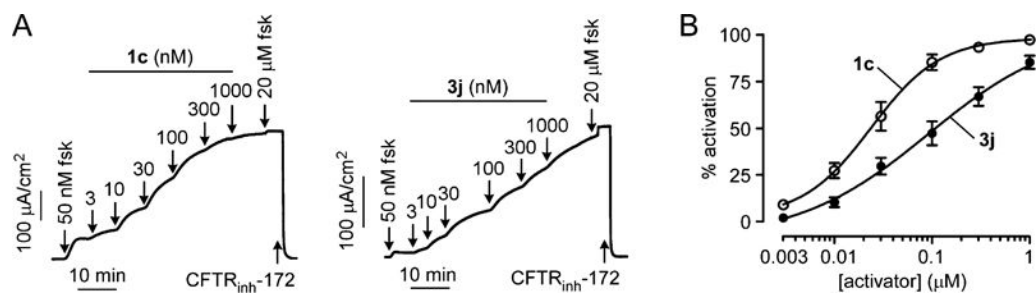
Figure 2. Short-circuit current measurement of CFTR activation by 1c and 3j . (A) Measurements done in FRT cells expressing human wild-type CFTR showing responses to indicated concentrations of forskolin, 1c , or 3j , and 10 \mu\text{M} CFTR inhibitor CFTR inh -172. (B) Concentration-dependent activation of CFTR (mean \pm SEM, n = 3 ).
