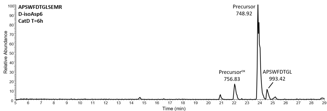
Figure 2.S18. LC-MS total ion chromatogram for peptide isomeric form listed in upper left corner.
