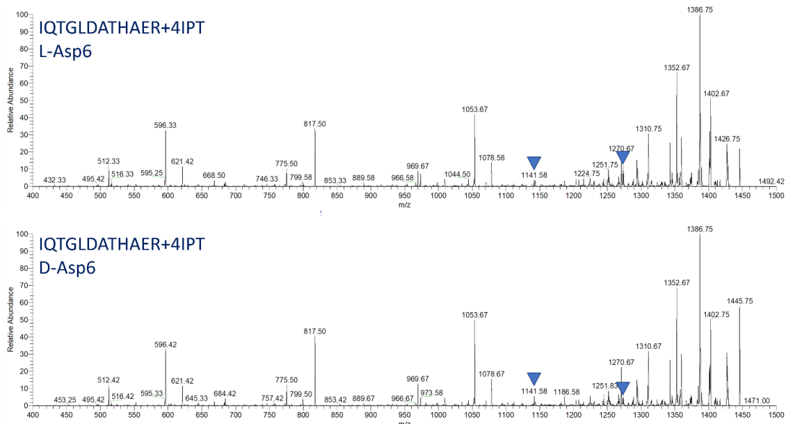
Figure 5.S7. RDD comparison of IQTGLDATHAER+4IPT L-Asp (Top) and D-Asp (Bottom). R_{\text{isomer}} = 3.30
