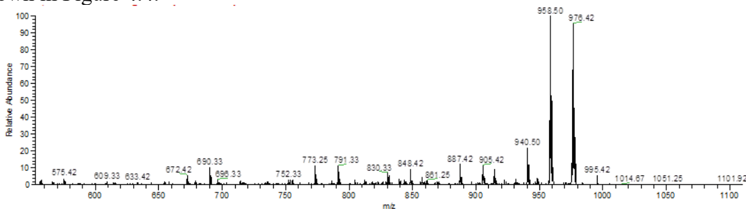
Figure 4.S9. CID fragmentation spectrum for the ligation product GPSWFDTGGK shown in Figure 4.4.
