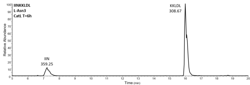
Figure 2.S37. LC-MS total ion chromatogram for peptide isomeric form listed in upper left corner.
