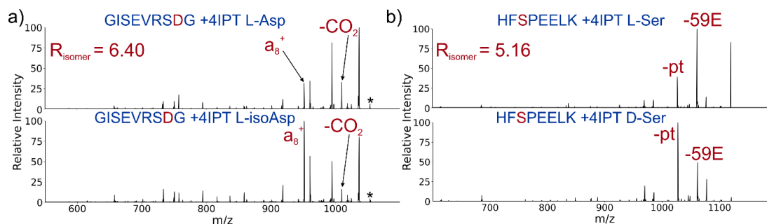
Figure 5.5. a) RDD examination of GISEVRSDG between L-Asp form (top) and L-isoAsp form (bottom). A score of 6.40 exceeds the threshold of 2.40 to confidently discriminate between isomer forms. b) RDD examination of WFDTGK epimers L-Asp (top) and D-Asp (bottom).
