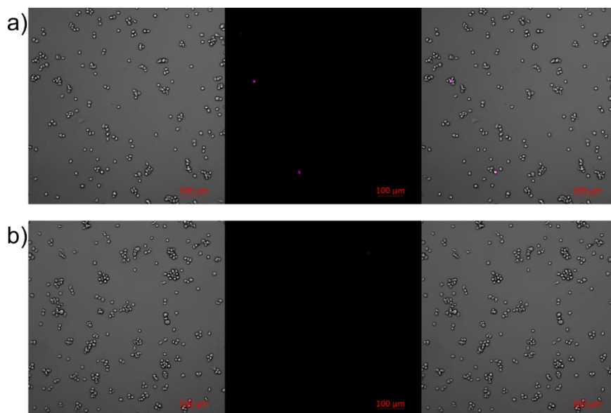
Figure 2.S2. Representative microscopy images of the brightfield, fluorescence emission, and merge (left, center, and right) depicting microglia incubated with the chimeric FRET peptide ( R_8-E_{edan}DAEFRHDK_{dab}G ) in the L-Asp form (a) and the D-isoAsp form (b).
