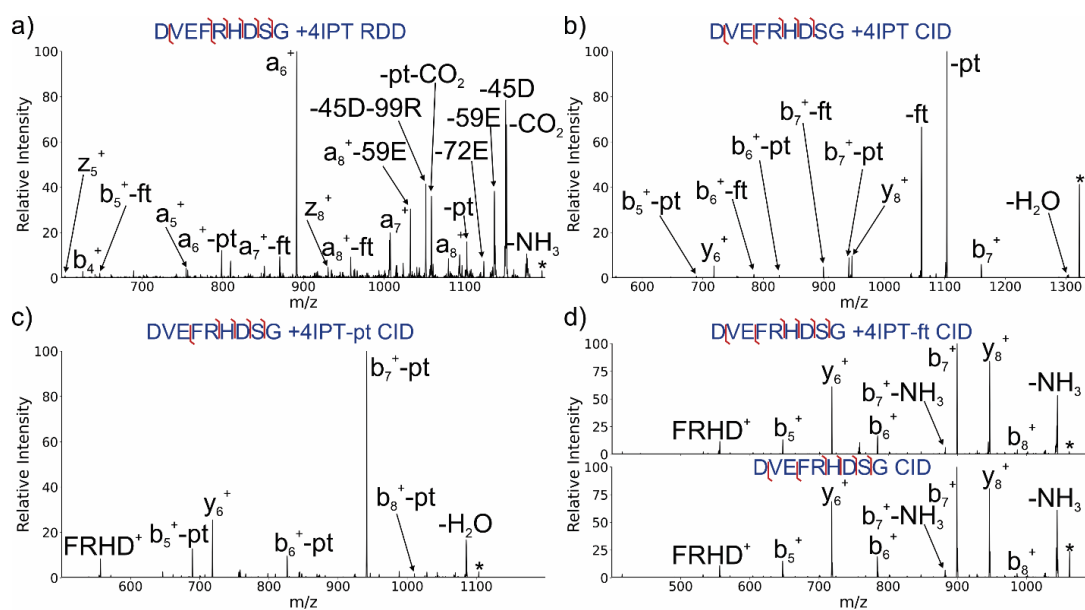
Figure 5.2. a) RDD fragmentation of DVEFRHDSG modified with 4IPT produces a-ions and side-chain losses. Unique losses of the partial tag (-pt) and full tag (-ft) and observed in some fragments. b) CID fragmentation of DVEFRHDSG modified with 4IPT produces b/y-ions and partial/full tag loss. c) CID fragmentation of the partial tag loss does not lead to full tag loss. d) CID fragmentation of the full tag loss (top) matches CID of the unmodified peptide (bottom).
