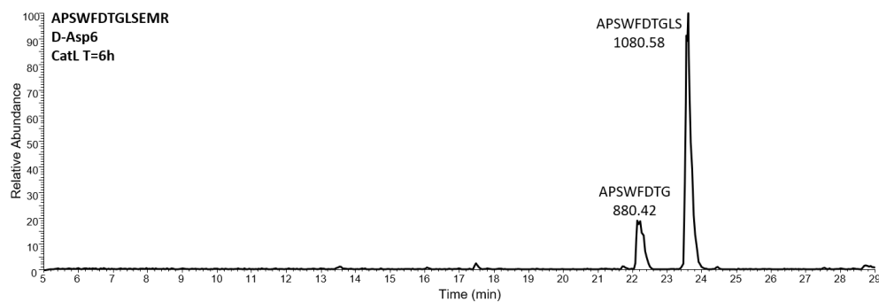
Figure 2.S33. LC-MS total ion chromatogram for peptide isomeric form listed in upper left corner.
