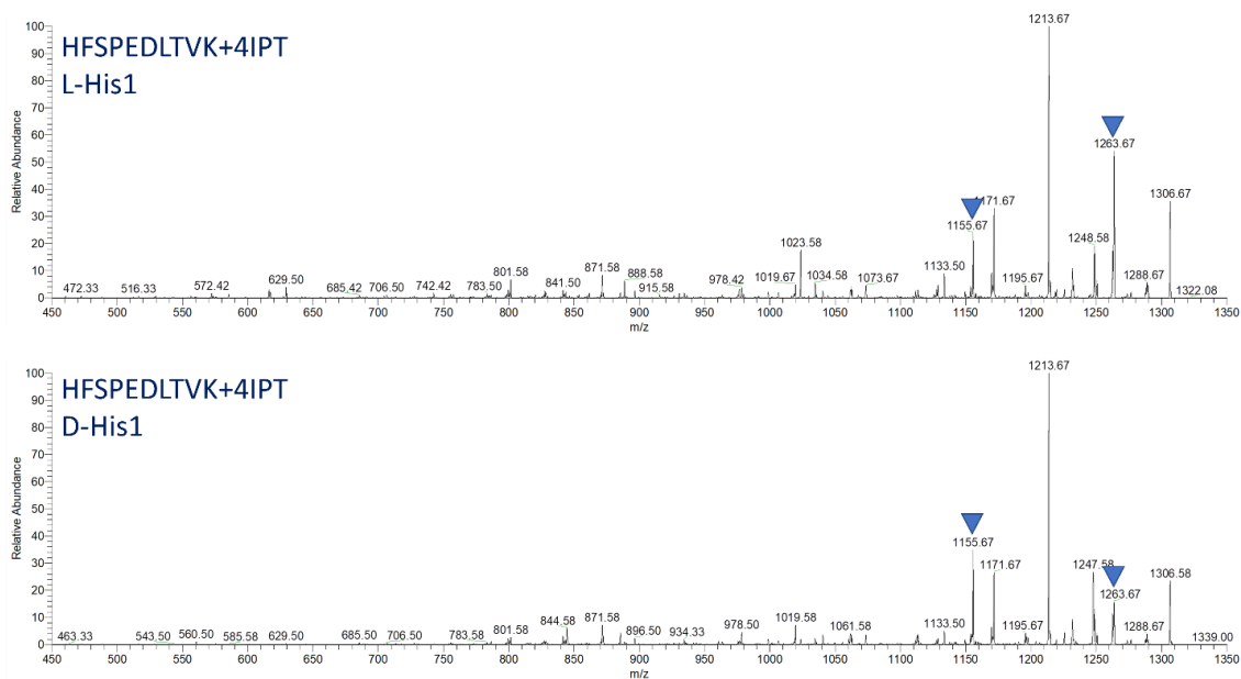
Figure 5.S8. RDD comparison of HFSPEDLTVK+4IPT L-His (Top) and D-His (Bottom). R_{\text{isomer}} = 5.16
