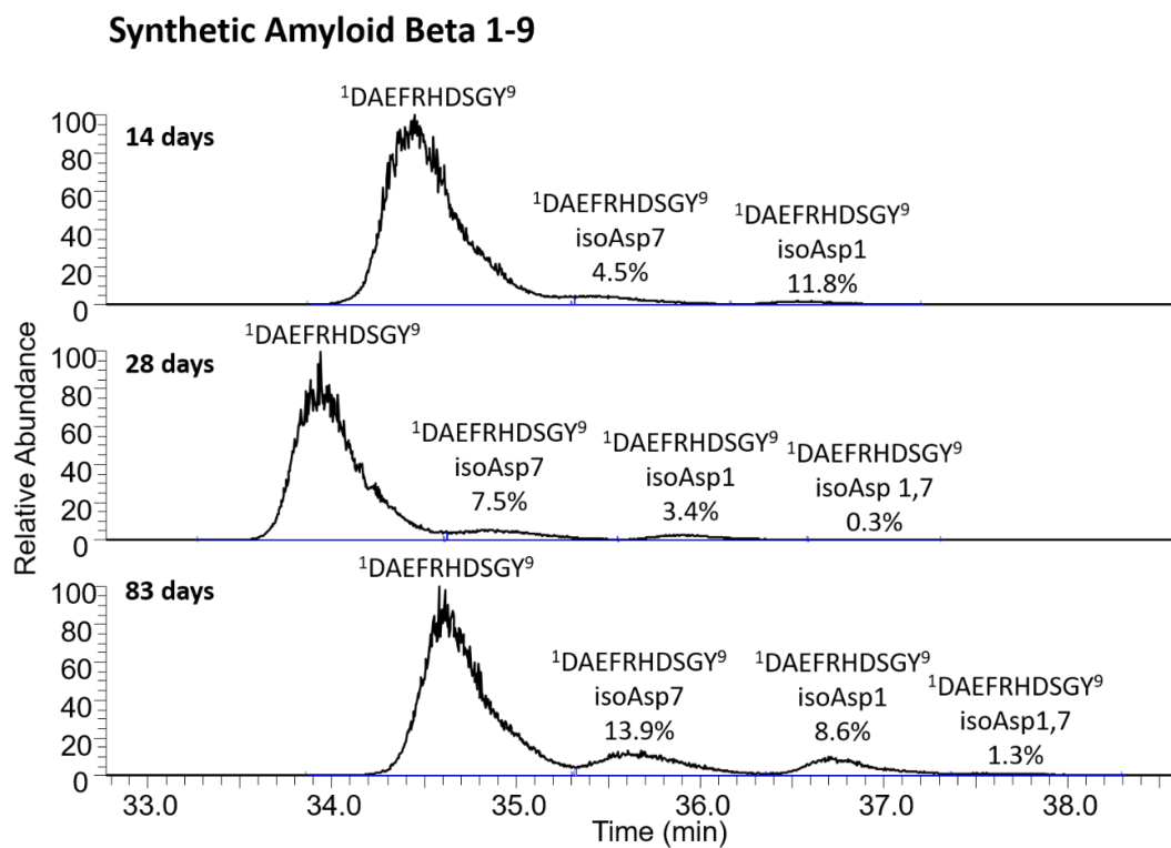
Figure 2.S4. LC-MS chromatograms corresponding to the aging data for synthetic amyloid beta 1-9 as presented in Figure 2.2.4. The isomerization rates are calculated based on LC-MS peak area.
