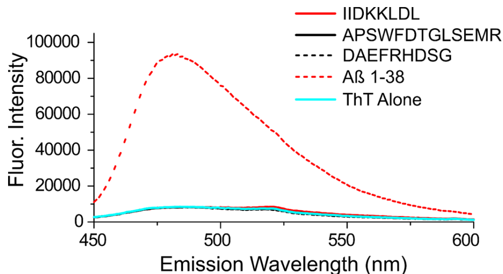
Figure 2.S10. Thioflavin-T (ThT) assay of model peptides to test for aggregation in acetate buffer after 30 minute incubation. A \beta 1-38 was used as a positive control. Lack of fluorescence for model peptides above the ThT background indicates that no aggregation is occurring prior to digestion.
