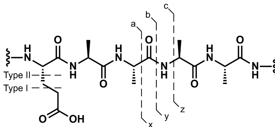
Figure 1.4. Mass spectrometry fragmentation nomenclature. a/x, b/y, and c/z ions represent backbone fragmentation while Type I/II fragments occur when part or all of a side chain is cleaved.
