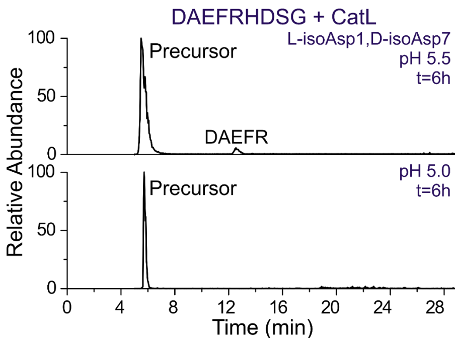
Figure 2.S11. Comparison of digestion efficiency at varying pH. Digestion of A \beta 1-9 by cathepsin L at pH 5.5 (upper trace) and pH 5.0 (lower trace). Less proteolytic cleavage is observed at the lower pH.
