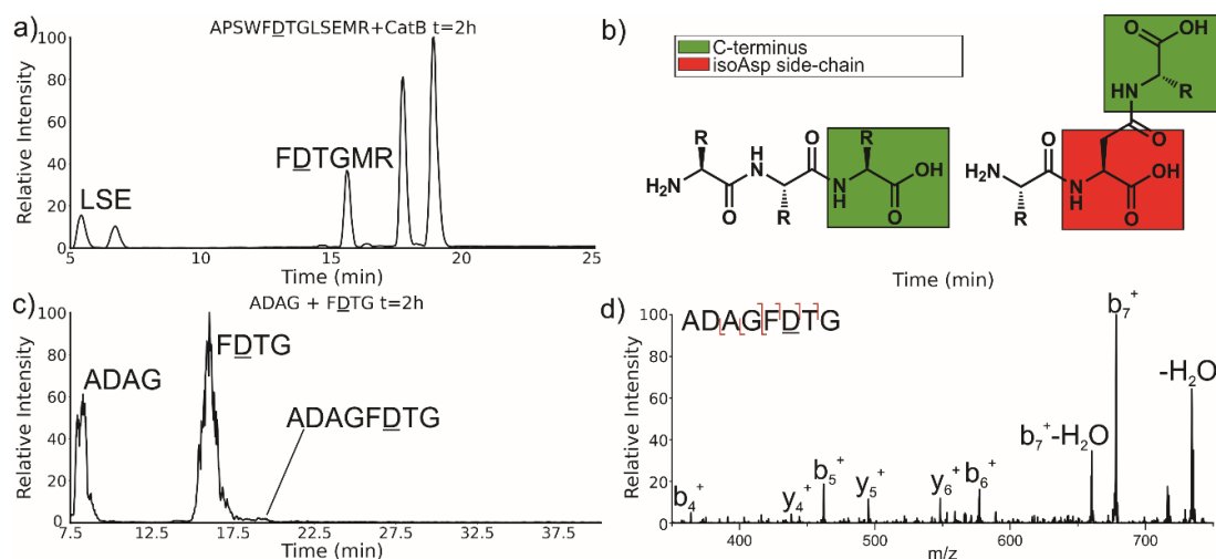
Figure 4.6. (a) LC chromatogram of the incubation of APSWF F DTGLSEMR. Incubation produces the ligated fragment F DTGMR which has been cleaved near the L-isoAsp residue due to recognition by catB. (b) Structures of a canonical peptide (left) and L-isoAsp containing peptide (right). Due to the altered connectivity of L-isoAsp, the side-chain structurally resembles a C-terminus and can be recognized by catB as a binding target. (c) LC chromatogram for the incubation of ADAG and F DTG with catB. The incubation produces the ligated fragment ADAGF(isoAsp)TG, CID fragmentation shown in (d).
