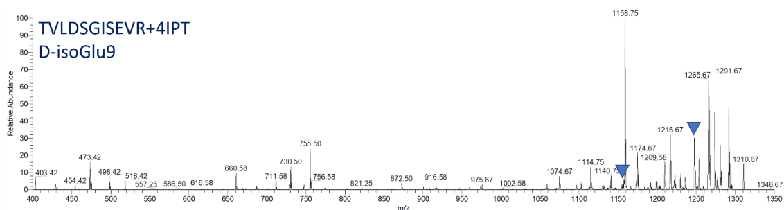
Figure 5.S6. RDD comparison of TVLDSGISEVR+4IPT L-Glu (Top) and D-isoGlu (Bottom). R_{\text{isomer}} = 5.15
