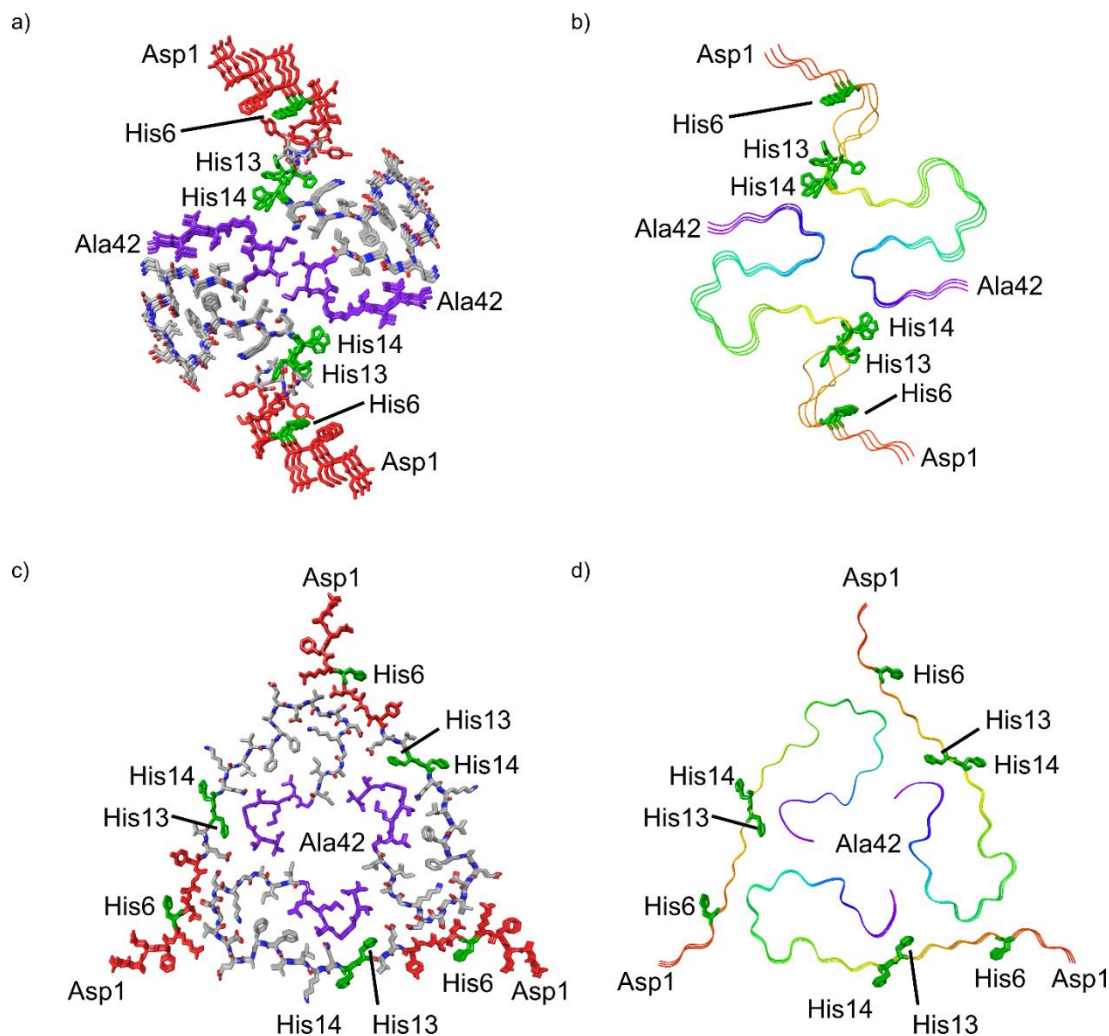
Figure 3.5. a) Tube representation and b) ribbon representation of Aβ 1-42 dimer fibril (PDB: 2NAO). The N-terminal region is shown by highlighting residues 1-10 in red and protrudes in a disordered fashion from the fibril core. The C-terminal region is shown by highlighting residues 33-40/42 in purple with exposed tail sticking out from the hydrophobic core. Relevant histidine residues are shown in green. c) Tube representation and d) ribbon representation of Aβ 1-40 trimer fibril (PDB: 2M4J). The N-terminal region is exposed with some accessibility of the following residues until the bend region.
