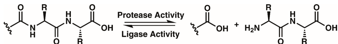
Scheme 4.1. The protease activity of CatB removes two amino acid residues as a dipeptide from the C-terminus of a substrate, while the ligase activity attaches a dipeptide to the C-terminus of a substrate.
