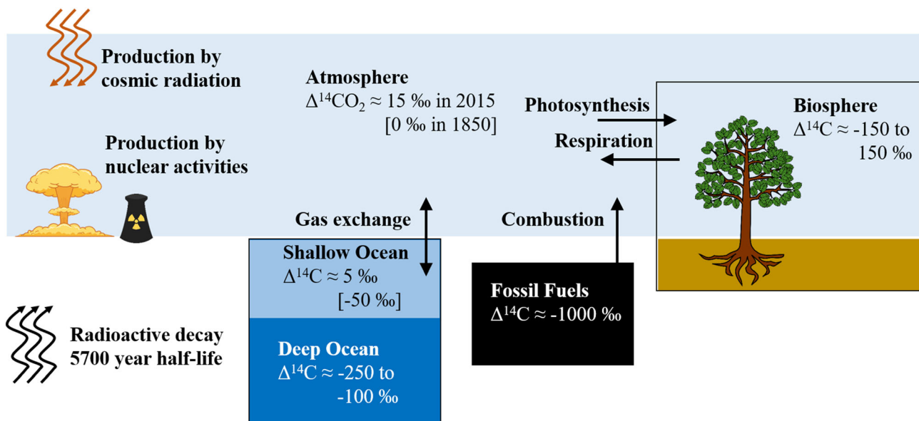
Figure 2. Diagram of ^{14}\text{C} in the global carbon cycle showing the pools interacting with atmospheric \text{CO}_2 on the timescale of the Industrial Period. Typical ranges of \Delta^{14}\text{C} are shown for each of the pools. Global average \Delta^{14}\text{C}_{\text{CO}_2} was approximately 15\text{‰} in 2015 and 0\text{‰} in 1850, whereas \Delta^{14}\text{C}_{\text{CO}_2} in the troposphere was much higher in 1964–1965, 600\text{‰} to 1,000\text{‰} (Figure 3). In the shallow ocean, average \Delta^{14}\text{C} was approximately 5\text{‰} in 2015 and -50\text{‰} in 1850. Production of ^{14}\text{C} occurs naturally through cosmic radiation and anthropogenically through nuclear activities. All ^{14}\text{C} undergoes radioactive decay with a half-life of 5,700 years.
