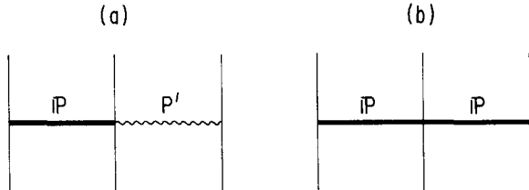
Fig. 2a) Diagram for single particle spectrum for k_{||} \sim O(s^{1/2}) in the diffractive Pomeron model. b) Diagram for pionization in the MPE model.
