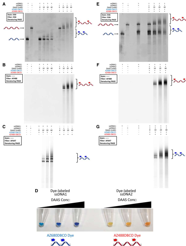
FIGURE 3. (A) Denaturing PAGE of the dye-labeled ssDNA1 and ssDNA2 samples, along with unlabeled controls. This gel was EtBr stained and imaged with an EtBr filter. (B) The same gel as in A, before EtBr staining, viewed using a laser/filter combination for Alexa Fluor 488 (used for imaging AZ488 fluorescence). (C) The same gel as in A, before EtBr staining, viewed using a laser/filter combination for Alexa Fluor 647 (used for imaging AZ680 fluorescence). (D) Picture of solutions containing the dye-labeled ssDNA1 and ssDNA2 samples in order of increasing DAAS labeling percentages. (E) Denaturing PAGE of mixtures of the dye-labeled ssDNA1 and ssDNA2 samples, along with unlabeled controls. This gel was EtBr stained and imaged with an EtBr filter. (F) The same gel as in E, before EtBr staining, imaged for AZ488 fluorescence. (G) The same gel as in E, before EtBr staining, imaged for AZ680 fluorescence. Note for (E–G): All ssDNA1/ssDNA2 combination lanes were made from previously dye-labeled samples that were mixed immediately before gel loading—no labeling was done on ssDNA1/ssDNA2 mixtures.
