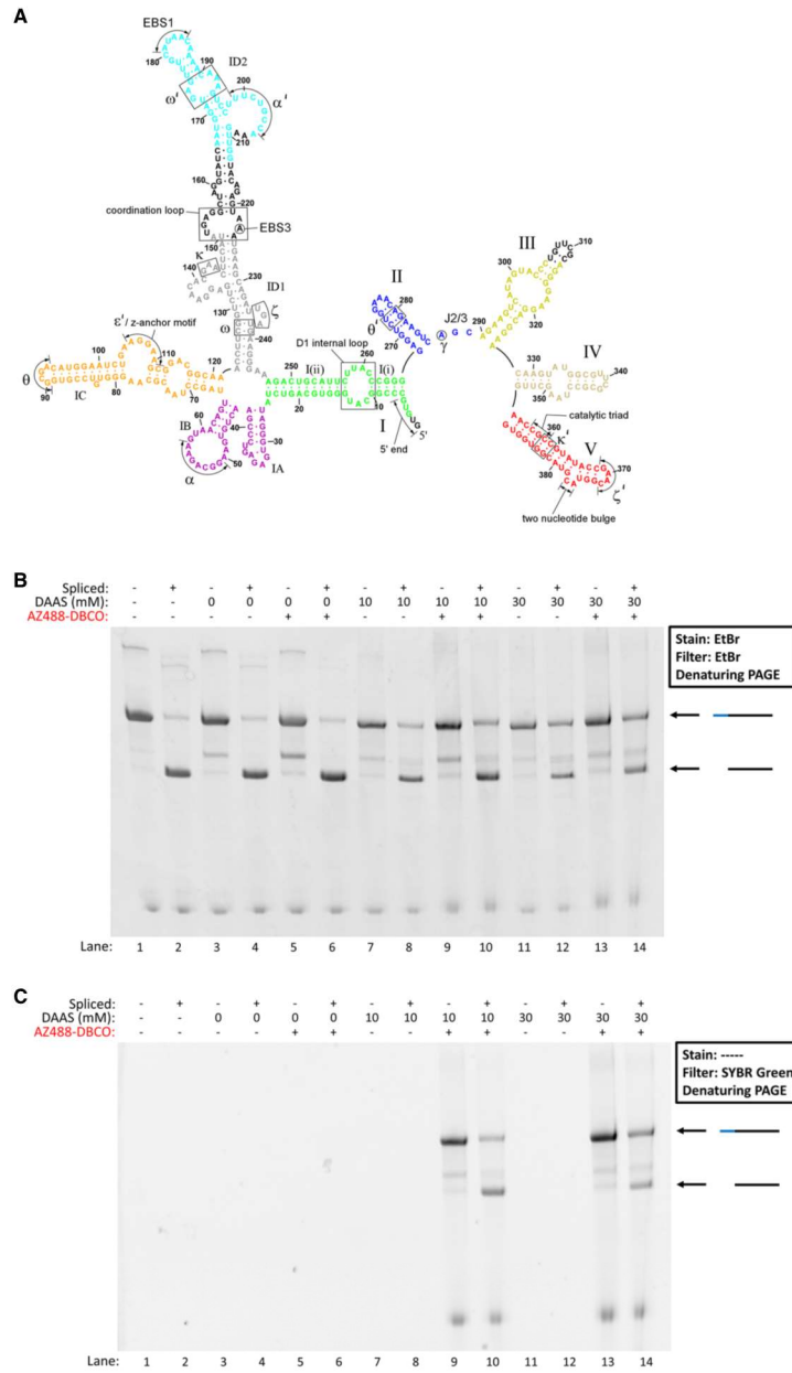
FIGURE 6. (A) Oceanobacillus iheyensis secondary structure map. (B) Denaturing PAGE showing before and after splicing time points (10 min splicing time) for a variety of O. i. samples labeled at different levels, with either DAAS by itself or with DAAS followed by AZ488-DBCO, along with unlabeled controls. Full-length (intron+ 5'-exon) and spliced bands are indicated to the right of the gel image. (C) The same gel as in B, before EtBr staining, imaged for AZ488 fluorescence.
