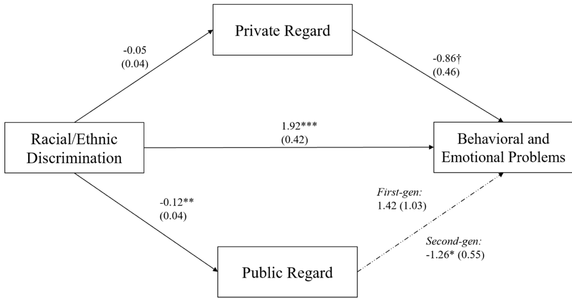
Figure 1. Final multigroup path model. Coefficients represent unstandardized regression weights and the numbers in parentheses represent standard deviations. All paths were constrained to be equal across groups except the path delineated with a dotted arrow, which was significant for second-generation Vietnamese American youth only. The model also controlled for age, gender, average parent occupational status, and number of family members in the household. Control variables and correlation between error terms for private and public regard not pictured for clarity. † p < .10 , * p < .05 , ** p < .01 , *** p < .001
