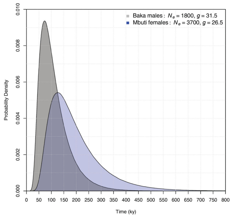
Fig. 3. Similarity of T_{\text{MRCA}} does not imply equivalent N_e of males and females
