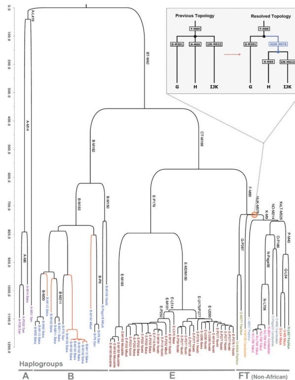
Fig. 2. Y chromosome phylogeny inferred from genomic sequencing
