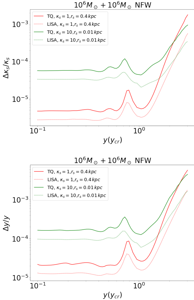
FIG. 8. The precisions of \kappa_s and y of different \kappa_s with the variation of y
