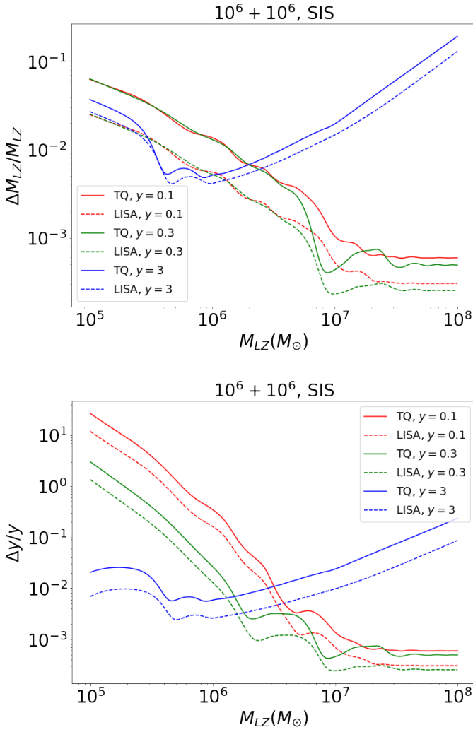
FIG. 6. The precisions of M_{Lz} and y of different y with the variation of M_{Lz}
