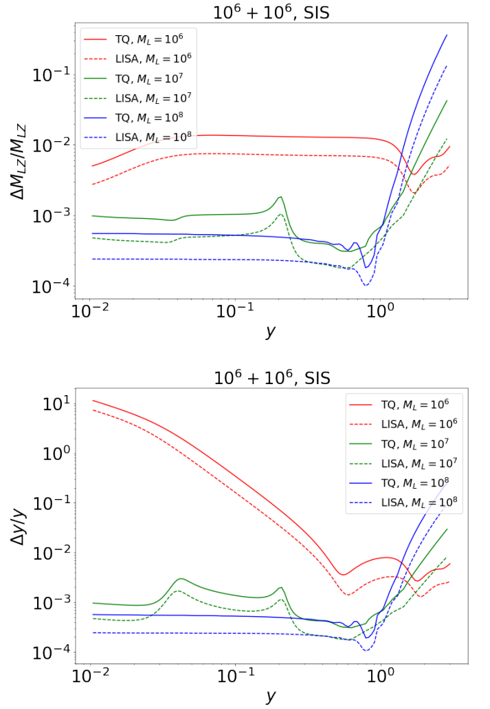
FIG. 7. The precisions of M_{Lz} and y of different M_{Lz} with the variation of y
