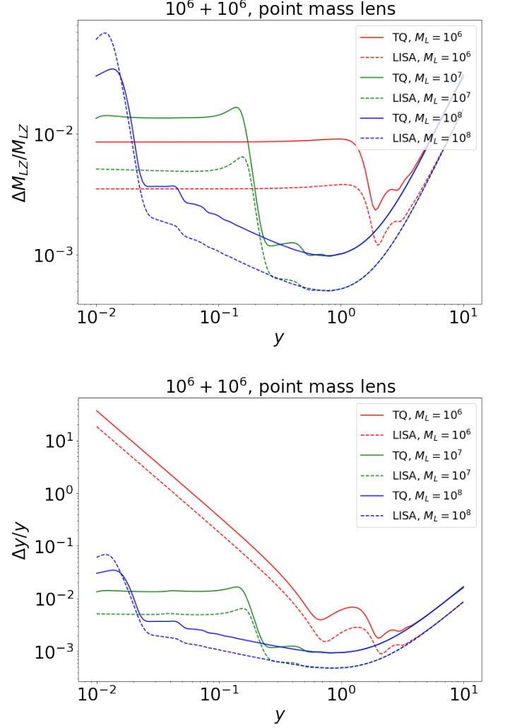
FIG. 5. The precisions of M_{Lz} and y of different M_{Lz} with the variation of y
