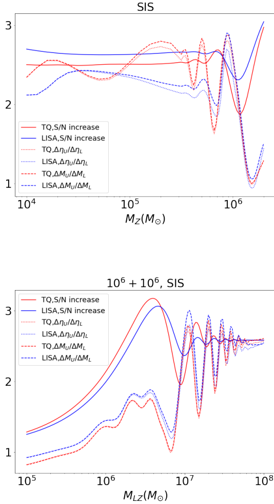
FIG. 2. The SNR and precisions increase of \eta and M_z with the variation of M_{Lz} and M_z with SIS lens
