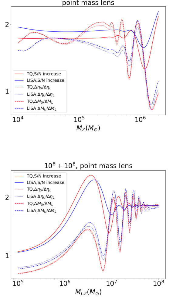
FIG. 1. The SNR and precisions increase of \eta and M_z with the variation of M_{Lz} and M_z with point mass lens.
