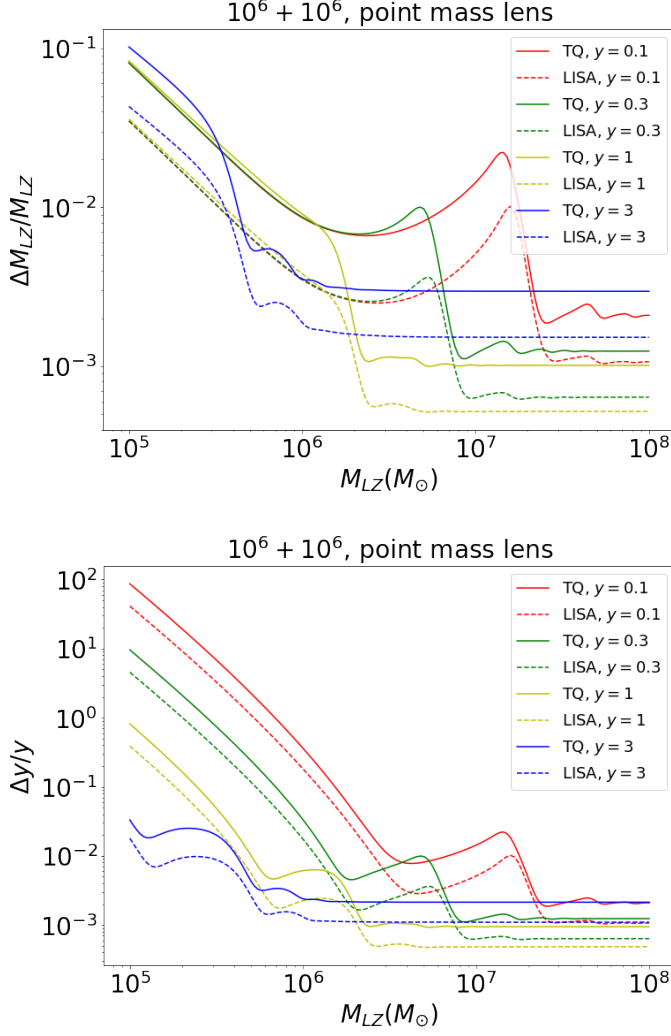
FIG. 4. The precisions of M_{Lz} and y of different y with the variation of M_{Lz}
