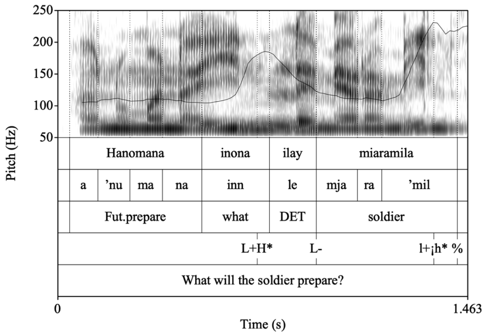
Figure 6: f0 track for Hanomana inona ilay miaramila? ‘What will the soldier prepare?’ showing that the realization of the pitch accent peak on the final syllable of a syntactic constituent delays the ip-final L- boundary tone to the following syllable
