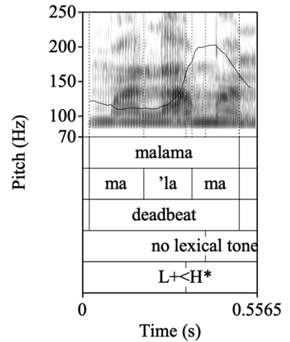
Figure 9: L+<H* preceding a syllable without lexical tone
