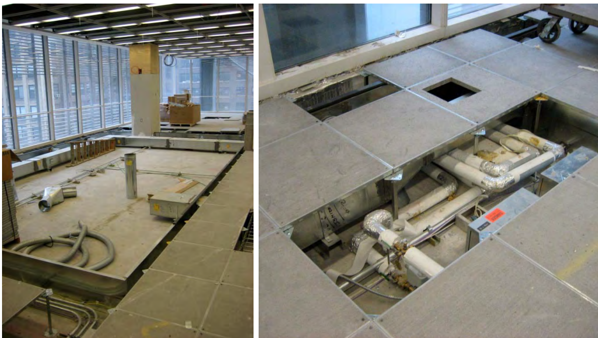
Figure 18. Images of the initial construction of the underfloor air distribution system. Copyright: LBNL.
