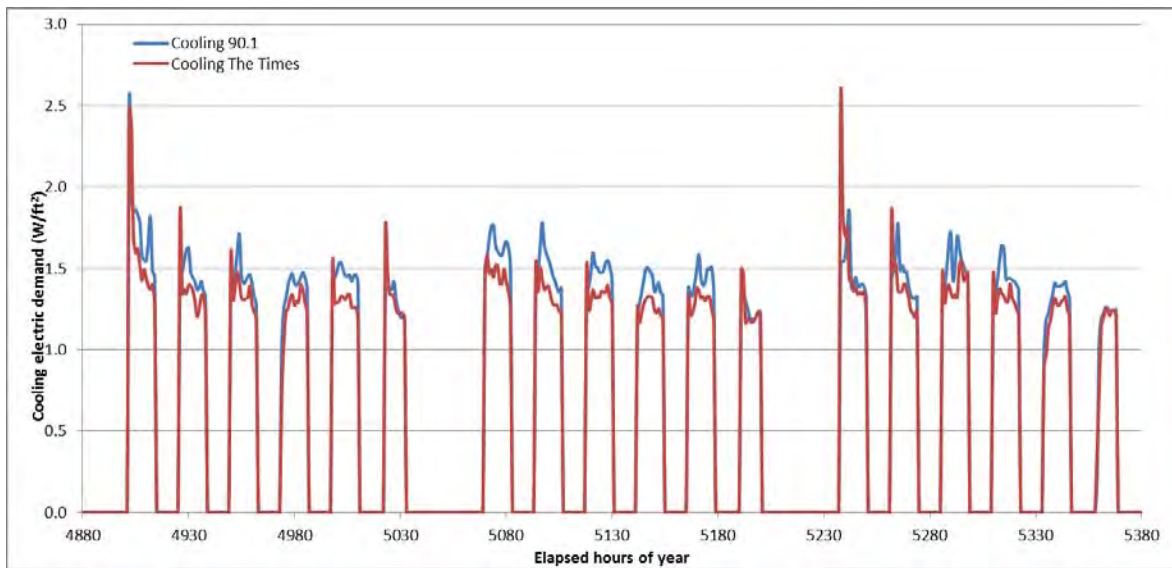
Figure 26. Peak cooling demand over the summer period from July 24 to August 12, 2011 for the ASHRAE 90.1-2001 and the Times Building model of the 20 th floor. Data produced using the calibrated EnergyPlus models.
