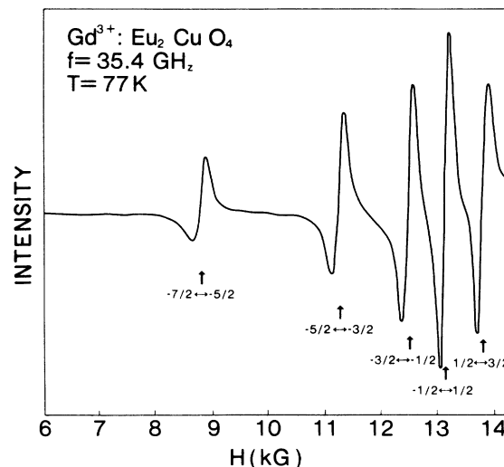
FIG. 2. ESR spectrum of \text{Eu}_2\text{CuO}_4 doped with 1.5 at.% Gd, taken at 35 GHz with the magnetic field parallel to the c axis. Notice that at this frequency we do observe the low-field -\frac{7}{2} \leftrightarrow -\frac{5}{2} fine-structure line.
