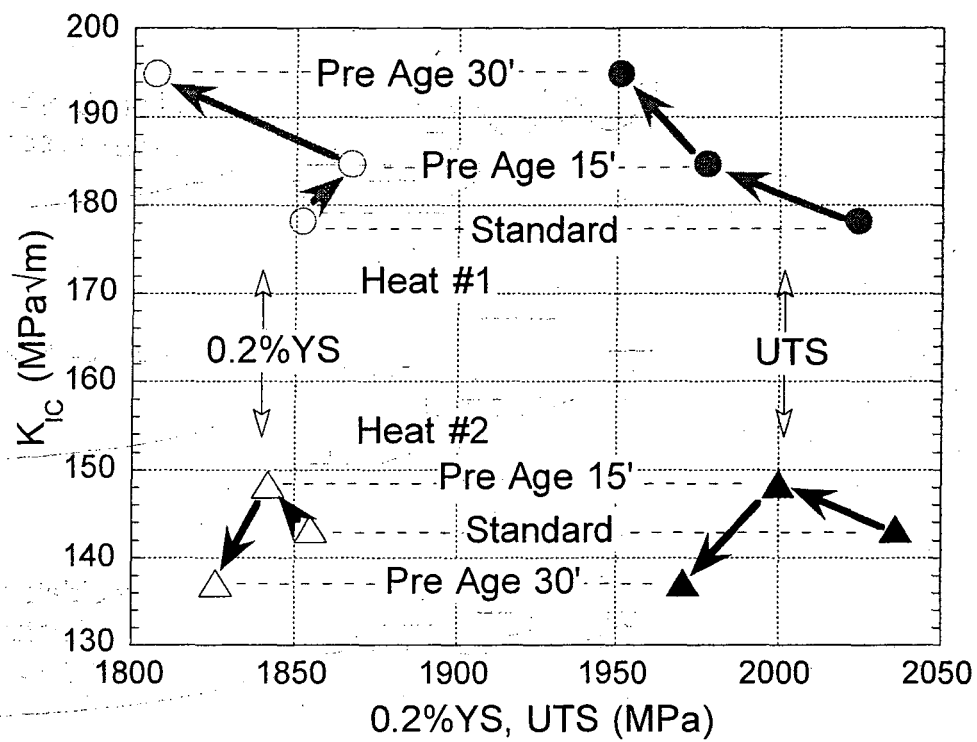
Figure 4.23 Effect of pre-aging conditions on the toughness-strength relationship.
