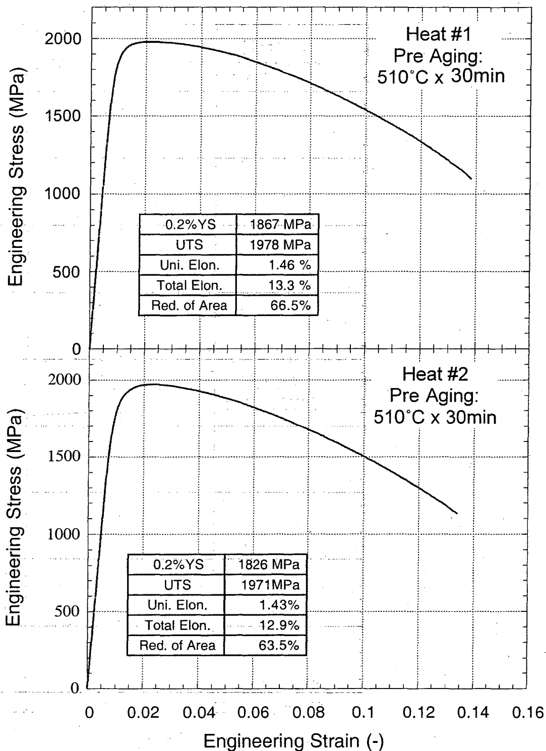
Figure A6 Effect of pre-aging on the engineering stress – engineering strain curve. Heat treatment: (A) 885°C x 1hr, OQ +(DF)-197°C x 1h + (PreAg) 510°C x 30min, OQ +(DF)-197°C x 1h + (Ag) 482°C x 5h, OQ
