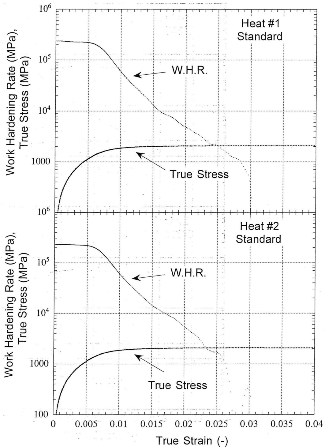
Figure 4.6 Work hardening rate – true strain curve.
