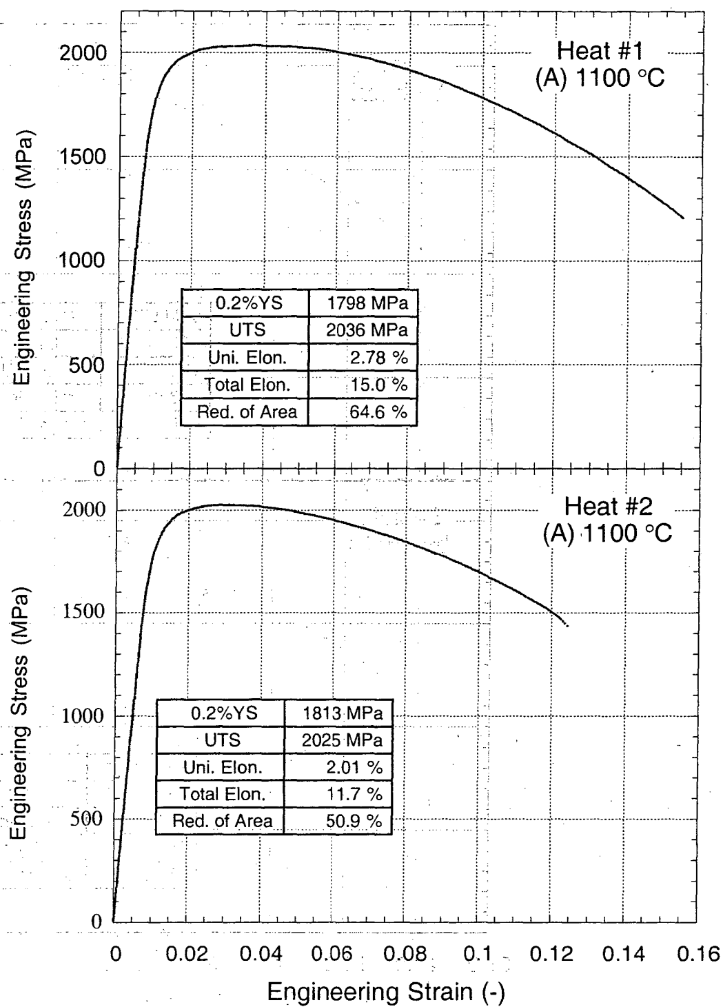
Figure A1 Effect of high temperature austenitization on the engineering stress – engineering strain curve Heat treatment: (A) 1100 °C x 1hr, OQ + (DF)-197 °C x 1h + (Ag) 482 °C x 5h, OQ
