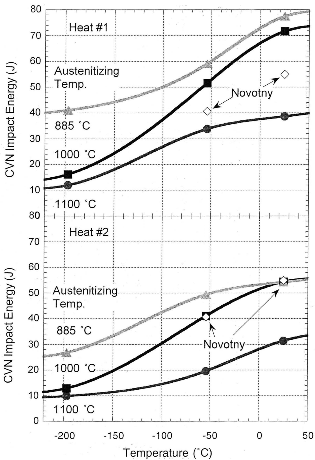
Figure 3.3 Effect of austenitizing temperature on the temperature dependence of the CVN impact energy.
