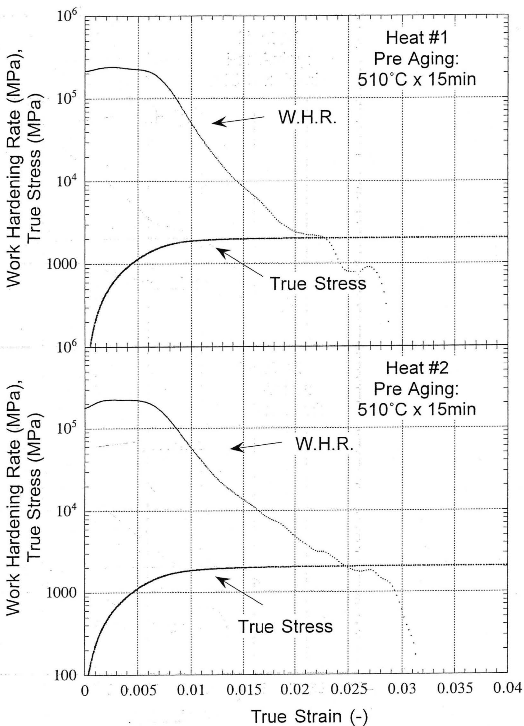
Figure 4.9 Effect of pre-aging on the work hardening rate – true strain curve. Heat treatment: (A) 885°C x 1h, OQ + (DF)-197°C x 1h + (PreAg) 510°C x 15min, OQ + (DF)-197°C x 1h + (Ag) 482°C x 5h, OQ
