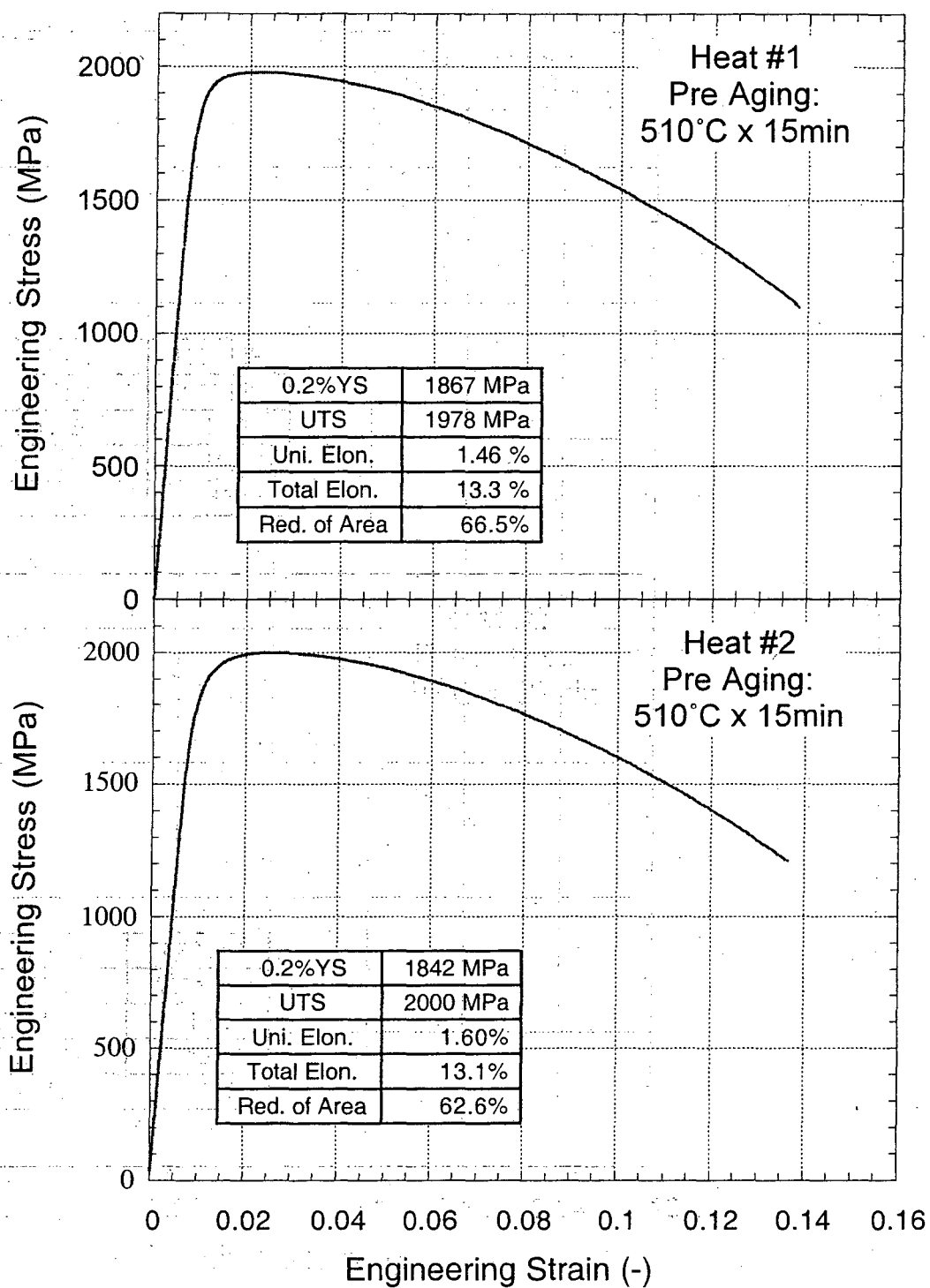
Figure A5 Effect of pre-aging on the engineering stress – engineering strain curve Heat treatment: (A) 885°C x 1hr, OQ +(DF)-197°C x 1h + (PreAg) 510°C x 15min, OQ + (DF)-197°C x 1h + (Ag) 482°C x 5h, OQ
