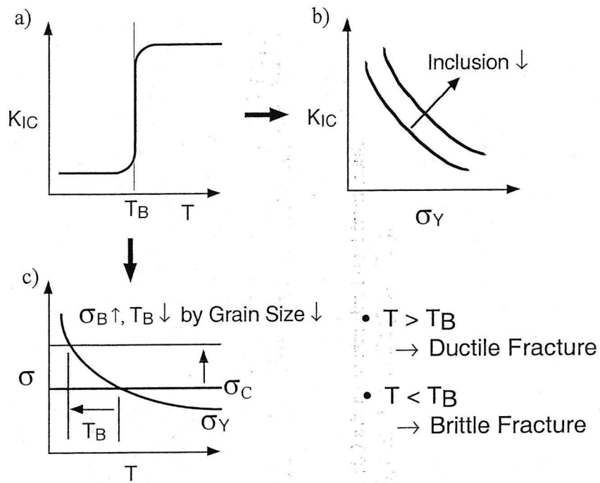
Figure 1.3 Fracture behavior of ferritic steels.
