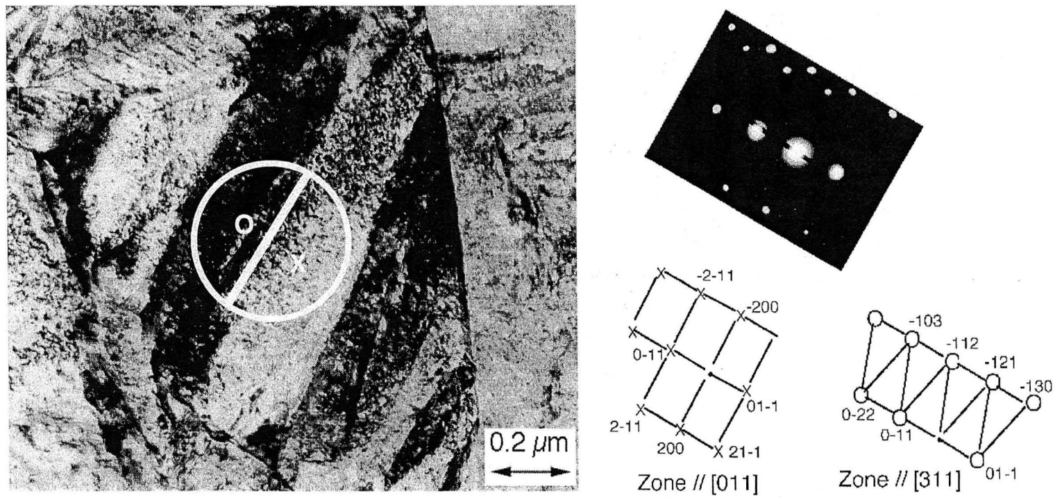
Figure 2.3 TEM bright field image and the SAD pattern of AerMet 100. Region marked "O" in the selected area in the TEM image has zone parallel to [311] , and "X" has [011]
