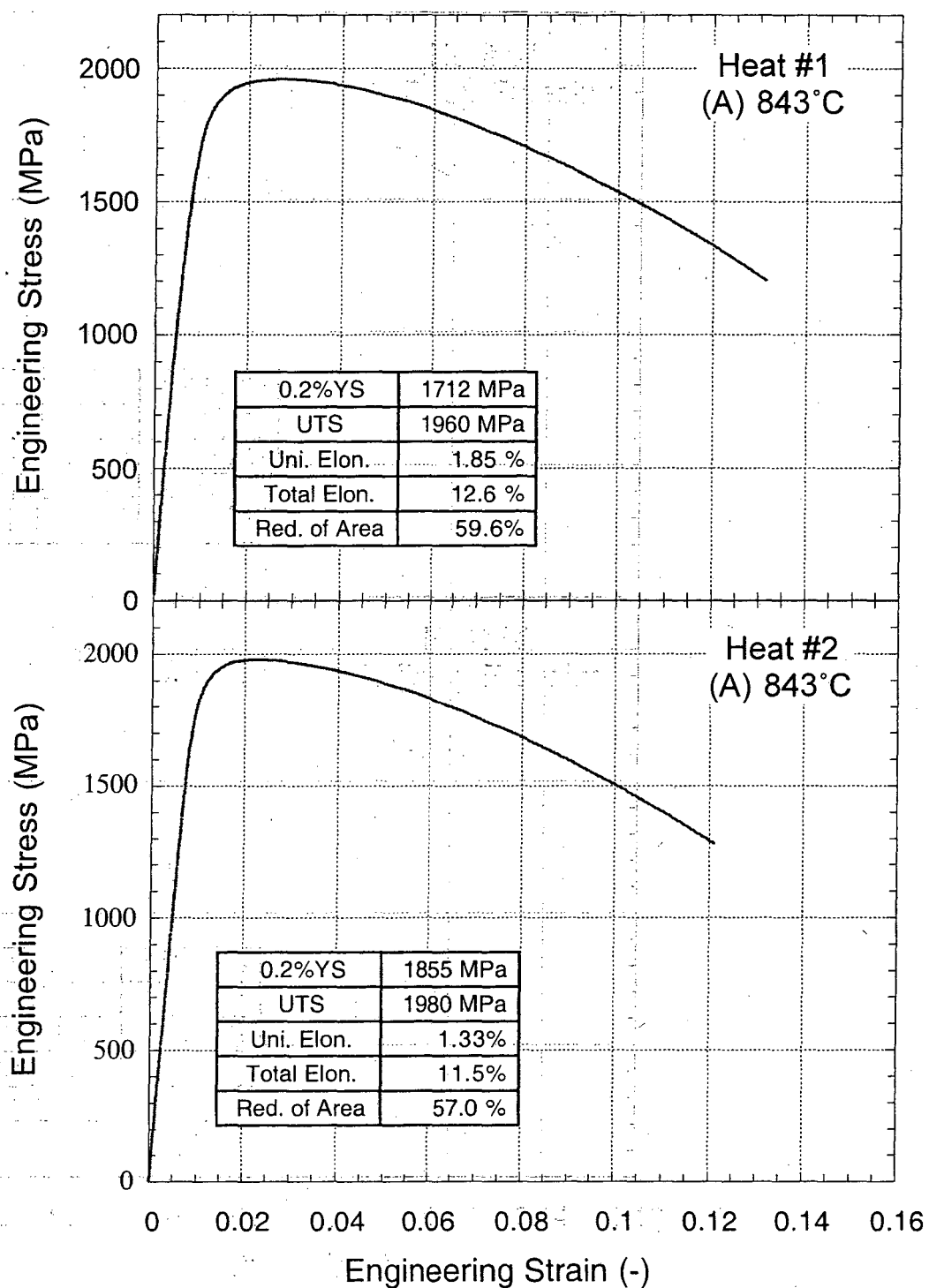
Figure A3. Effect of low temperature austenitization on the engineering stress – engineering strain curve.
