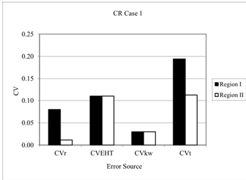
Figure 5. Error term contributions for the CRM for Coso West Sugarloaf (WSL) obsidian at 20°C, showing the improvement due to the method. The current uncertainty in EHT ( \sigma_{\text{EHT}} = 1.0^\circ\text{C} ) is assumed. The calibration process has greatly reduced the effects of intra-source water variation; accuracy in Region I is again limited by rim measurement ( \text{CV}_r ), and in Region II by EHT ( \text{CV}_{\text{EHT}} ).
