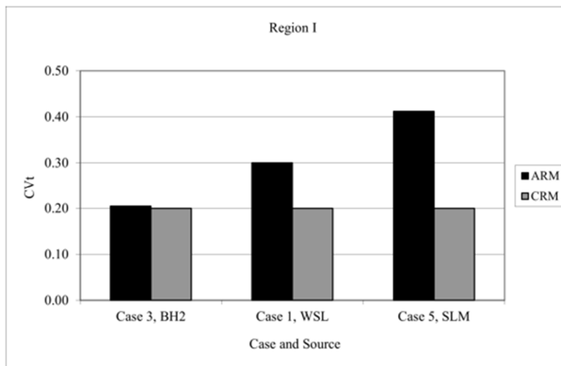
Figure 6. Comparison of age CV for the ARM and CRM in Region I for three typical obsidians, showing the improvement due to the CRM. Bodie Hills Group 2 (BH2) is a dry obsidian which hydrates slowly, Coso West Sugarloaf (WSL) is a moderately wet obsidian, and Coso Sugarloaf Mountain (SLM) is a wet, fast-hydrating obsidian.
