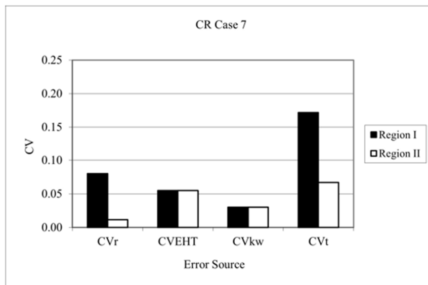
Figure 9. Error term contributions for the CRM for both Coso West Sugarloaf (WSL) and Bodie Hills Group 2 (BH2) obsidian at 20°C, with the uncertainty in EHT reduced to \sigma_{\text{EHT}} = 0.5^\circ\text{C} . In Region II the error sources are well balanced, with a total \text{CV}_t \approx 7\% . In Region I the accuracy is limited by rim measurement ( \text{CV}_r ).
