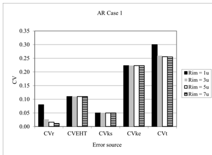
Figure 4. Error term contributions for the ARM for Coso West Sugarloaf (WSL) obsidian at 20°C. Rim values < 4μ fall within Region I. Note the accuracy is worse in Region I due to rim measurement error (CV r ), and improves with increasing rim value; also note the large error contribution from intra-source variations in intrinsic water (CV ke ).
