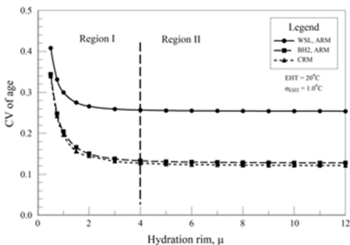
Figure 2. Age coefficient of variation as a function of hydration rim. Three cases are shown: a relatively fast obsidian (Coso West Sugarloaf) and a slow obsidian (Bodie Hills Group 2), computed by the ARM; and age CV computed by CRM. Age accuracy is better in Region II than in Region I because the error contribution due to hydration rim measurement becomes negligible for rims > 4 \mu .
