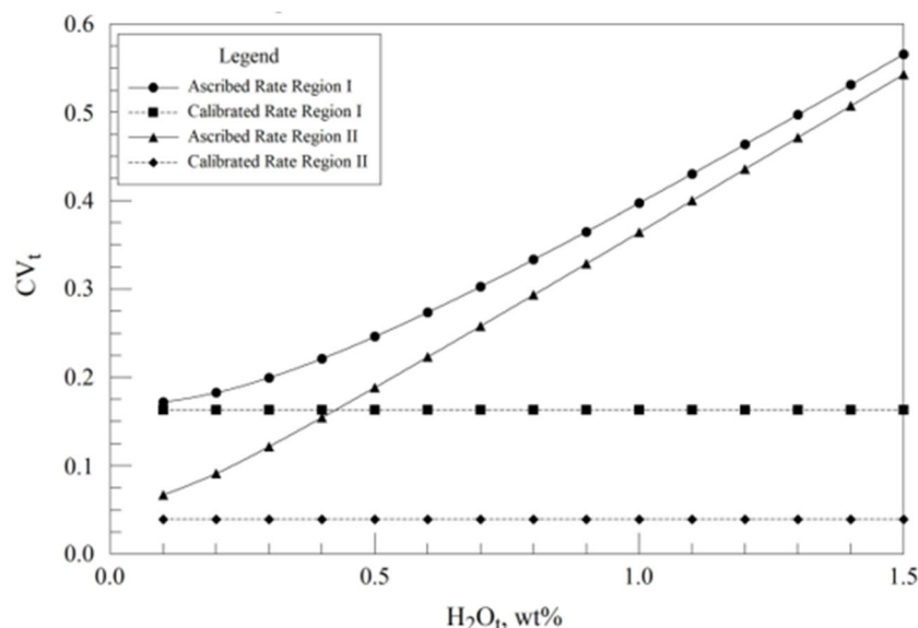
Figure 8. Age CV for ARM and CRM, as a function of total water content. Note that use of the CRM leads to improved accuracy, but the accuracy in Region I is always worse than in Region II.
