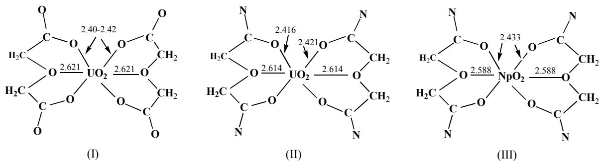
Figure 6. Solid structures of actinyl complexes. (I) [\text{C}_2\text{H}_5\text{NH}_2(\text{CH}_2)_2\text{NH}_2\text{C}_2\text{H}_5][\text{UO}_2(\text{ODA})_2](\text{cr}) [4]. (II) \text{UO}_2(\text{TMOGA})_2(\text{ClO}_4)_2(\text{cr}) [12], (III) \text{NpO}_2(\text{TMOGA})_2\text{ClO}_4(\text{cr}) [11]. The cation in (I) and the anion in (II) and (III) are not shown for clarity.
