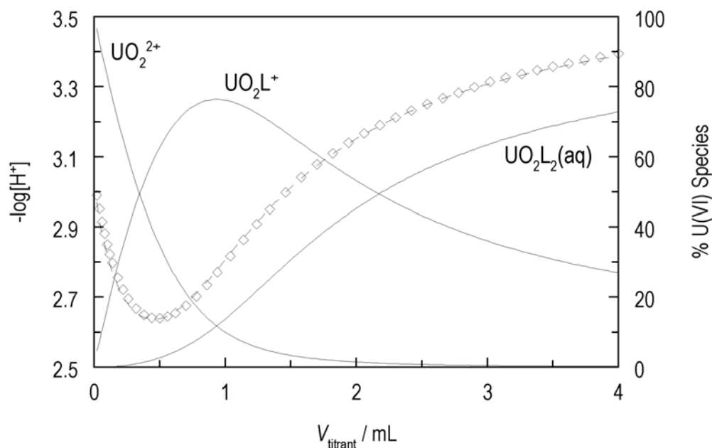
Figure 3. A representative potentiometric titration of the U(VI)-DMOGA system, I = 1.0 \text{ mol}\cdot\text{dm}^{-3} \text{ NaClO}_4 , t = 25^\circ\text{C} . Initial cup solution (20.0 ml): C_{\text{H}} = 0.950 \text{ mmol}\cdot\text{dm}^{-3} , C_{\text{U}} = 8.85 \text{ mmol}\cdot\text{dm}^{-3} . Titrant: C_{\text{H}} = 0.148 \text{ mol}\cdot\text{dm}^{-3} , C_{\text{DMOGA}} = 0.346 \text{ mol}\cdot\text{dm}^{-3} . Symbols: \diamond - experimental data ( -\log[\text{H}^+] ); dashed line – fit ( -\log[\text{H}^+] ); solid lines - percentage of U(VI) species (right y-axis), L stands for the deprotonated DMOGA ligand.
