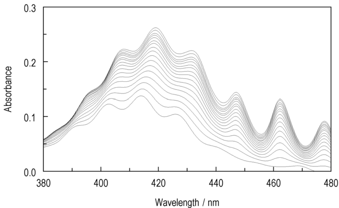
Figure 2. Spectrophotometric titration of the U(VI)-DMOGA system, I = 1.0 \text{ mol}\cdot\text{dm}^{-3} \text{ NaClO}_4 , t = 25^\circ\text{C} . Initial cuvette solution (2.50 ml): C_{\text{H}} = 0.0212 \text{ mol}\cdot\text{dm}^{-3} , C_{\text{U}} = 0.0177 \text{ mol}\cdot\text{dm}^{-3} . Titrant: C_{\text{H}} = 0.01915 \text{ mol}\cdot\text{dm}^{-3} , C_{\text{DMOGA}} = 0.2192 \text{ mol}\cdot\text{dm}^{-3} . The spectra have been normalized to account for dilution due to volume increase along the titration.
