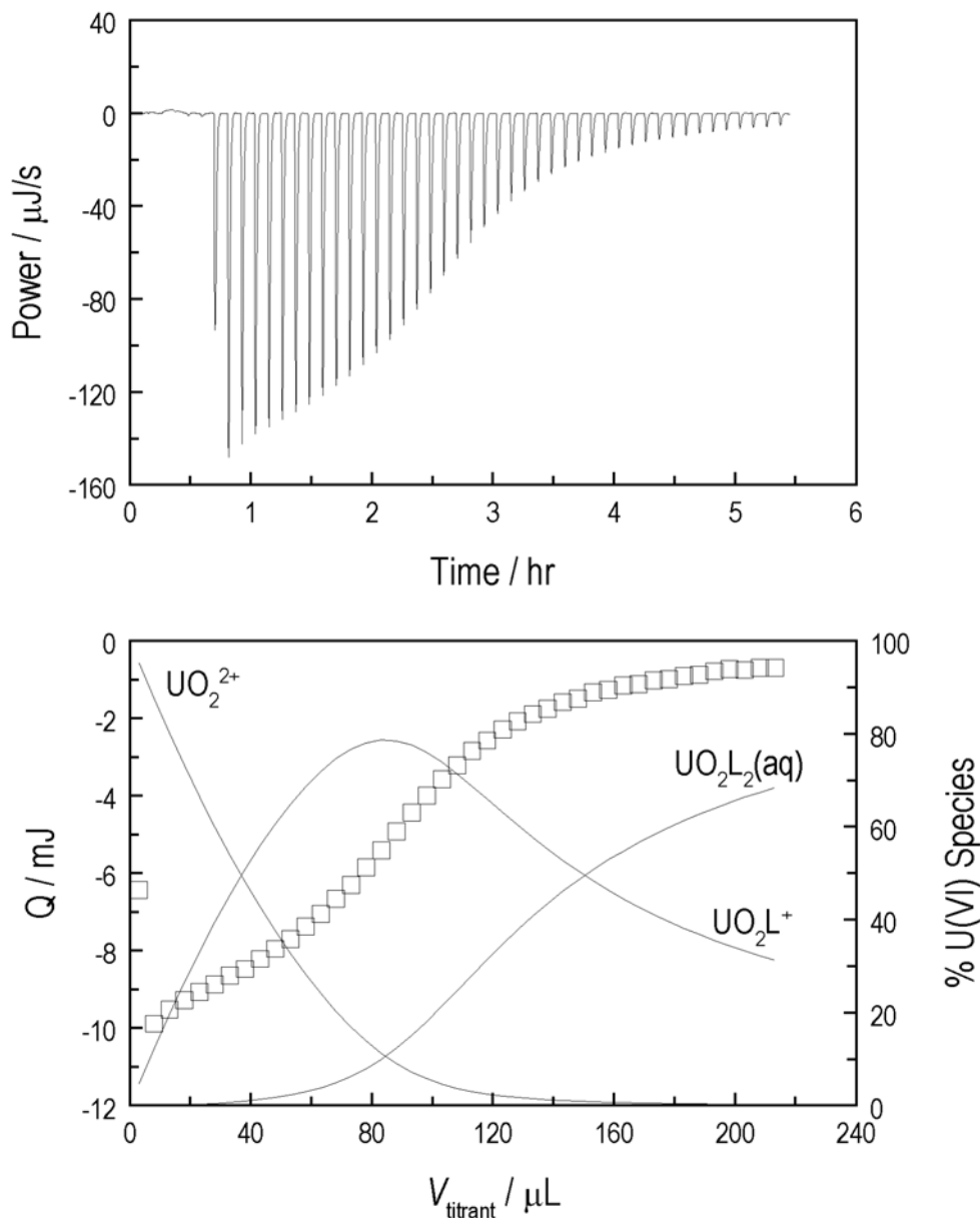
Figure 4. Calorimetric titration of the U(VI)-DMOGA system. , I = 1.0 \text{ mol}\cdot\text{dm}^{-3} \text{ NaClO}_4 , t = 25^\circ\text{C} . Initial cup solution (0.900 ml): C_{\text{H}} = 11.78 \text{ mmol}\cdot\text{dm}^{-3} , C_{\text{U}} = 9.833 \text{ mmol}\cdot\text{dm}^{-3} . Titrant: C_{\text{H}} = 0.0109 \text{ mol}\cdot\text{dm}^{-3} , C_{\text{DMOGA}} = 0.2282 \text{ mol}\cdot\text{dm}^{-3} . (Top) Thermogram; (bottom) Stepwise heat ( \square , left y-axis) and speciation of U(VI) (lines, right y-axis) vs. the volume of titrant.
