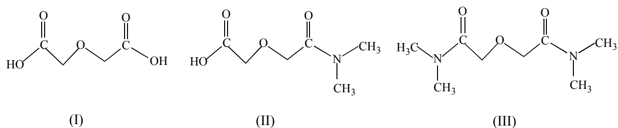
Figure 1. (I) Oxydiacetic acid (ODA); (II) dimethyl-3-oxa-glutaramic acid (DMOGA); (III) tetramethyl-3-oxa-glutaramide (TMOGA).
